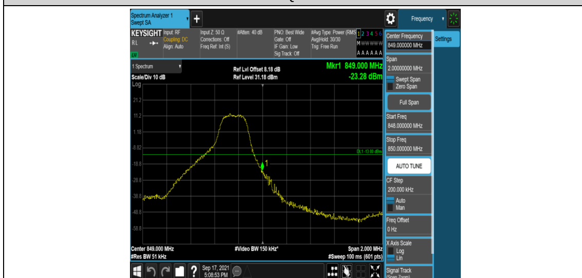
Band5-3MHz-16QAM-20635-1RB#14
