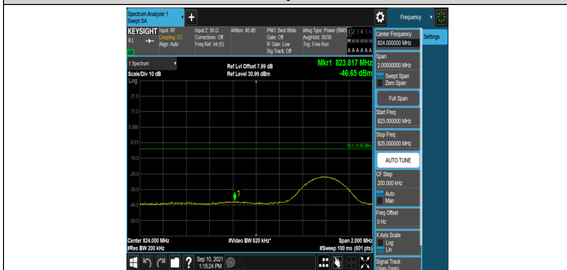
Band5-10MHz-16QAM-20450-1RB#49
