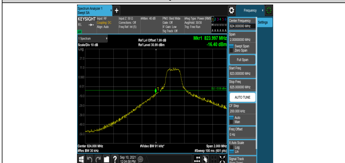
Band5-1.4MHz-16QAM-20407-1RB#0
