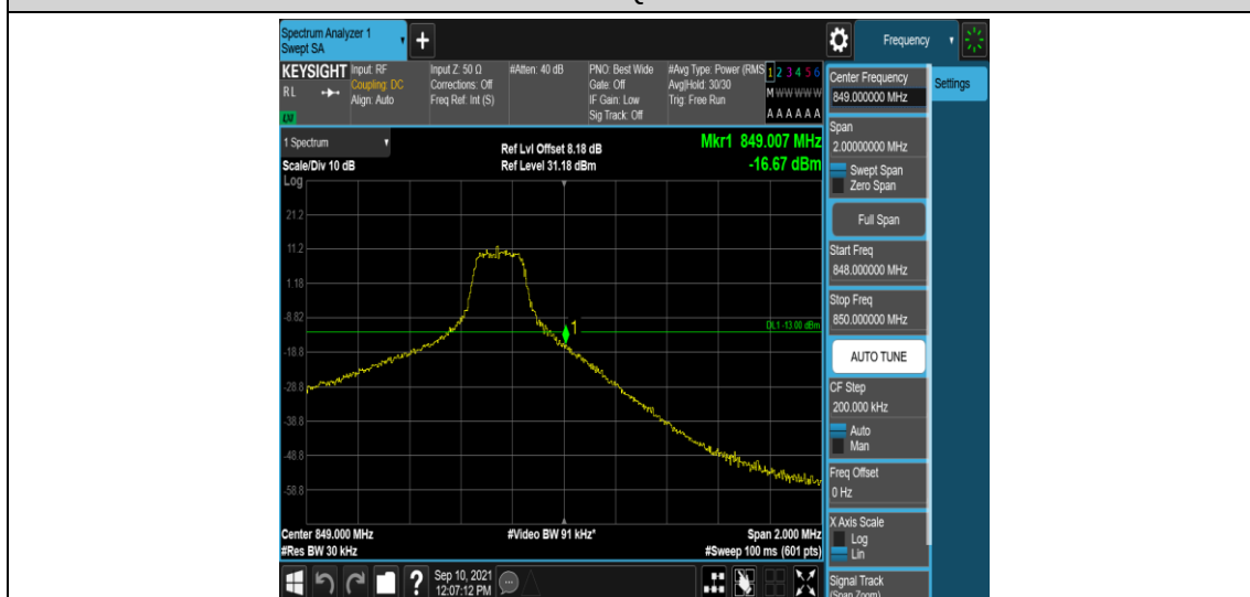
Band5-1.4MHz-16QAM-20643-1RB#5
