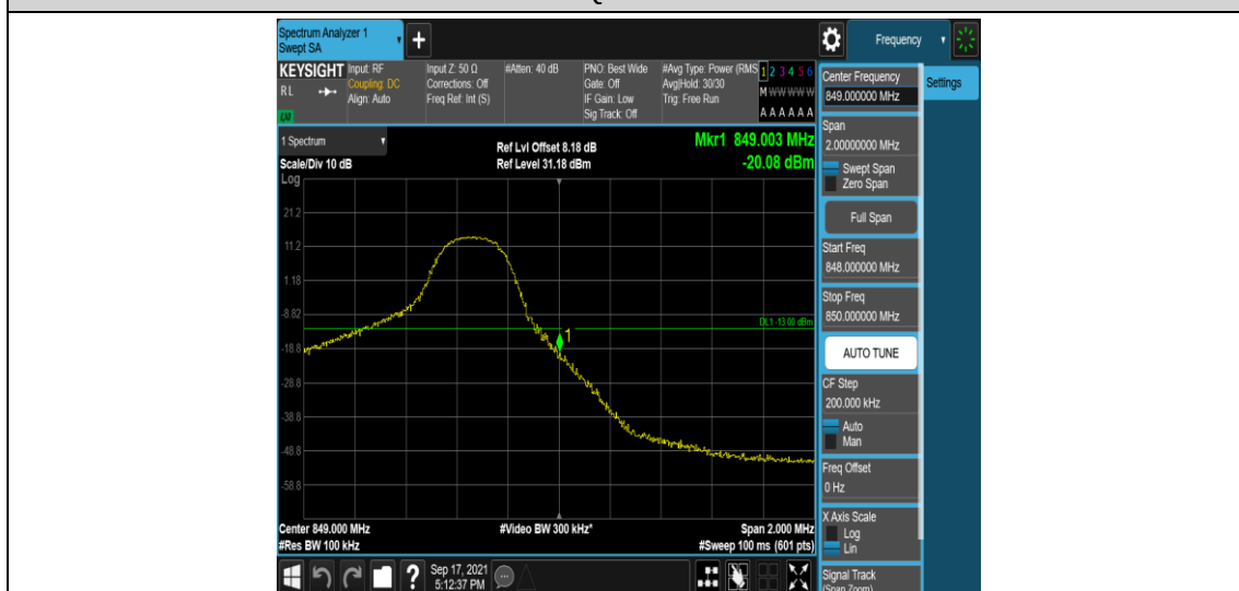
Band5-5MHz-QPSK-20625-1RB#24
