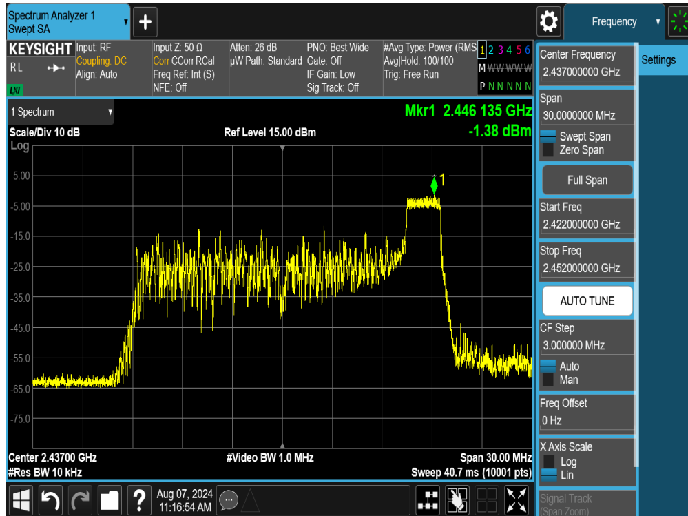
Plot 7-38. Power Spectral Density Plot MIMO ANT2 (802.11ax/be OFDMA – 26 Tones – Ch. 6)
