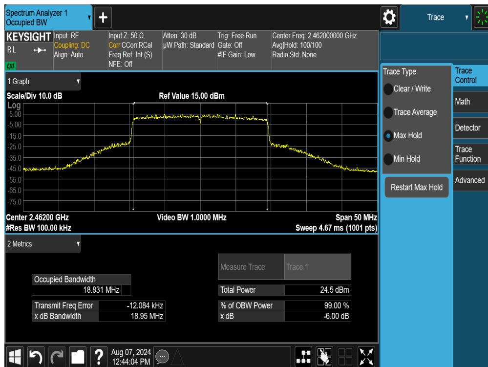
Plot 7-24. 6dB Bandwidth Plot MIMO ANT2 (802.11ax/be OFDMA – 242Tones – Ch. 11)
