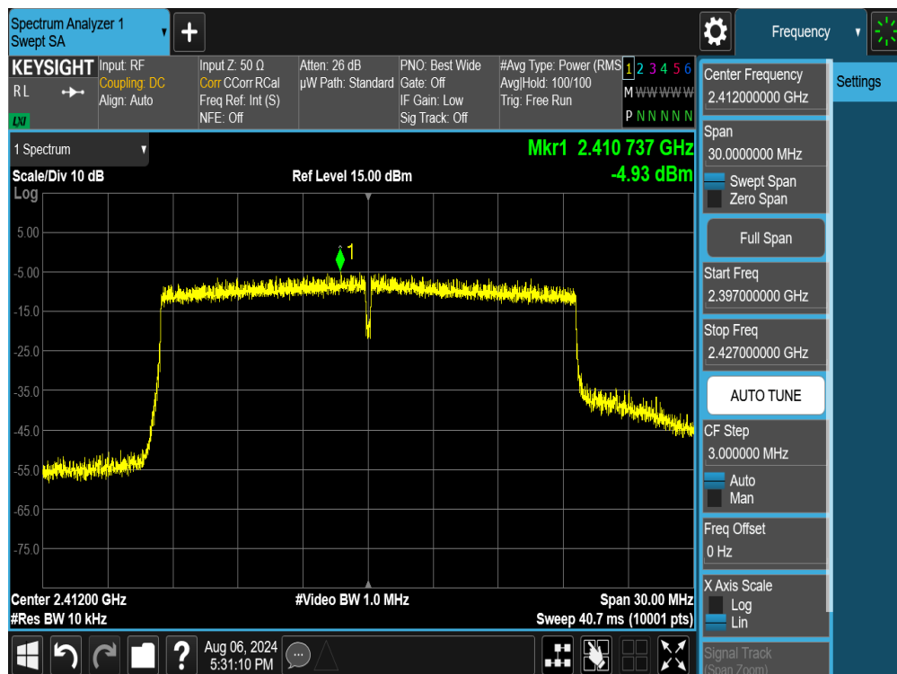
Plot 7-28. Power Spectral Density Plot SISO ANT1 (802.11ax/be OFDMA – 242 Tones – Ch. 1)
