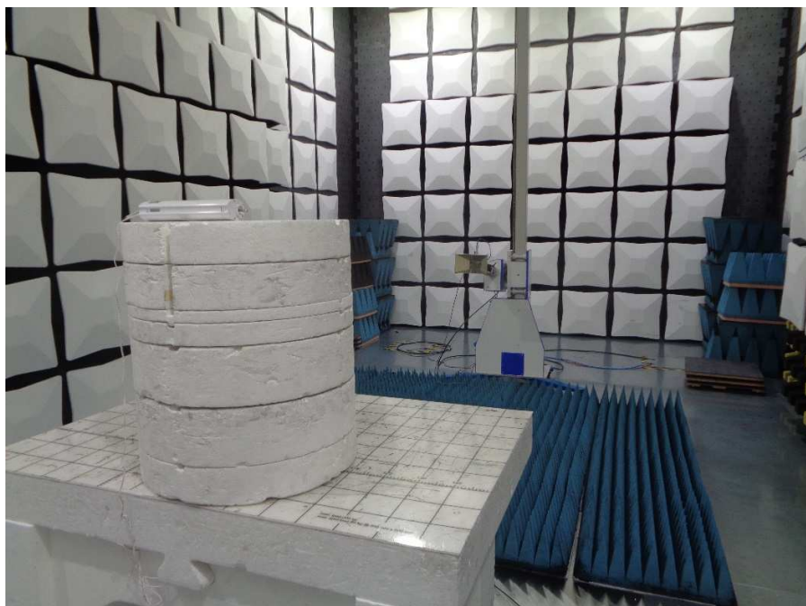
Figure 6: Radiated Spurious Emissions 1 – 18 GHz Back View
