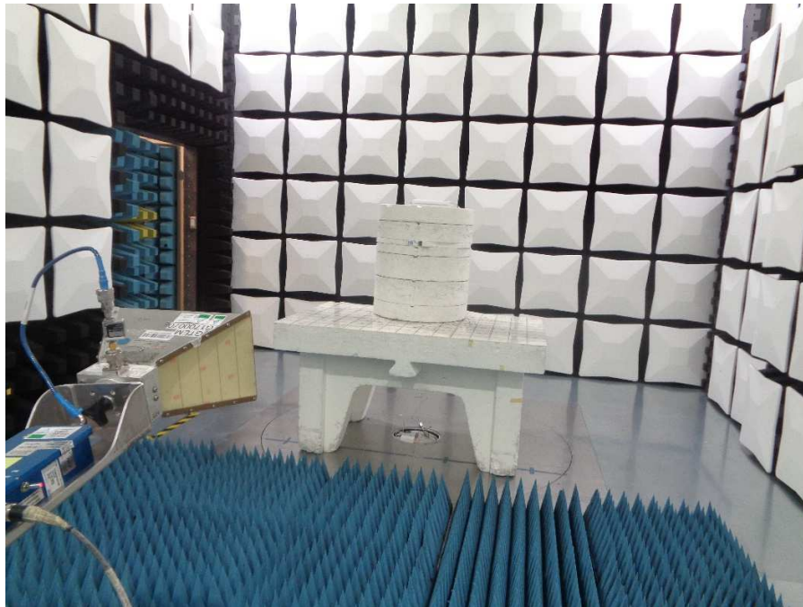
Figure 7: Radiated Spurious Emissions 1 – 18 GHz Front View
