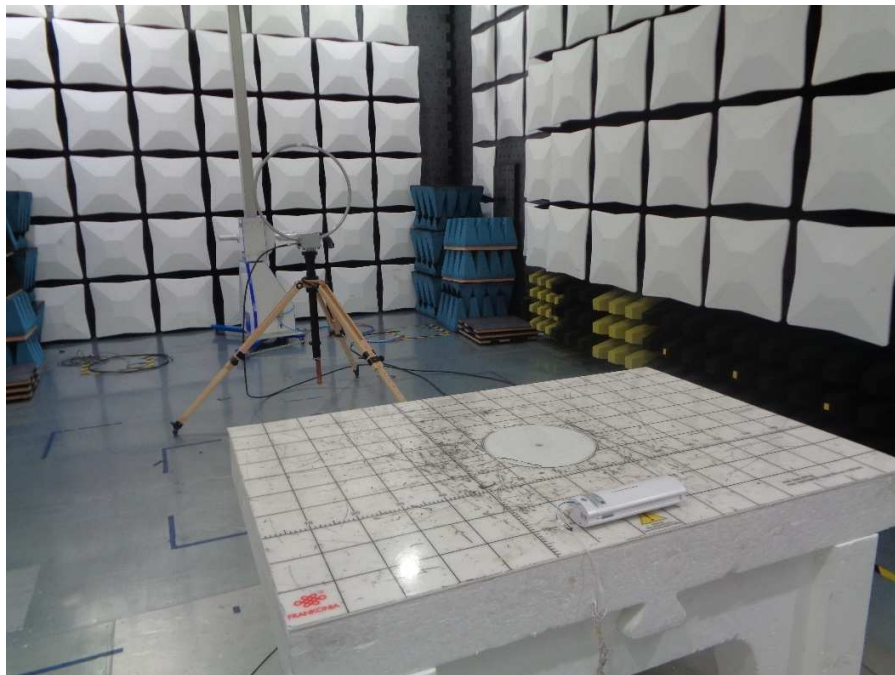
Figure 3: Radiated Spurious Emissions 9 kHz to 30 MHz Back View
