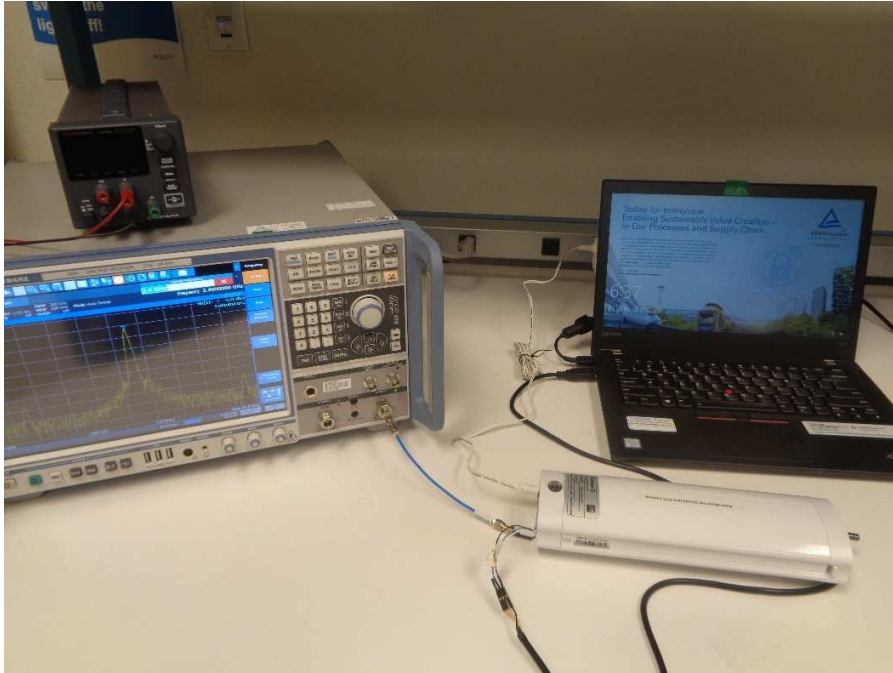
Figure 1: Conducted Testing Setup
