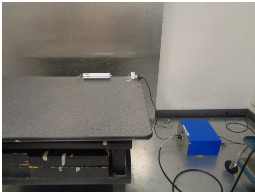
Figure 10: AC Conducted Emissions 150 kHz to 30 MHz Front View
