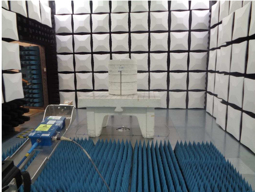
Figure 9: Radiated Spurious Emissions 18 – 26.5 GHz Front View
