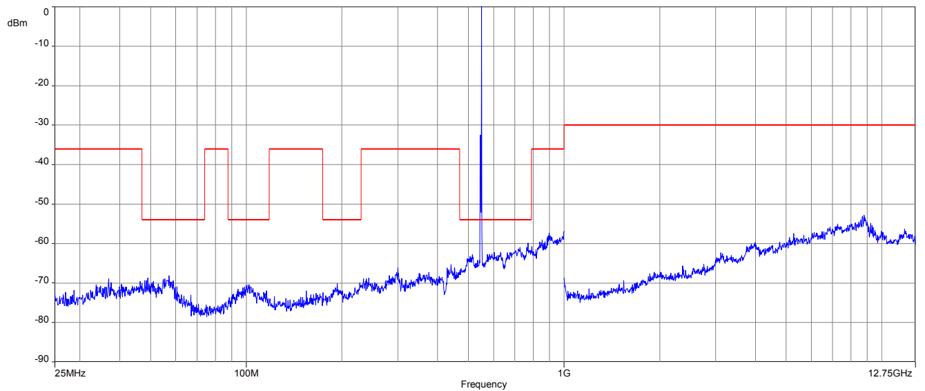
Plot 4: 550.0 MHz, spurious emissions, 25 MHz – 12.75 GHz
