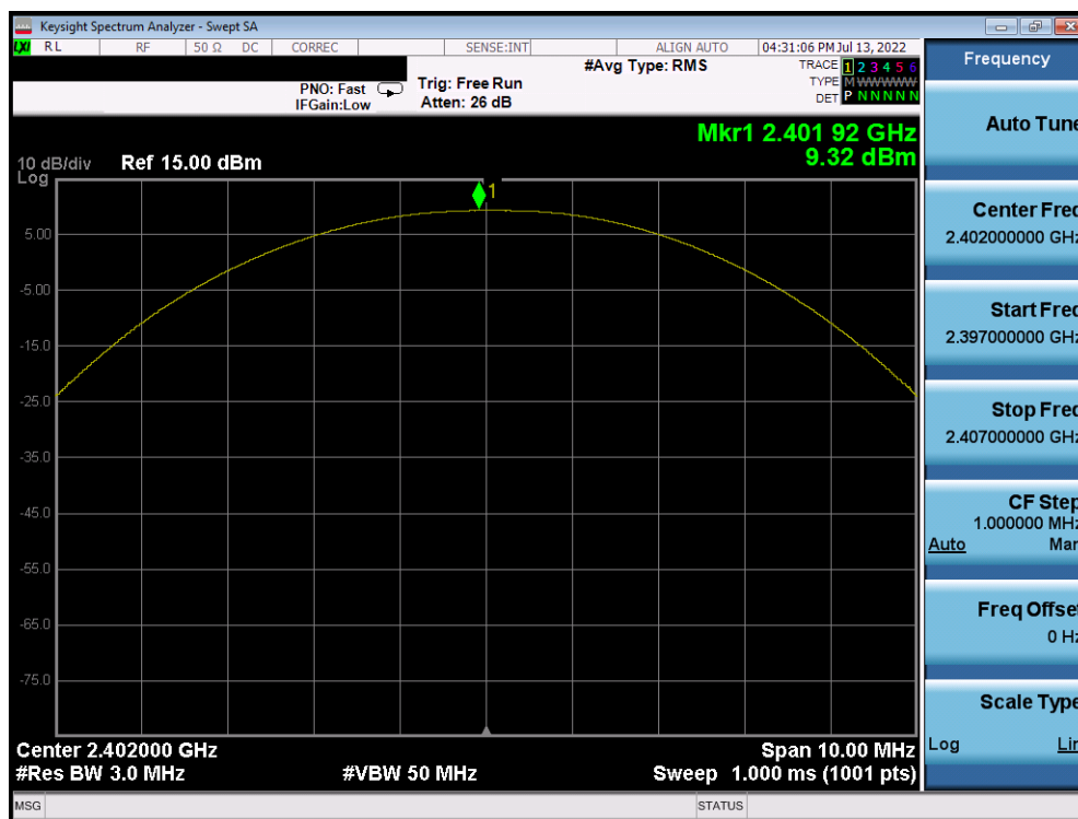
Plot 7-25. Peak Power Plot (Bluetooth (LE), 125kbps – Ch. 0) – ANT 1
