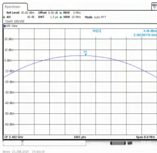
DH5-Ant1-2402-PASS
