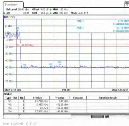
2DH5-Ant1-Hop_2480-PASS
