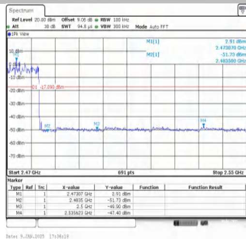
3DH5-Ant1-Hop_2480-PASS
