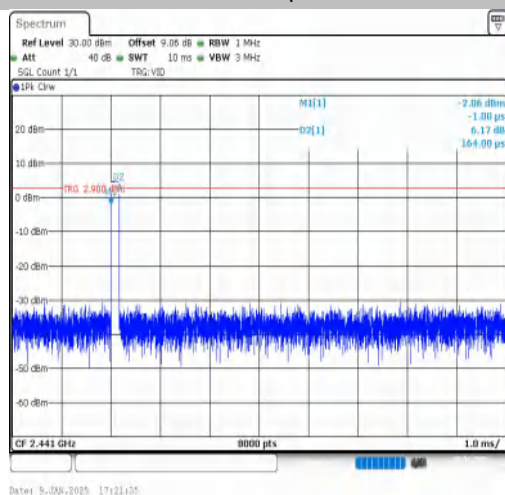
DH3-Ant1-Hop-PASS
