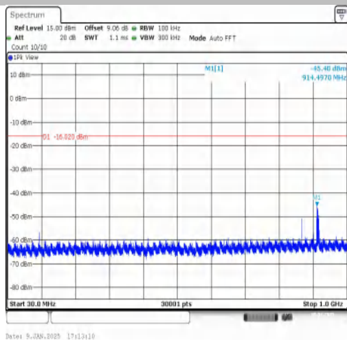
3DH5-Ant1-2441-30~1000-PASS
