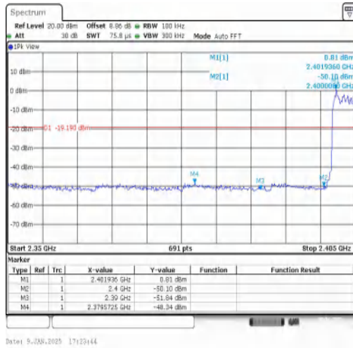
2DH5-Ant1-Hop_2402-PASS
