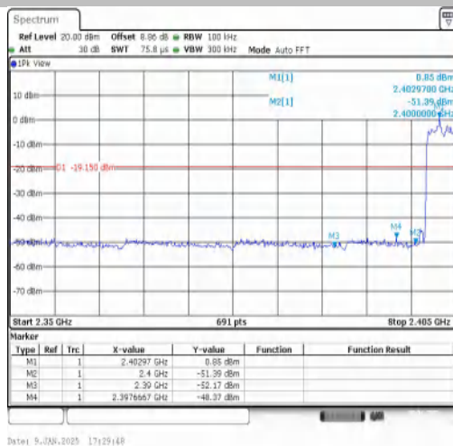
3DH5-Ant1-Hop_2402-PASS
