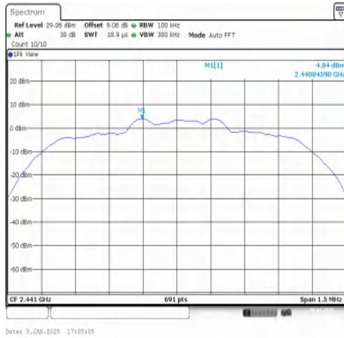
2DH5-Ant1-2441-0~Reference-PASS
