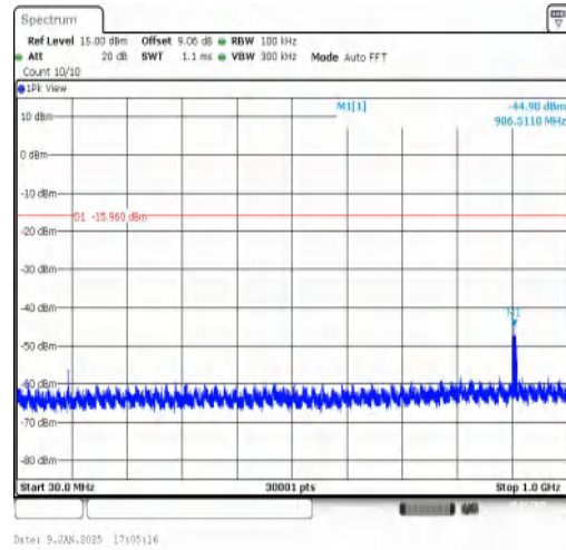
2DH5-Ant1-2441-30~1000-PASS
