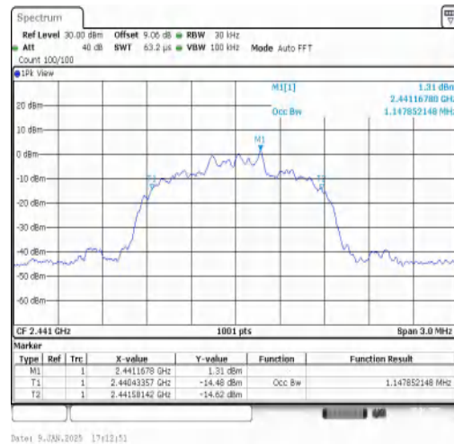
3DH5-Ant1-2441
