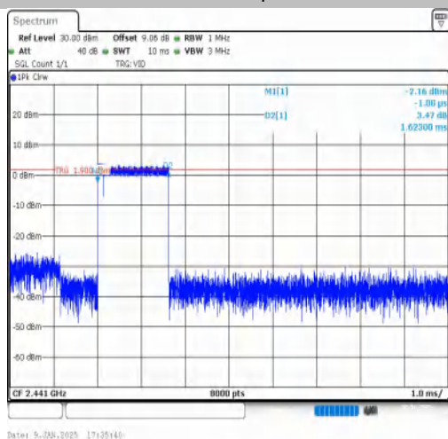
3DH3-Ant1-Hop-PASS
