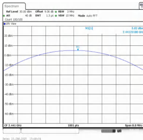
DH5-Ant1-2441-PASS
