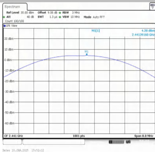
2DH5-Ant1-2441-PASS
