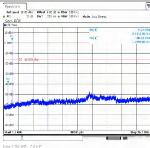
3DH5-Ant1-2441-1000~26500-PASS
