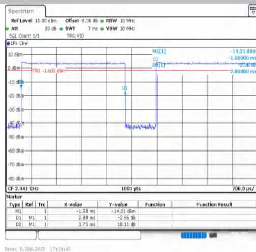
NTNV-2DH5-Ant1-2441
