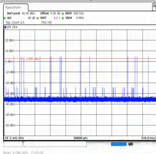
DH3-Ant1-Hop-PASS
