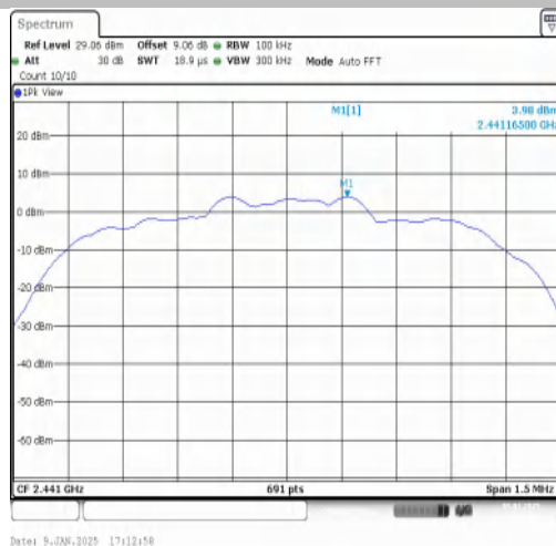
3DH5-Ant1-2441-0~Reference-PASS
