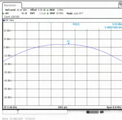
2DH5-Ant1-2480-PASS
