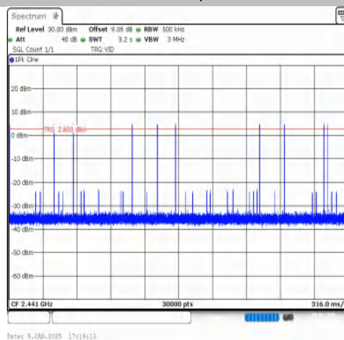
DH5-Ant1-Hop-PASS
