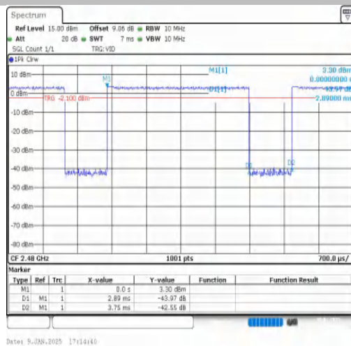
NTNV-3DH5-Ant1-2480
