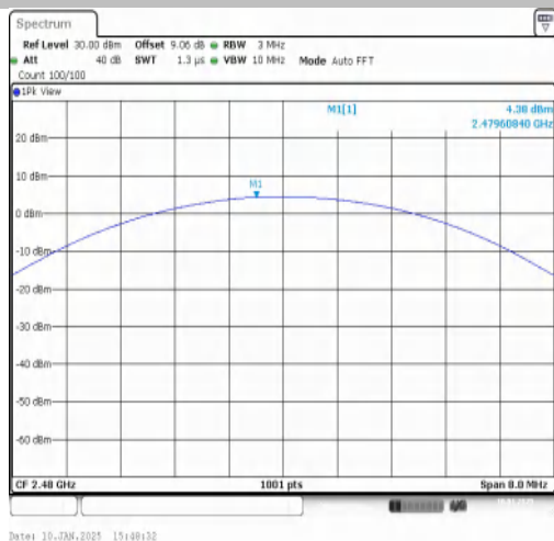
DH5-Ant1-2480-PASS
