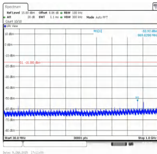
3DH5-Ant1-2402-30~1000-PASS
