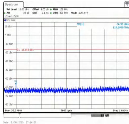
3DH5-Ant1-2480-30~1000-PASS
