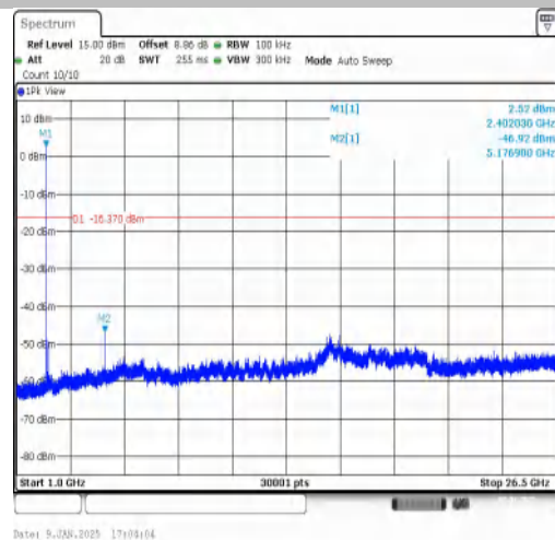
2DH5-Ant1-2402-1000~26500-PASS
