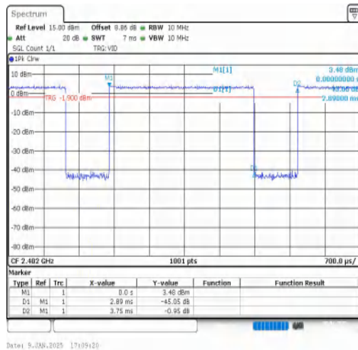
NTNV-3DH5-Ant1-2402
