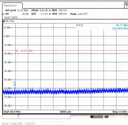
2DH5-Ant1-2402-30~1000-PASS
