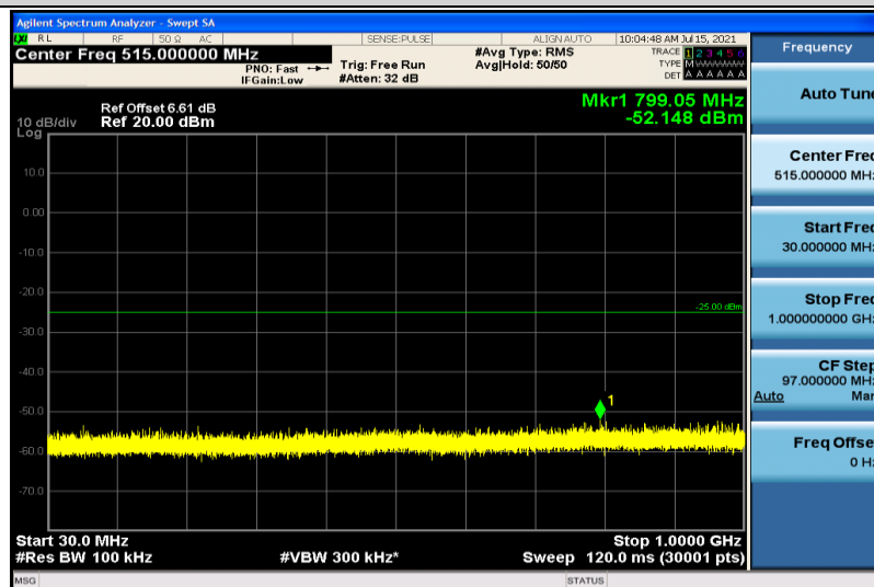
Band38-5MHz-16QAM-37775-1RB#0-30~1000MHz
