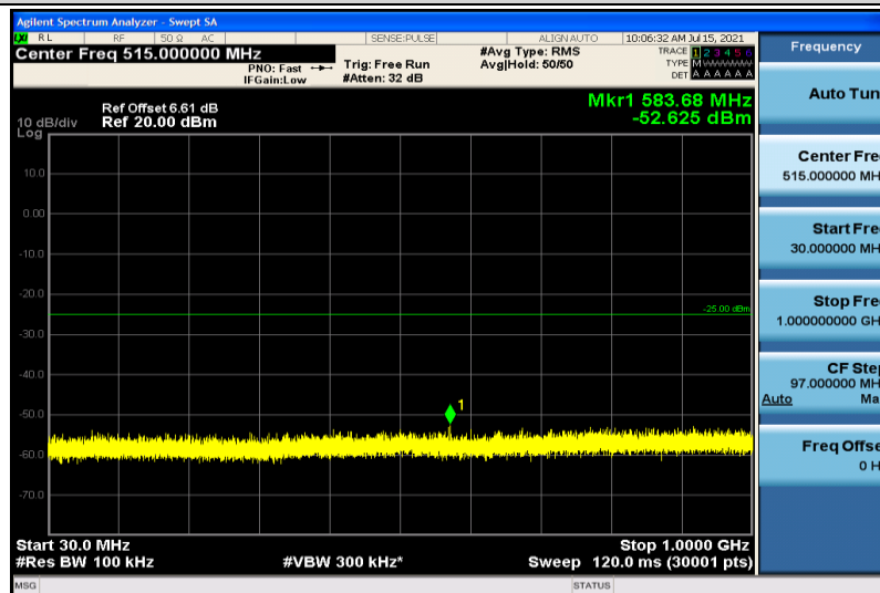
Band38-5MHz-16QAM-38000-1RB#0-30~1000MHz
