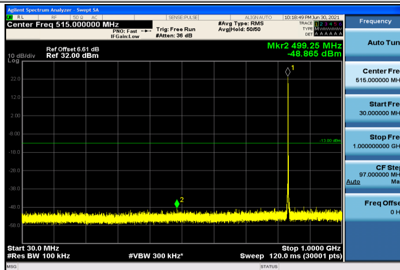
Band5-1.4MHz-QPSK-20525-1RB#0-30~1000MHz
