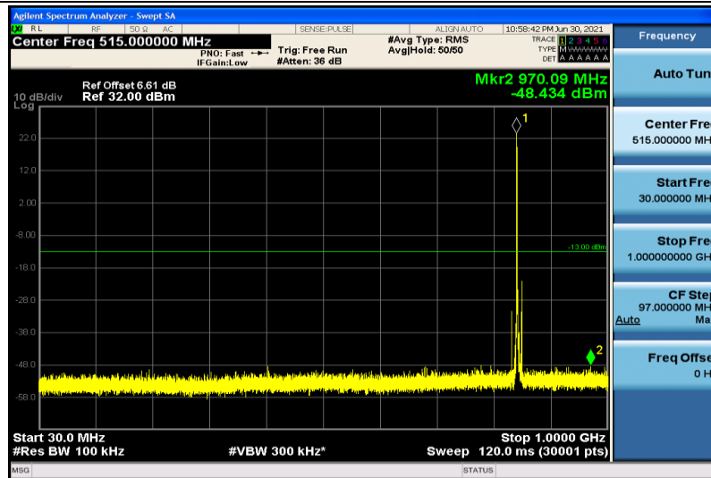
Band5-5MHz-QPSK-20625-1RB#0-30~1000MHz
