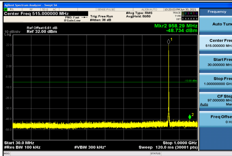
Band5-1.4MHz-QPSK-20643-1RB#0-30~1000MHz
