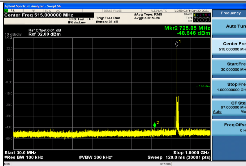
Band5-5MHz-16QAM-20525-1RB#0-30~1000MHz
