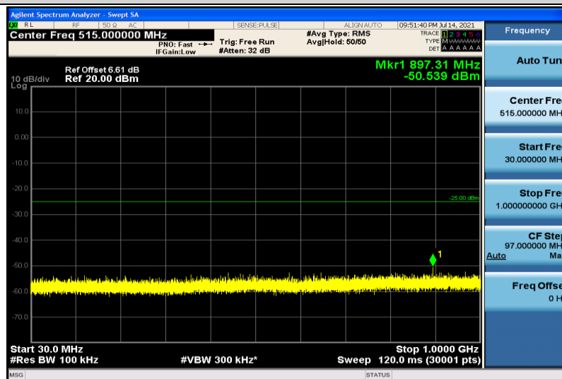
Band38-15MHz-16QAM-37825-1RB#0-30~1000MHz
