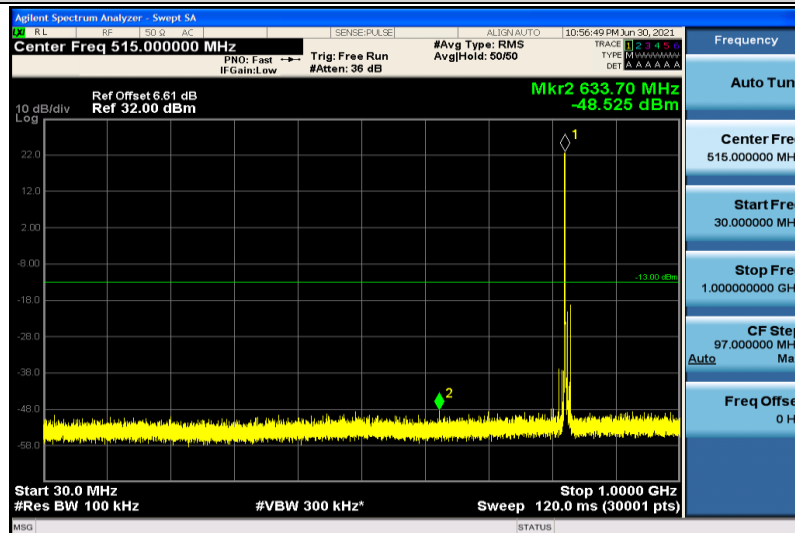
Band5-5MHz-16QAM-20425-1RB#0-30~1000MHz
