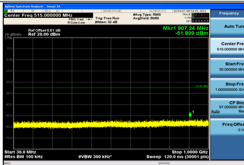
Band38-5MHz-QPSK-37775-1RB#0-30~1000MHz
