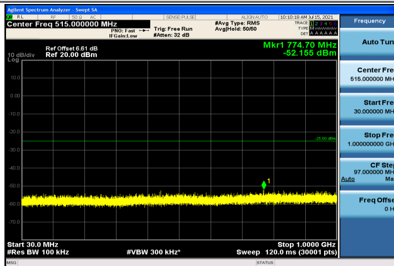
Band38-20MHz-QPSK-38000-1RB#0-30~1000MHz
