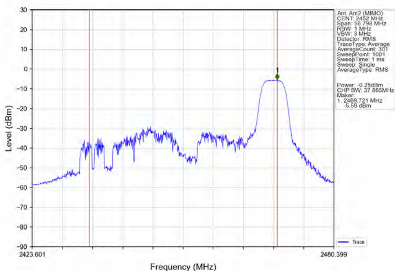
802.11ax(HE40) HCH 2452MHz RU52 Right Ant2 (MIMO) NTN
