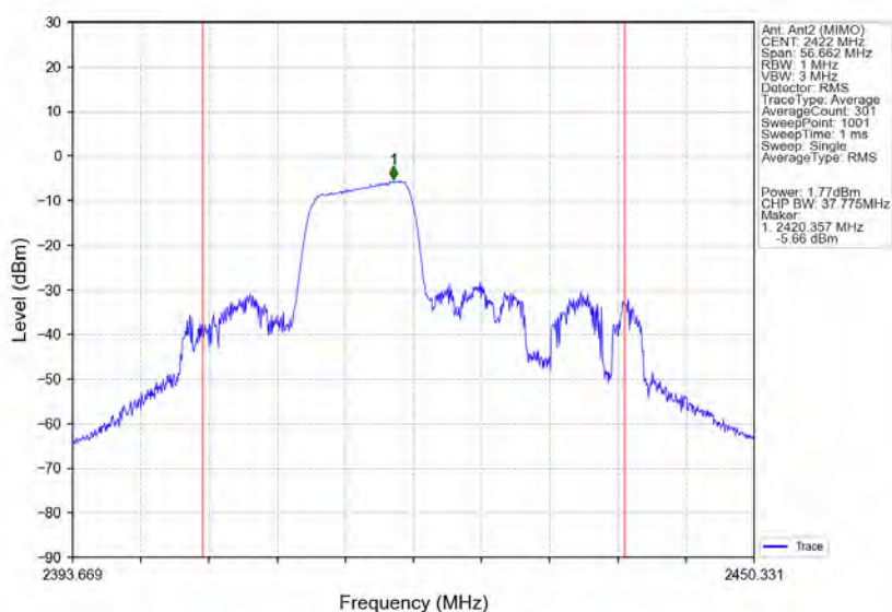
802.11ax(HE40) LCH 2422MHz RU106 Mid Ant2 (MIMO) NTVN
