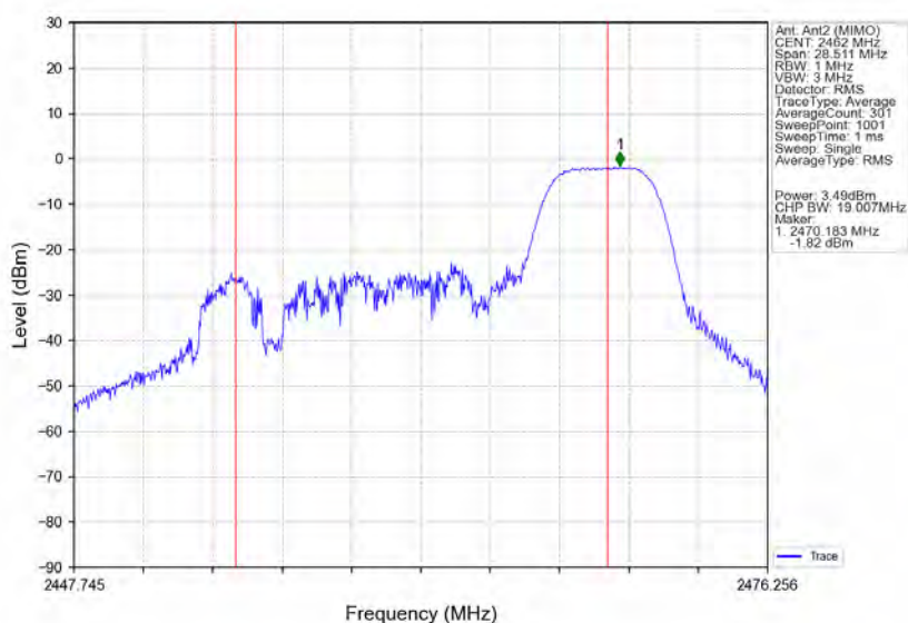
802.11ax(HE20) HCH 2462MHz RU52 Right Ant2 (MIMO) NTN
