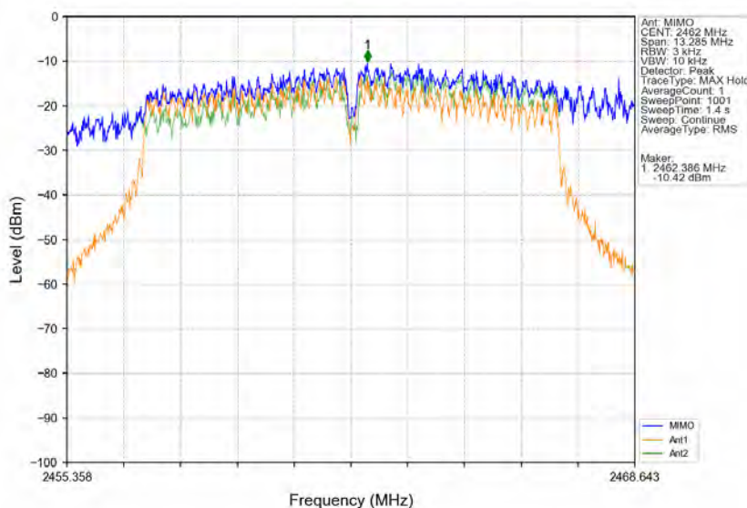
802.11g HCH 2462MHz MIMO NTN
