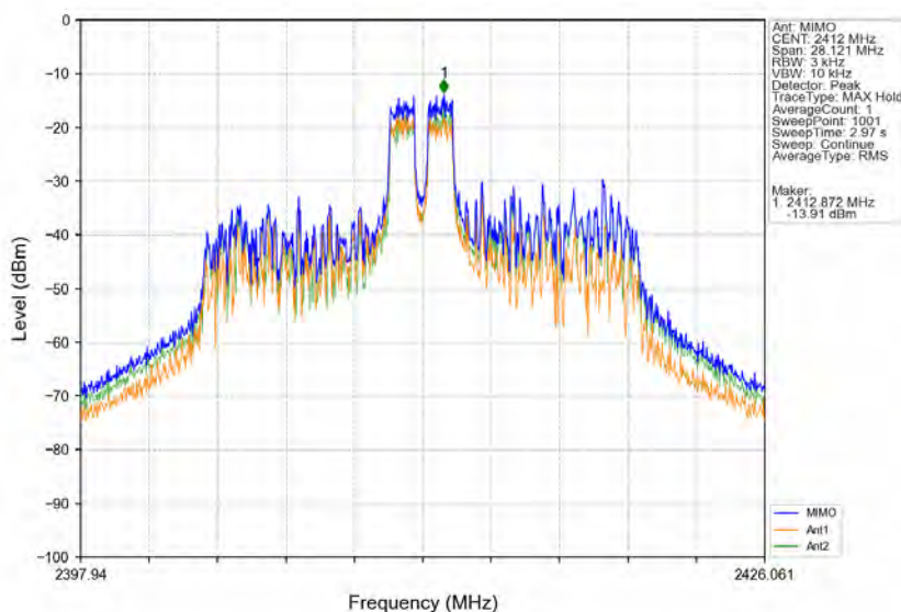
802.11ax(HE20) LCH_2412MHz_RU26_Mid_MIMO NTN
