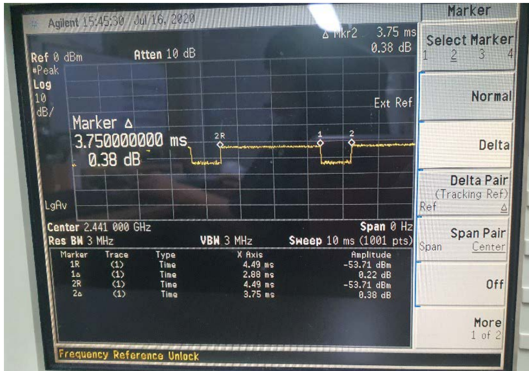
Figure 8.2 Bluetooth Transmission Plot
