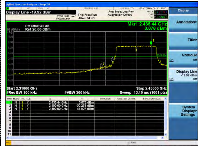
Left bandedge
