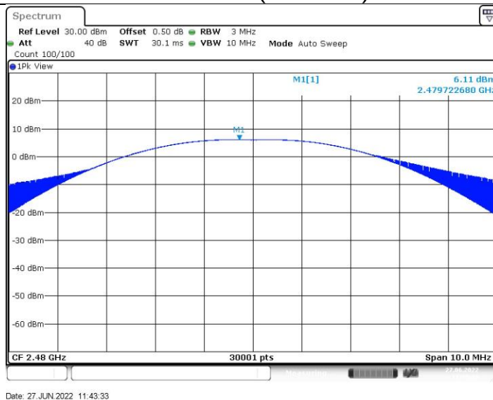
Channel 39 (2480MHz)
