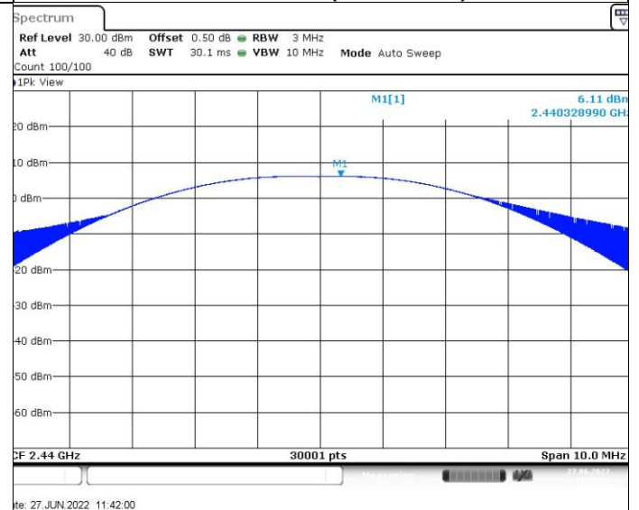
Channel 19 (2440MHz)
