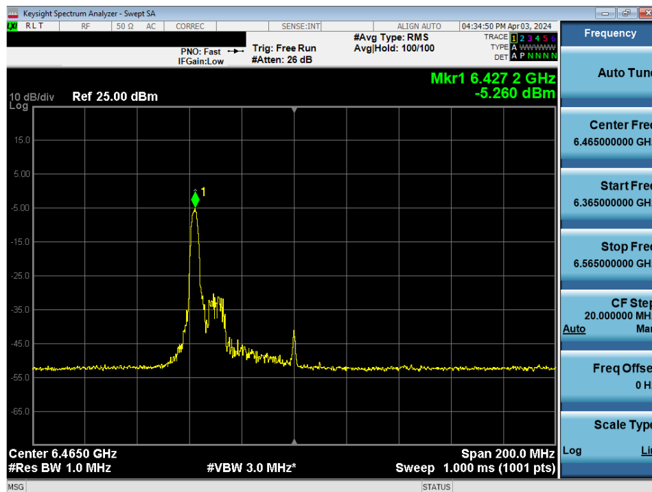
Plot 7-90. Power Spectral Density Plot MIMO ANT1 (80MHz BW 802. 11be (26 Tones) (UNII Band 6) – Ch. 103)
