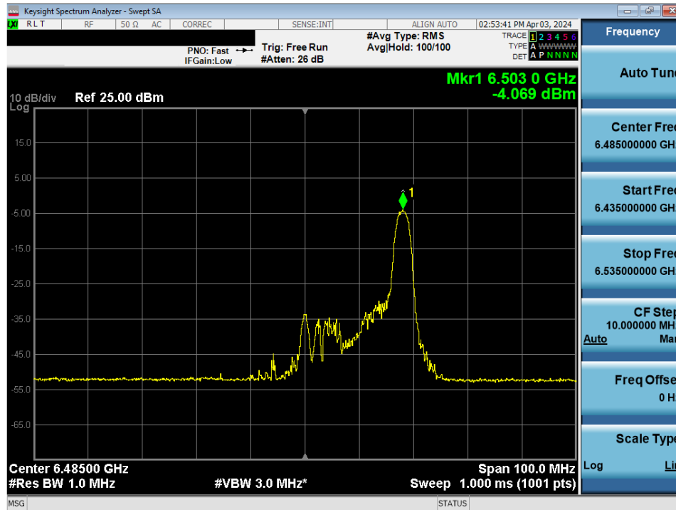
Plot 7-89. Power Spectral Density Plot MIMO ANT1 (40MHz BW 802. 11be (26 Tones) (UNII Band 6) – Ch. 107)
