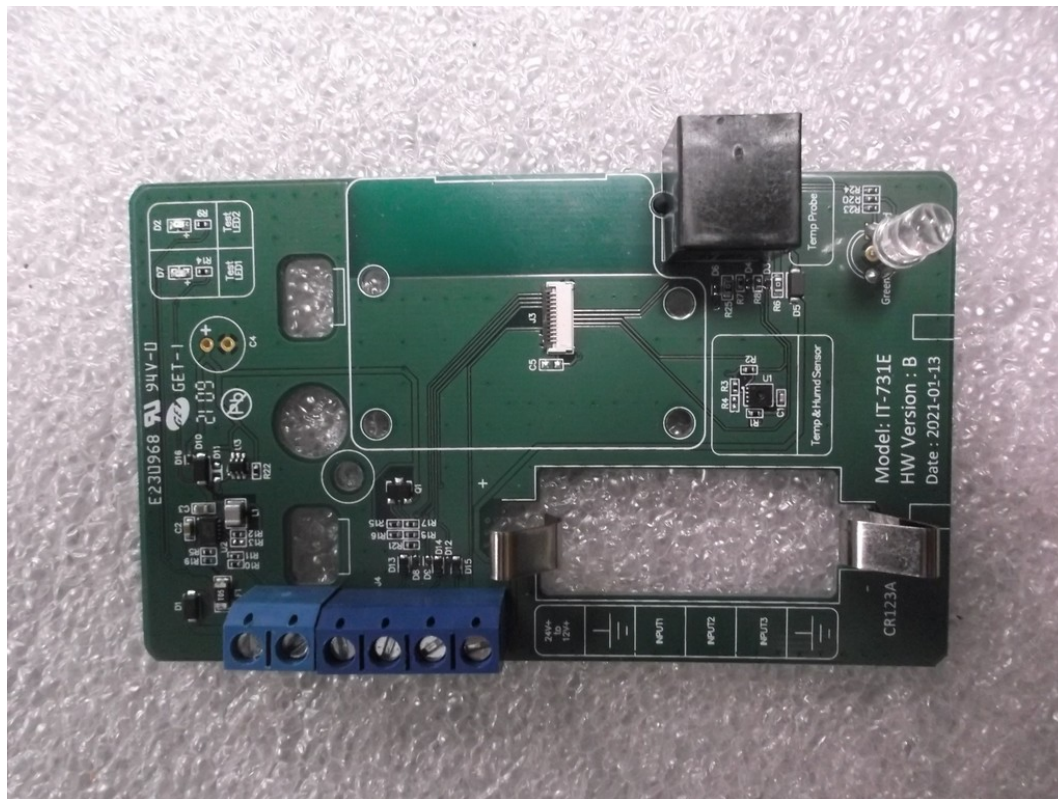
PCB Component Side View
