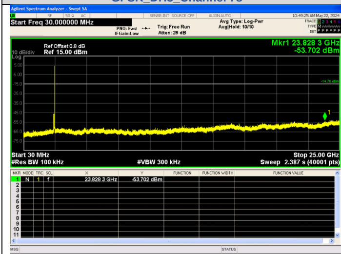
30.0 MHz - 25000.0 MHz GFSK_DH5_Channel 78
