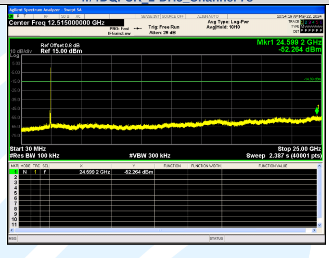
30.0 MHz - 25000.0 MHz \pi/4 DQPSK_2-DH5_Channel 78
