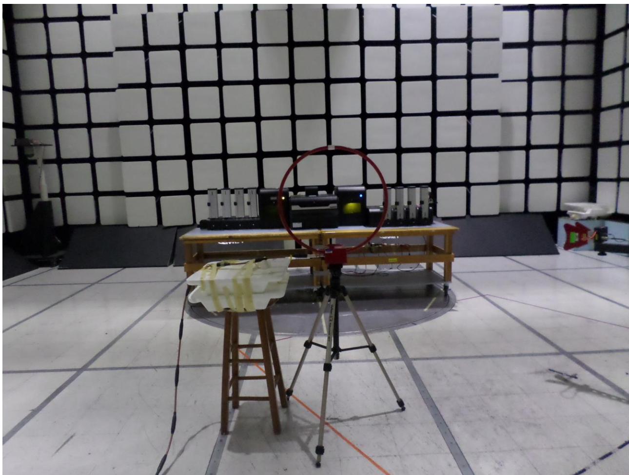
Figure 6: Radiated Spurious Emissions - 0.009-30 MHz, 0-Degrees, Front View
