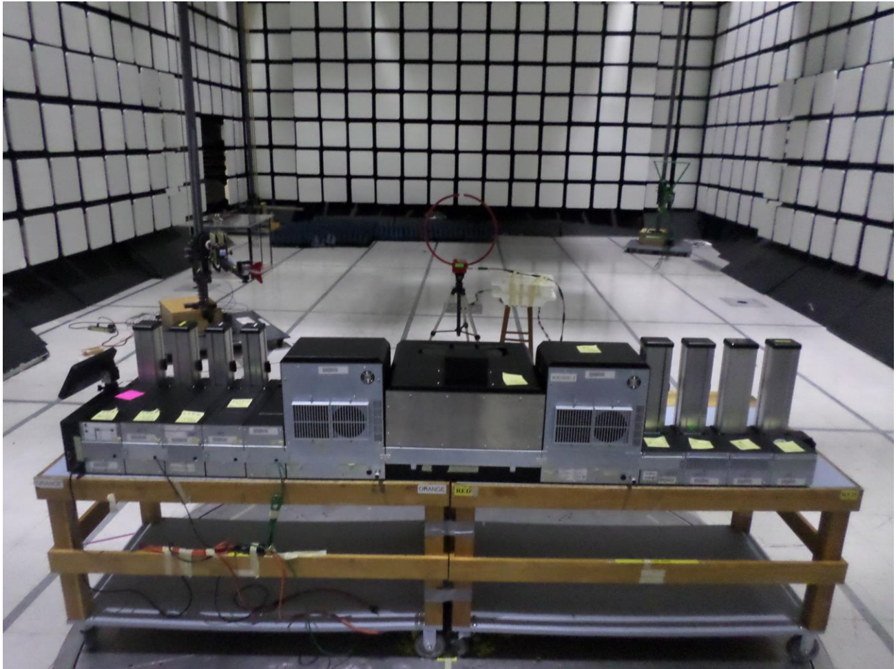
Figure 7: Radiated Spurious Emissions - 0.009-30 MHz, 0-Degrees, Rear View
