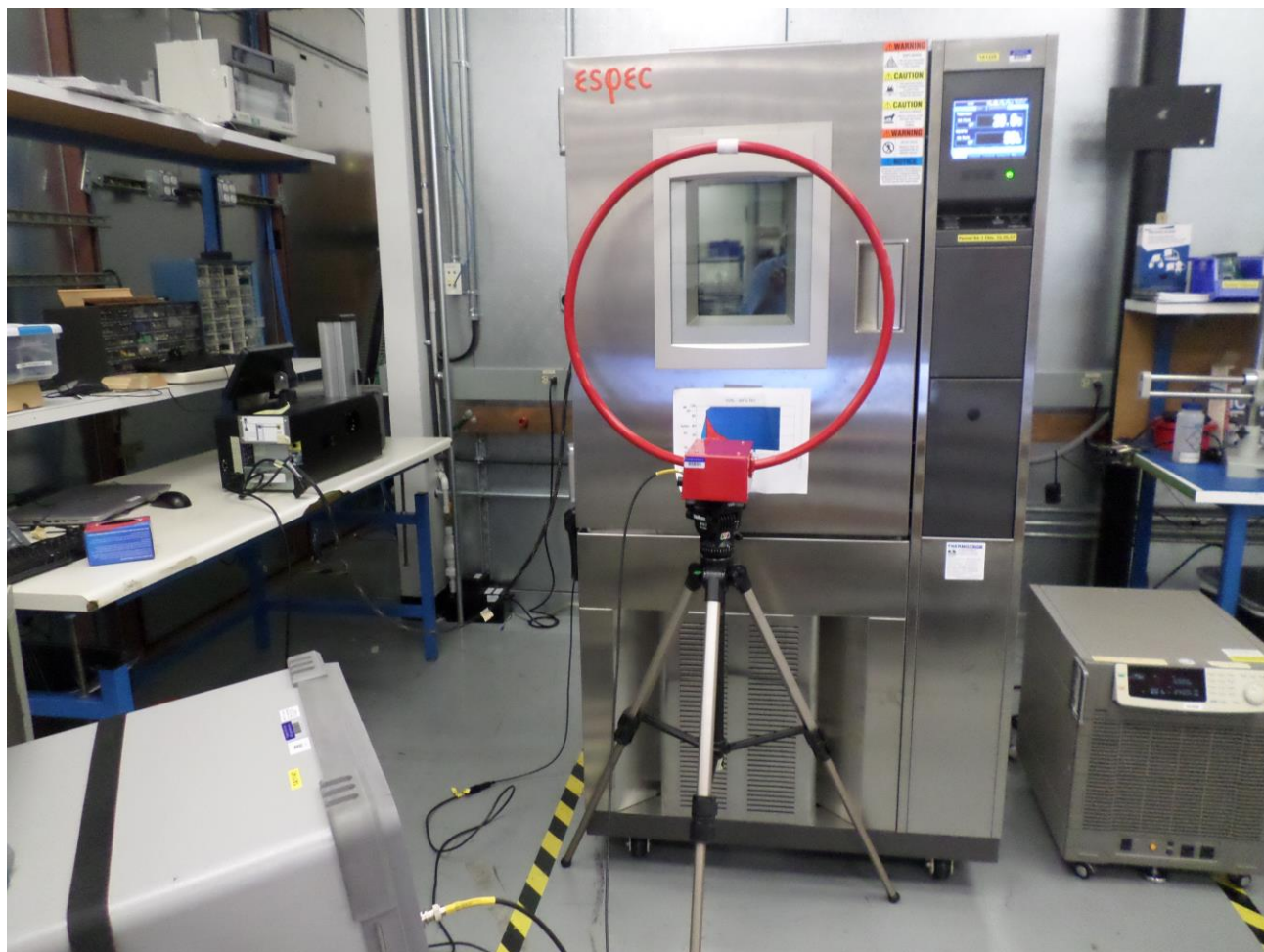
Figure 5: Frequency Stability Setup Photo
