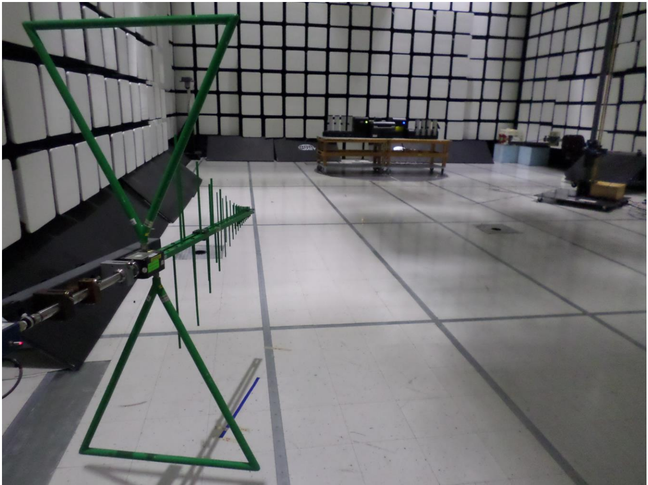
Figure 12: Radiated Spurious Emissions - 30-1000 MHz, Antenna View
