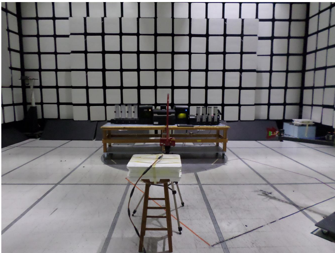
Figure 8: Radiated Spurious Emissions - 0.009-30 MHz, 90-Degrees, Front View
