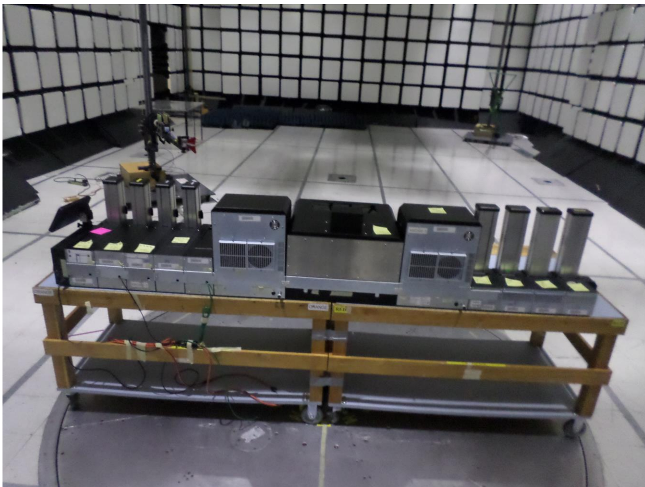
Figure 11: Radiated Spurious Emissions - 30-1000 MHz, Rear View
