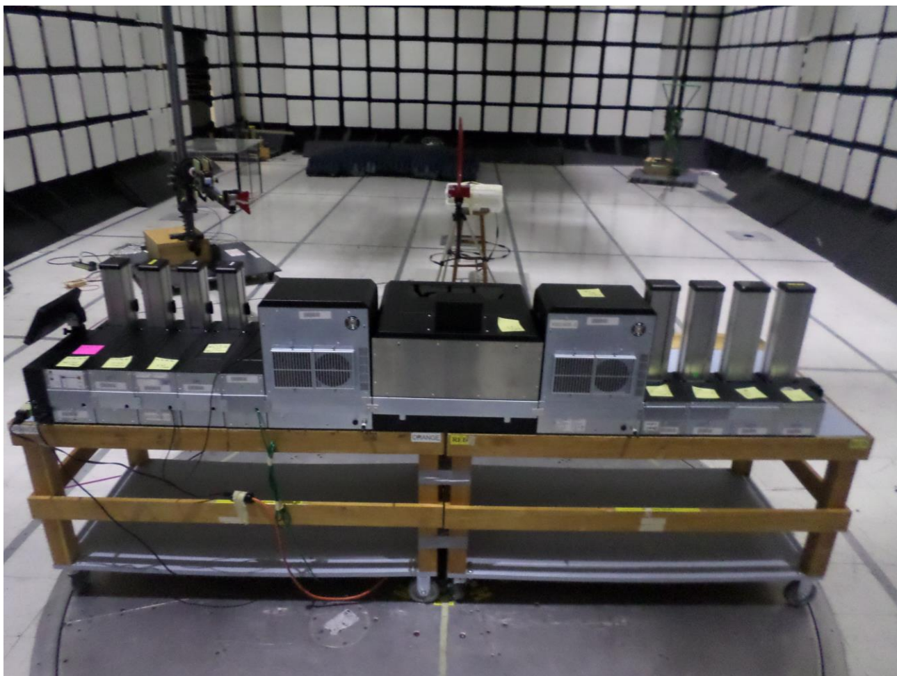
Figure 9: Radiated Spurious Emissions - 0.009-30 MHz, 90-Degrees, Rear View
