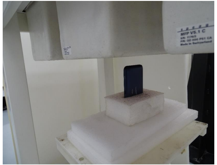
Photo 11: Right Side 20mm
