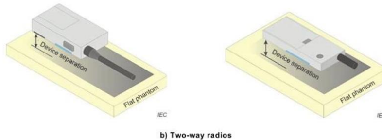
Figure 10 – Test positions for front-of-face devices
