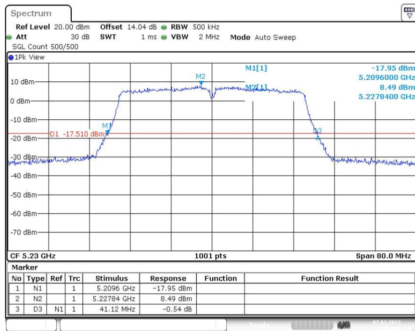
Fig. 14 Occupied 26dB Bandwidth (802.11ac-VHT40, 5230MHz)
