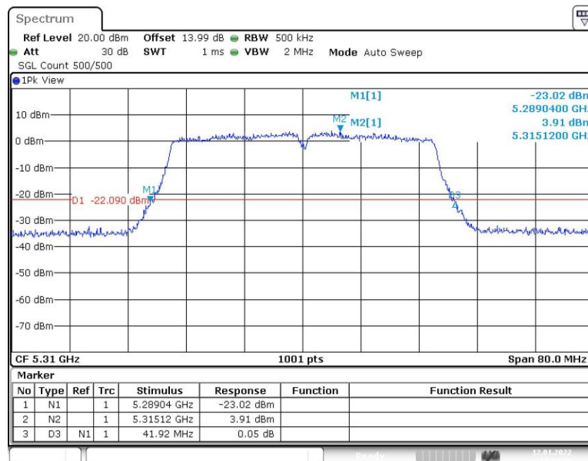
Fig. 16 Occupied 26dB Bandwidth (802.11ac-VHT40, 5310MHz)
