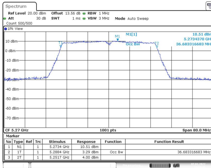
Fig. 47 99% Occupied Bandwidth (802.11ac-VHT40, 5270MHz)
