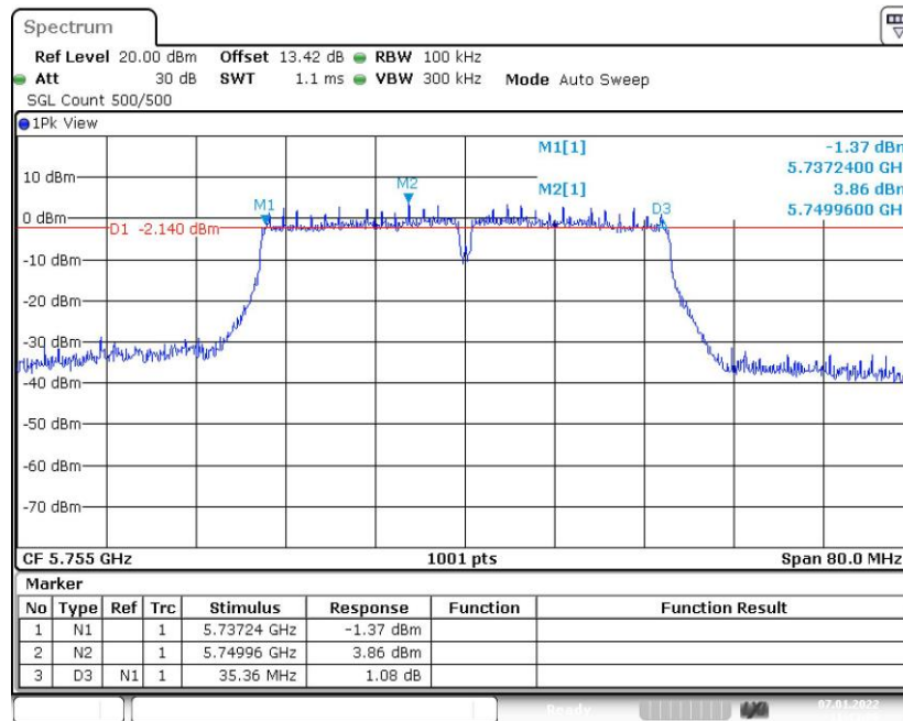
Fig. 30 Occupied 6dB Bandwidth (802.11ac-VHT40, 5755MHz)
