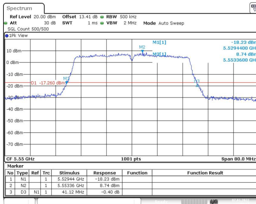
Fig. 18 Occupied 26dB Bandwidth (802.11ac-VHT40, 5550MHz)
