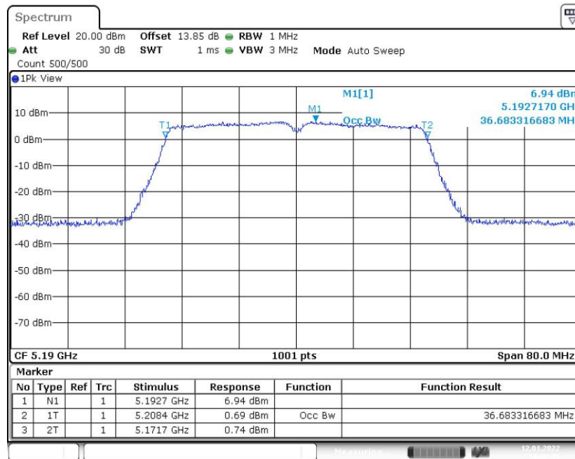
Fig. 45 99% Occupied Bandwidth (802.11ac-VHT40, 5190MHz)
