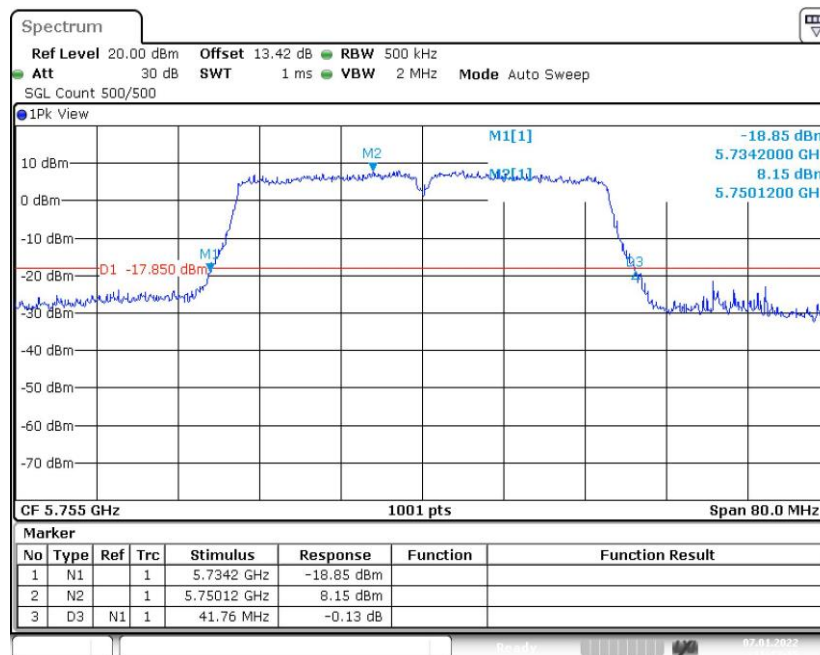
Fig. 20 Occupied 26dB Bandwidth (802.11ac-VHT40, 5755MHz)
