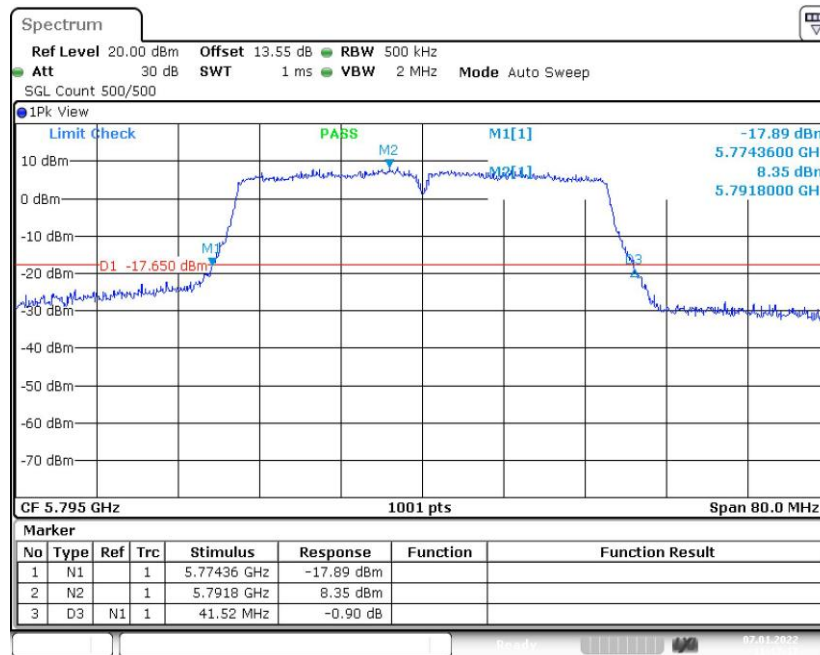
Fig. 21 Occupied 26dB Bandwidth (802.11ac-VHT40, 5795MHz)
