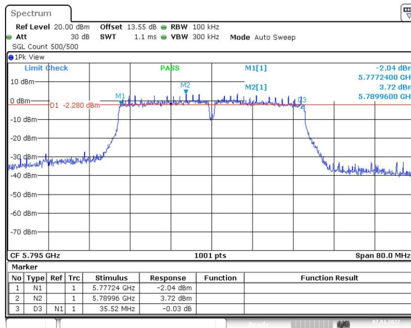
Fig. 31 Occupied 6dB Bandwidth (802.11ac-VHT40, 5795MHz)
