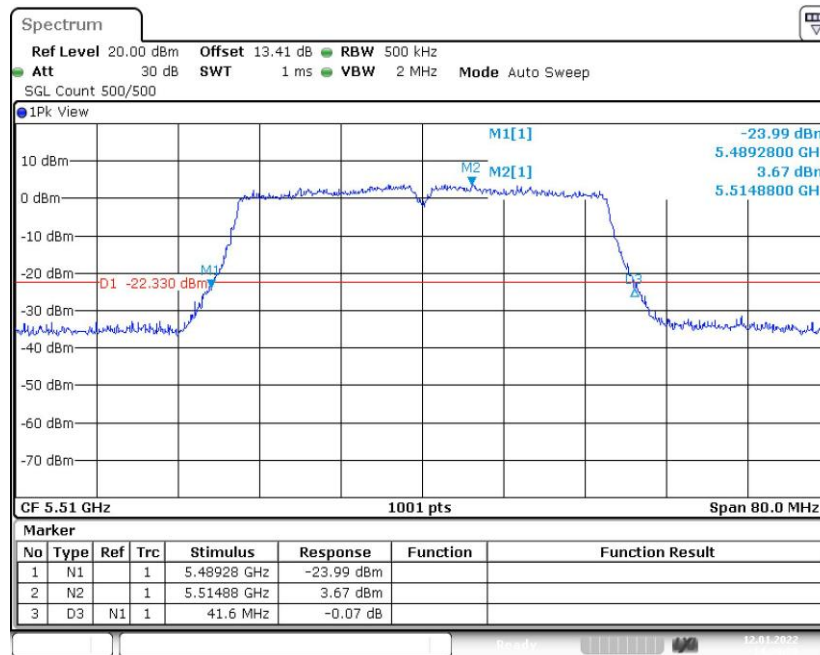
Fig. 17 Occupied 26dB Bandwidth (802.11ac-VHT40, 5510MHz)
