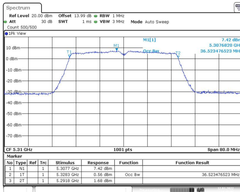
Fig. 48 99% Occupied Bandwidth (802.11ac-VHT40, 5310MHz)
