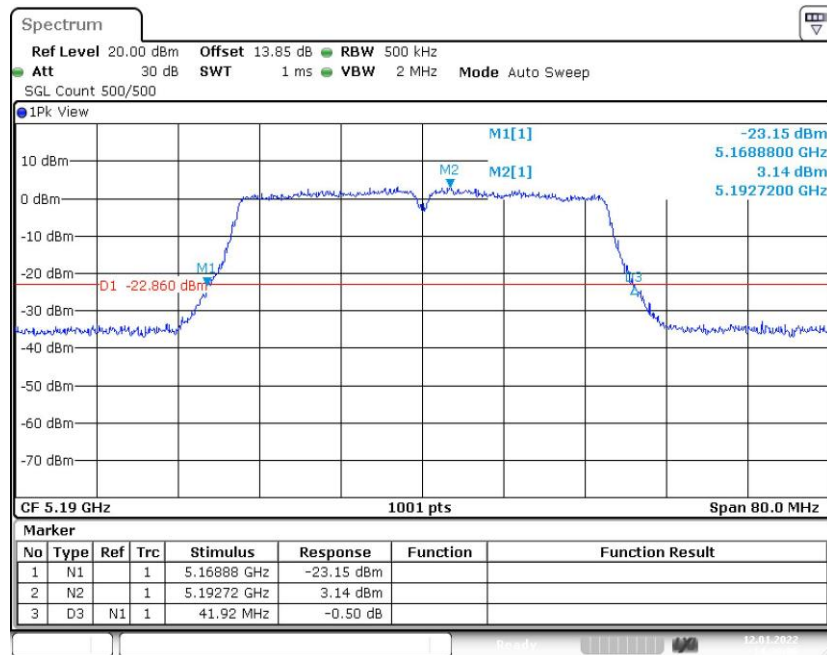
Fig. 13 Occupied 26dB Bandwidth (802.11ac-VHT40, 5190MHz)
