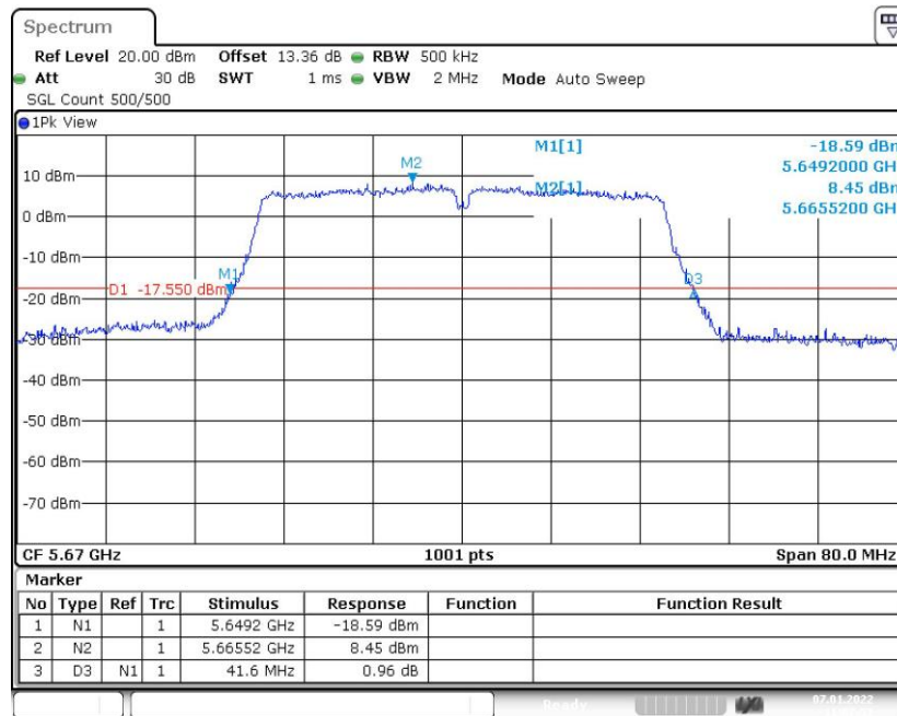
Fig. 19 Occupied 26dB Bandwidth (802.11ac-VHT40, 5670MHz)
