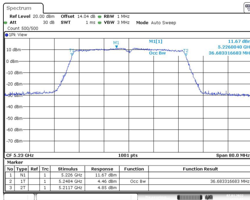
Fig. 46 99% Occupied Bandwidth (802.11ac-VHT40, 5230MHz)
