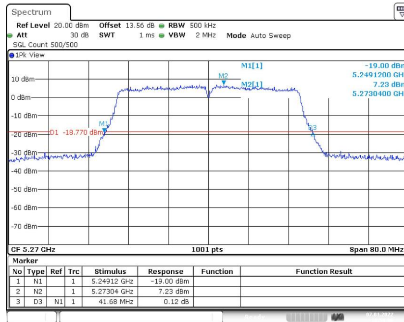
Fig. 15 Occupied 26dB Bandwidth (802.11ac-VHT40, 5270MHz)
