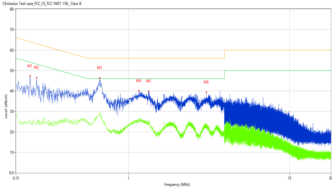
Figure 58: Conducted Emission on AC Mains, L Phase
