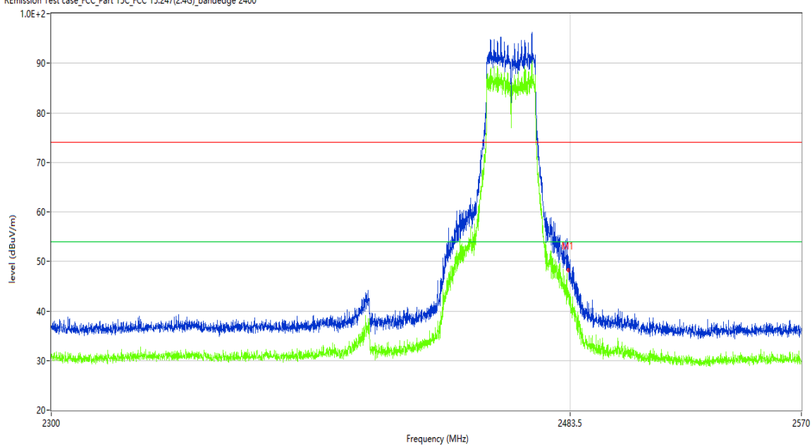
Figure 55: Band Edge (Restricted-band band-edge), 802.11n(HT20), 2462MHz Horizontal
