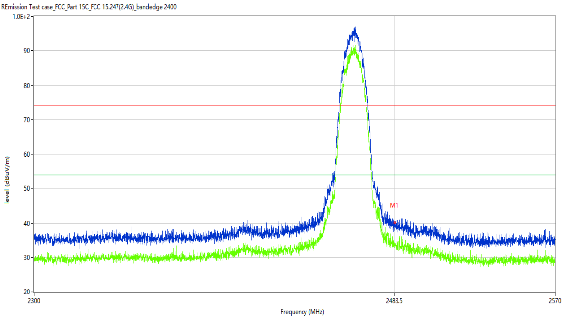
Figure 51: Band Edge (Restricted-band band-edge), 802.11b, 2462MHz Horizontal
