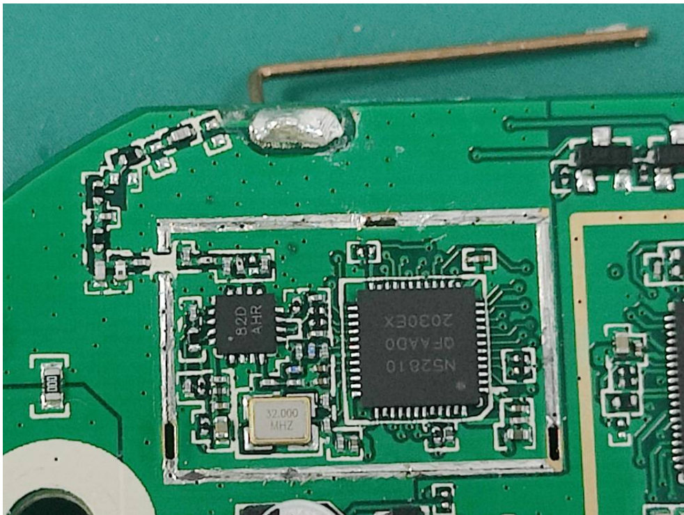
FHSS ANT
