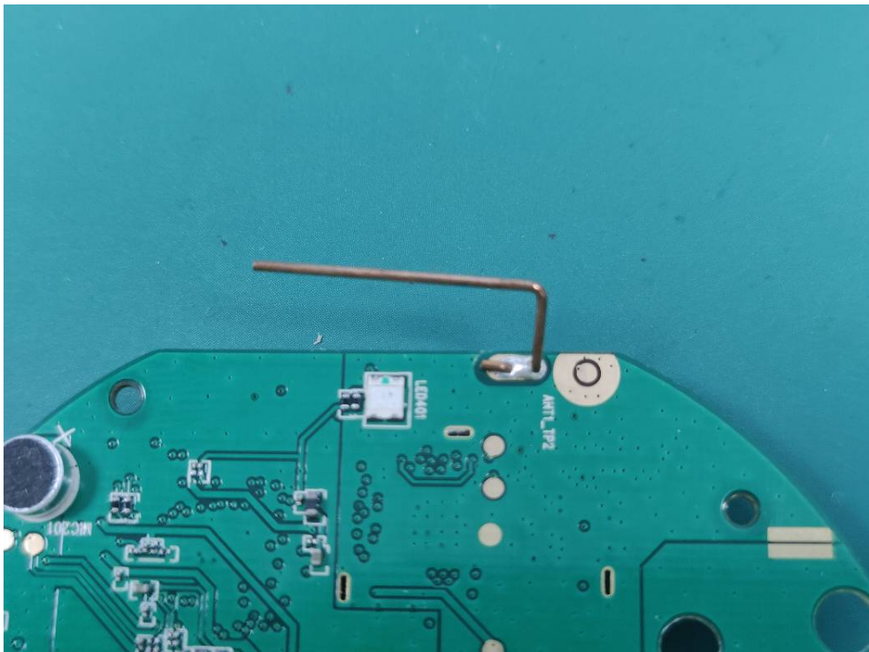
FHSS ANT
