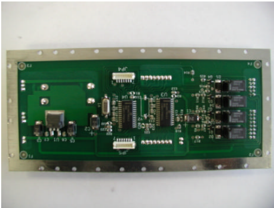
Logic Board Front View
