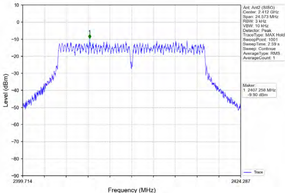
802.11g LCH 2412MHz Ant2 (SISO) NTVN
