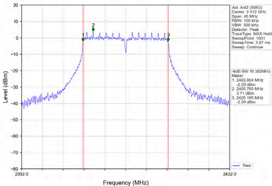
802.11g LCH 2412MHz Ant2 (SISO) NTV
