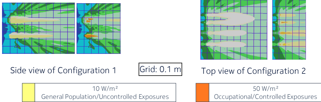
Figure 4 – Power density from AWEWA/B (or FA3WA) for the actual maximum transmitted power of 0.36 W (corresponding to the actual EIRP threshold of 49.52 dBm) and the beam oriented in azimuth = 0° & elevation = 0°, together with the power density from FA3UB (or AWEUC/D) for the actual maximum transmitted power of 0.19 W (corresponding to the actual EIRP threshold of 49.52 dBm) and the beam oriented in azimuth = 0° & elevation = 0°
