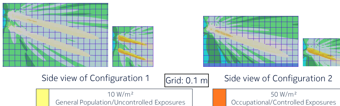
Figure 7 – Power density from AWEWA/B (or FA3WA) for the time-averaged maximum transmitted power of 1.42 W (corresponding to the time-averaged maximum EIRP of 55.52 dBm) and the beam oriented in azimuth = 0° & elevation = +20°, together with the power density from FA3UB (or AWEUC/D) for the time-averaged maximum transmitted power of 0.76 W (corresponding to the time-averaged maximum EIRP of 55.52 dBm) and the beam oriented in azimuth = 0° & elevation = +15°
