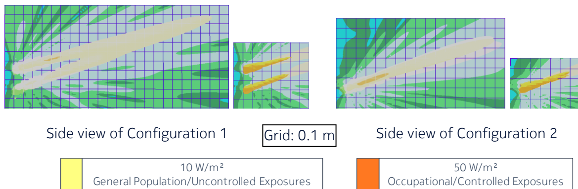
Figure 9 – Power density from AWEWA/B (or FA3WA) for the time-averaged maximum transmitted power of 1.42 W (corresponding to the time-averaged maximum EIRP of 55.52 dBm) and the beam oriented in azimuth = 0° & elevation = -20°, together with the power density from FA3UB (or AWEUC/D) for the time-averaged maximum transmitted power of 0.76 W (corresponding to the time-averaged maximum EIRP of 55.52 dBm) and the beam oriented in azimuth = 0° & elevation = -15°
