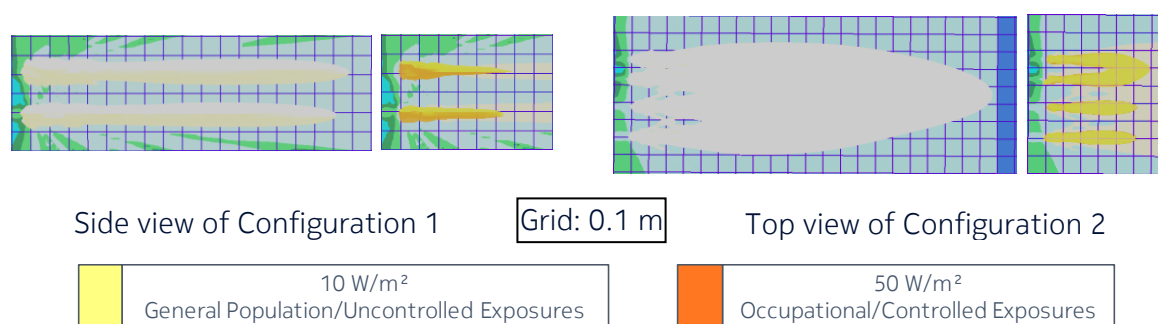
Figure 3 – Power density from AWEWA/B (or FA3WA) for the time-averaged maximum transmitted power of 1.42 W (corresponding to the time-averaged maximum EIRP of 55.52 dBm) and the beam oriented in azimuth = 0° & elevation = 0°, together with the power density from FA3UB (or AWEUC/D) for the time-averaged maximum transmitted power of 0.76 W (corresponding to the time-averaged maximum EIRP of 55.52 dBm) and the beam oriented in azimuth = 0° & elevation = 0°
