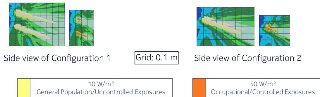
Figure 8 – Power density from AWEWA/B (or FA3WA) for the actual maximum transmitted power of 0.4 W (corresponding to the actual EIRP threshold of 49.52 dBm) and the beam oriented in azimuth = 0° & elevation = +20°, together with the power density from FA3UB (or AWEUC/D) for the actual maximum transmitted power of 0.2 W (corresponding to the actual EIRP threshold of 49.52 dBm) and the beam oriented in azimuth = 0° & elevation = +15°
