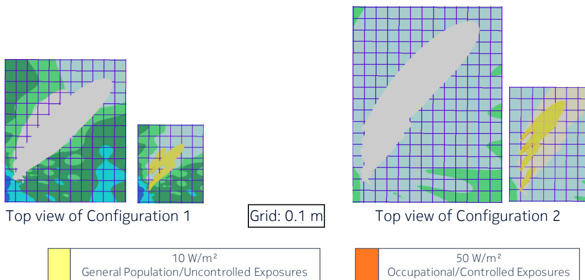
Figure 5 – Power density from AWEWA/B (or FA3WA) for the time-averaged maximum transmitted power of 1.42 W (corresponding to the time-averaged maximum EIRP of 55.52 dBm) and the beam oriented in azimuth = +60° & elevation = 0°, together with the power density from FA3UB (or AWEUC/D) for the time-averaged maximum transmitted power of 0.76 W (corresponding to the time-averaged maximum EIRP of 55.52 dBm) and the beam oriented in azimuth = +45° & elevation = 0°
