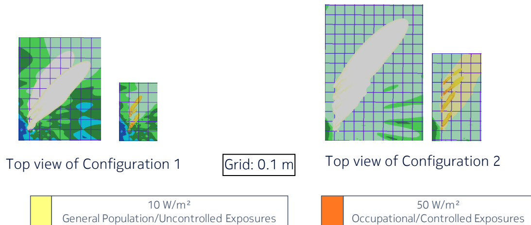
Figure 6 – Power density from AWEWA/B (or FA3WA) for the actual maximum transmitted power of 1.2 W (corresponding to the actual EIRP threshold of 49.52 dBm) and the beam oriented in azimuth = +60° & elevation = 0°, together with the power density from FA3UB (or AWEUC/D) for the actual maximum transmitted power of 0.37 W (corresponding to the actual EIRP threshold of 49.52 dBm) and the beam oriented in azimuth = +45° & elevation = 0°
