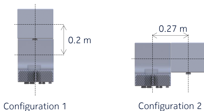
Figure 2 – Co-location configurations of AWEWA/B + FA3UB or AWEUC/D + FA3WA used for the RF exposure assessment to provide conservative compliance distances
