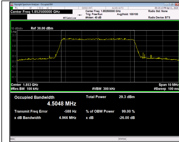
Band2-5MHz-64QAM-18625-25RB#0-PASS
