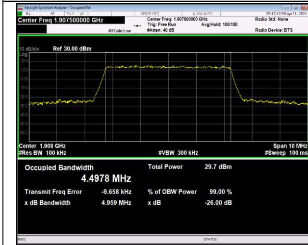
Band2-5MHz-64QAM-19175-25RB#0-PASS
