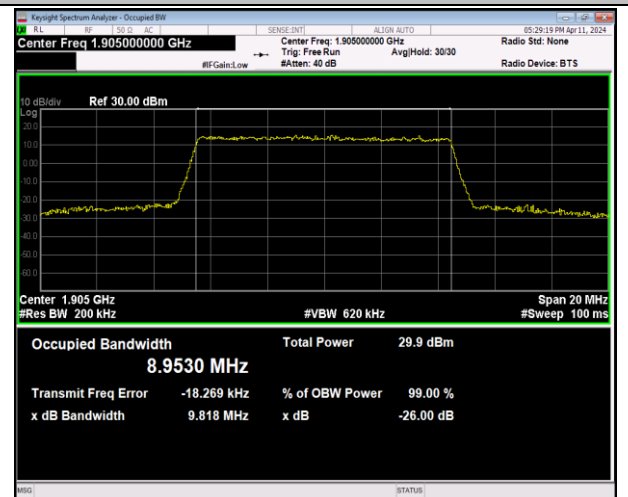
Band2-10MHz-64QAM-19150-50RB#0-PASS
