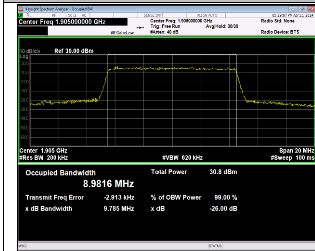
Band2-10MHz-16QAM-19150-50RB#0-PASS
