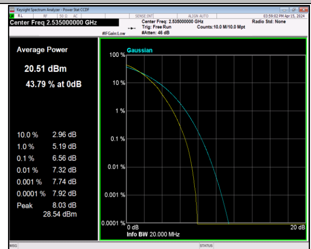
Band7-20MHz-64QAM-21100-100RB#0-PASS
