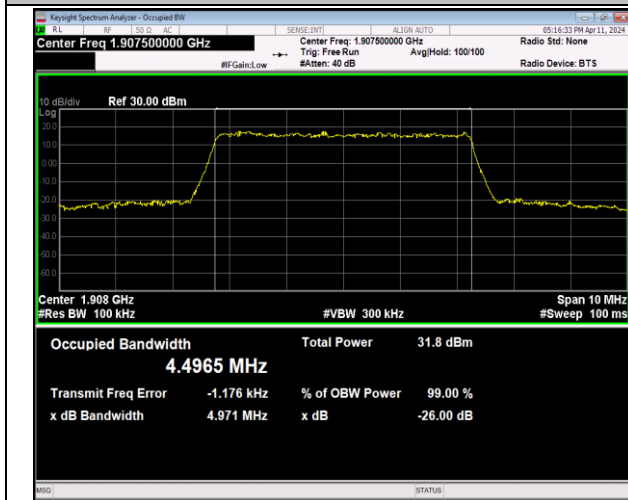
Band2-5MHz-QPSK-19175-25RB#0-PASS
