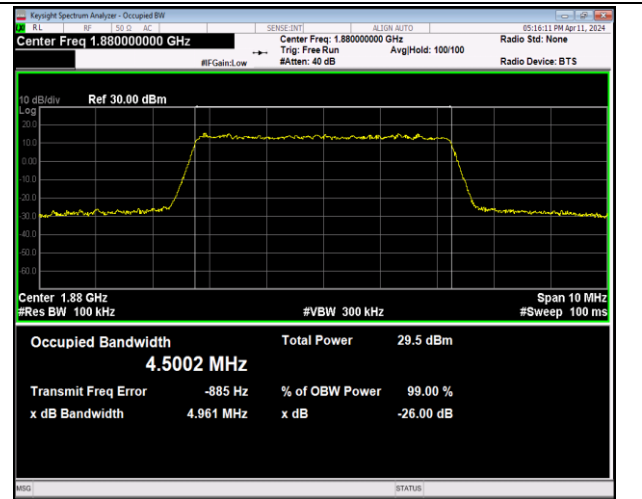
Band2-5MHz-64QAM-18900-25RB#0-PASS
