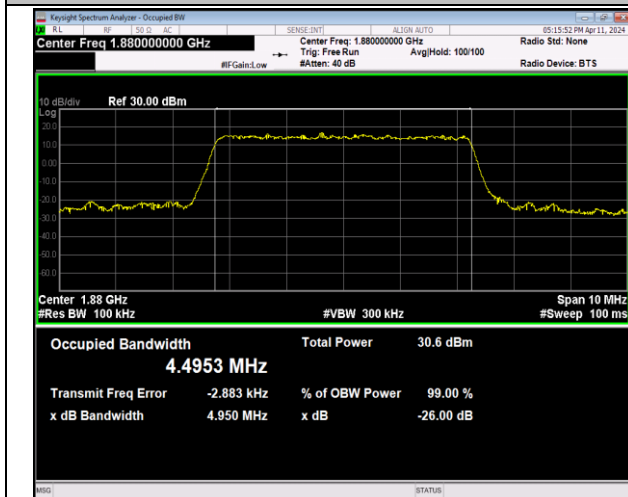
Band2-5MHz-16QAM-18900-25RB#0-PASS
