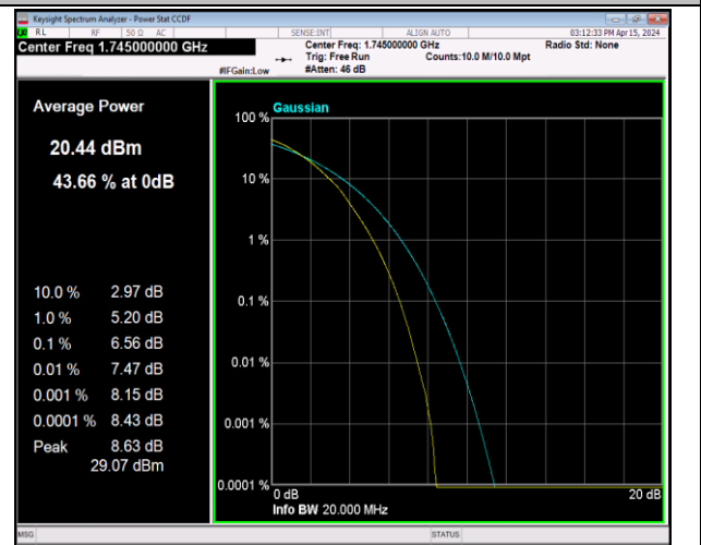
Band66-20MHz-64QAM-132322-100RB#0-PASS
