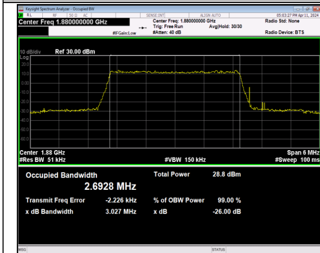
Band2-3MHz-64QAM-18900-15RB#0-PASS
