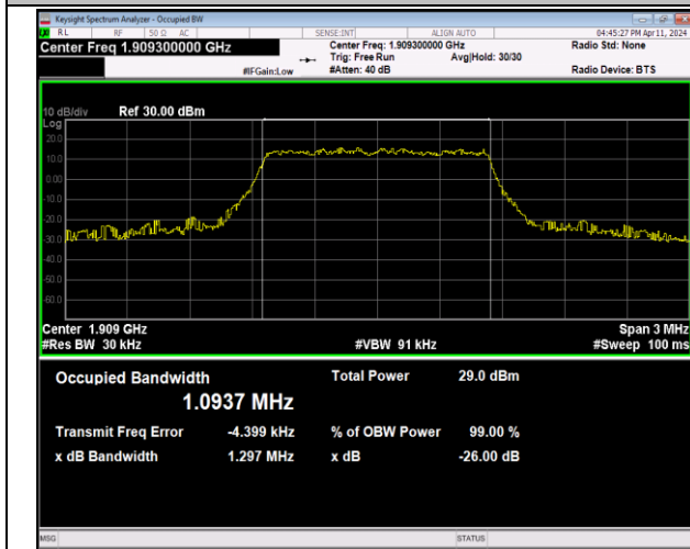
Band2-1.4MHz-64QAM-19193-6RB#0-PASS
