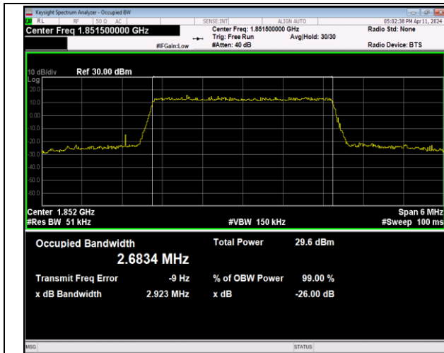
Band2-3MHz-16QAM-18615-15RB#0-PASS
