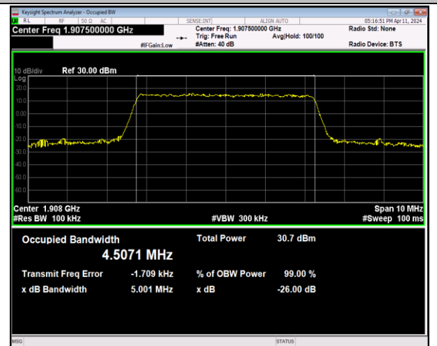
Band2-5MHz-16QAM-19175-25RB#0-PASS
