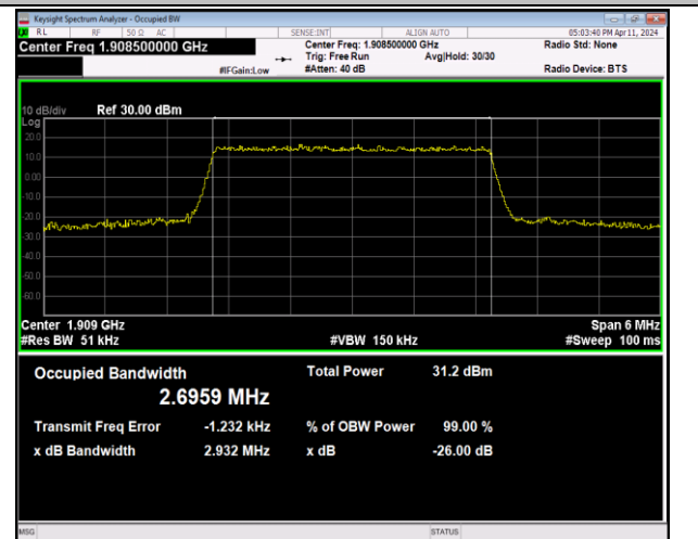
Band2-3MHz-QPSK-19185-15RB#0-PASS
