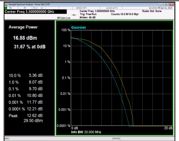
42(3450-3550)-20MHz-16QAM-42590-100RB#0-PASS
