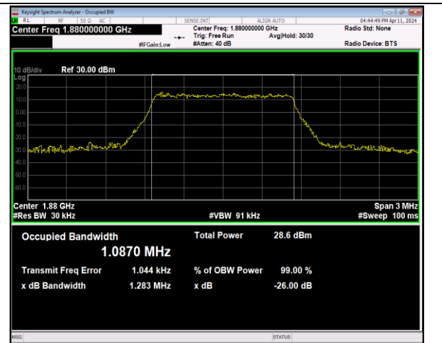
Band2-1.4MHz-64QAM-18900-6RB#0-PASS
