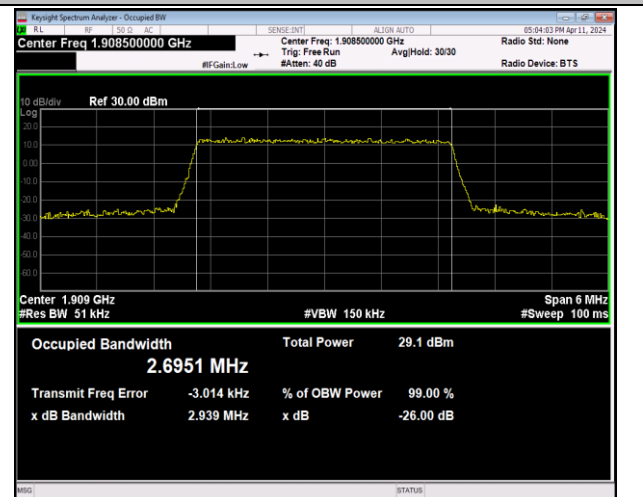
Band2-3MHz-64QAM-19185-15RB#0-PASS
