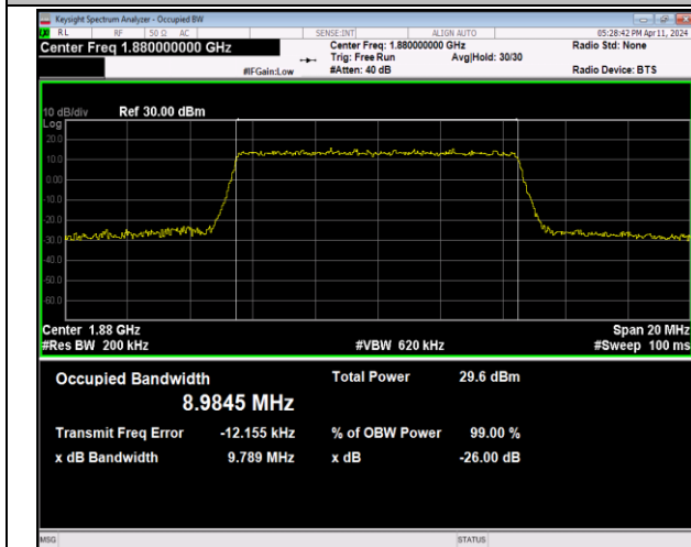
Band2-10MHz-64QAM-18900-50RB#0-PASS
