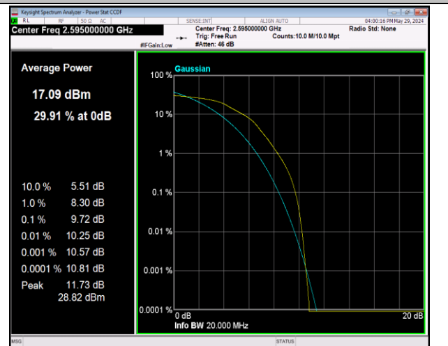
Band38-20MHz-16QAM-38000-100RB#0-PASS
