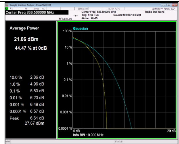
Band5-10MHz-16QAM-20525-50RB#0-PASS
