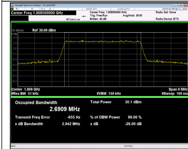
Band2-3MHz-16QAM-19185-15RB#0-PASS
