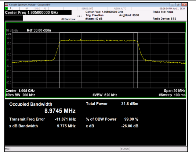
Band2-10MHz-QPSK-19150-50RB#0-PASS
