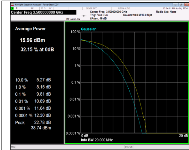
42(3450-3550)-20MHz-64QAM-42590-100RB#0-PASS
