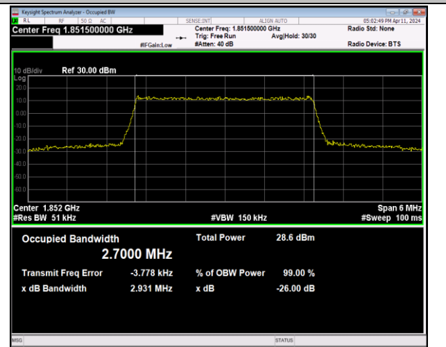
Band2-3MHz-64QAM-18615-15RB#0-PASS
