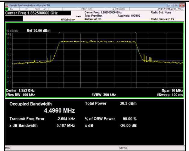
Band2-5MHz-16QAM-18625-25RB#0-PASS
