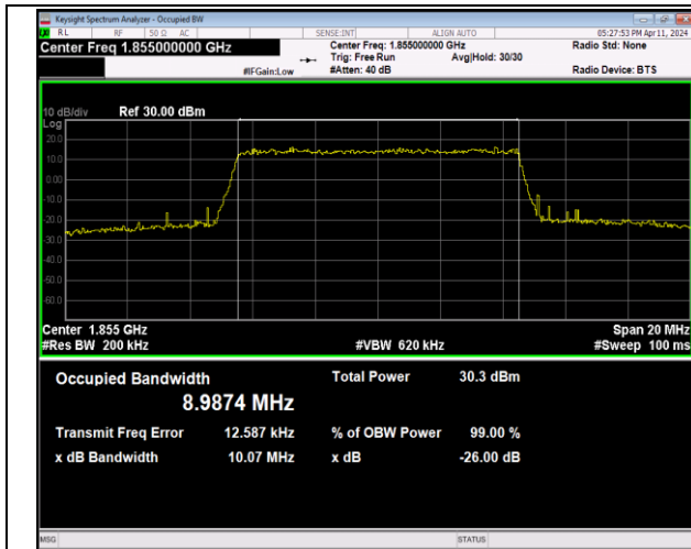
Band2-10MHz-16QAM-18650-50RB#0-PASS
