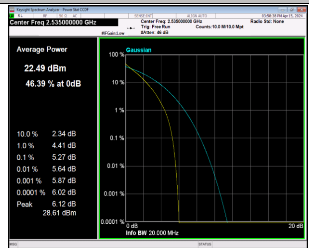
Band7-20MHz-QPSK-21100-100RB#0-PASS
