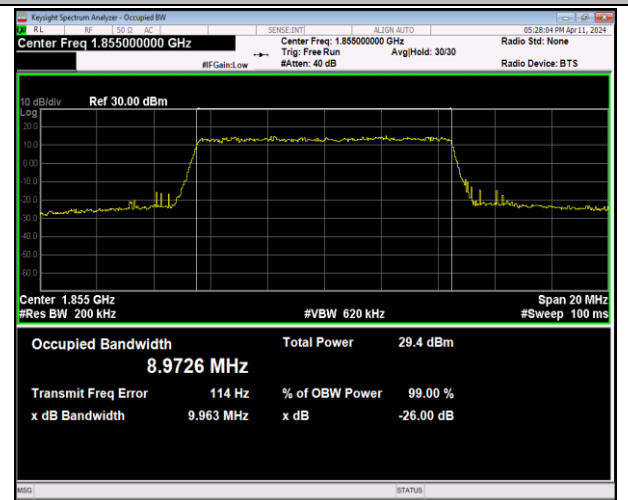
Band2-10MHz-64QAM-18650-50RB#0-PASS
