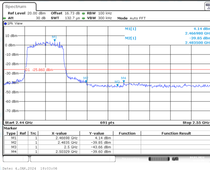
11AX20-CDD_Ant2_High_2462
