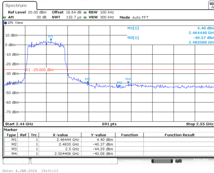
11AX20-CDD_Ant2_High_2462
