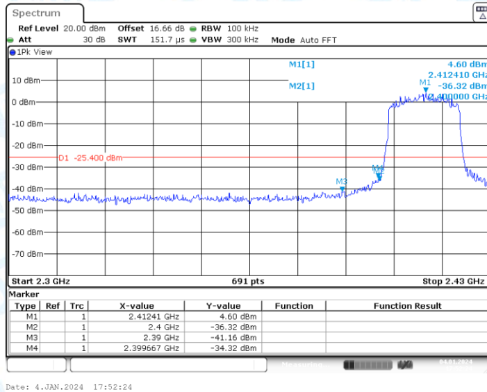
11AX20-CDD_Ant2_Low_2412
