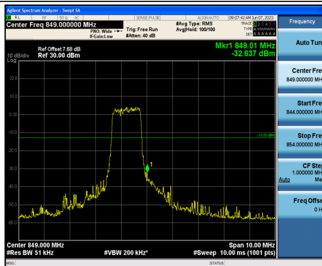
Band5-5MHz-16QAM-20625-6-0-High--32.64-PASS
