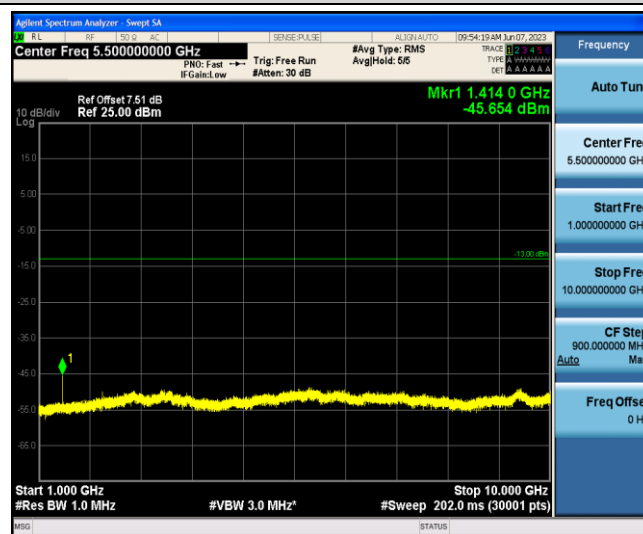
Band12-1.4MHz-16QAM-23095-1-0-Low-1000-10000--45.65-PASS
