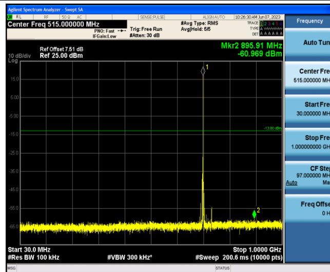
Band12-3MHz-16QAM-23095-1-0-Low-30-1000--60.97-PASS
