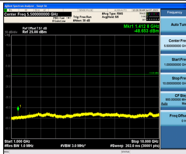
Band12-3MHz-16QAM-23095-1-0-Low-1000-10000--48.65-PASS
