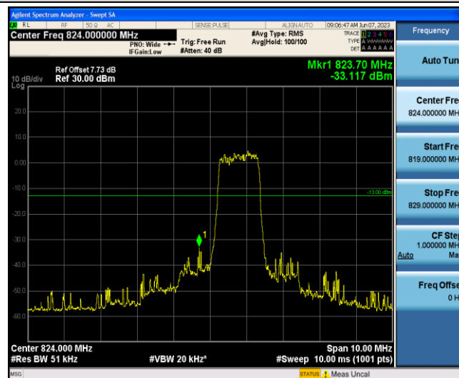
Band5-5MHz-QPSK-20425-6-0-Low--33.12-PASS
