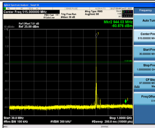
Band12-3MHz-16QAM-23165-1-0-Low-30-1000--60.88-PASS
