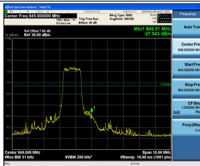
Band5-10MHz-16QAM-20600-6-0-High--37.54-PASS
