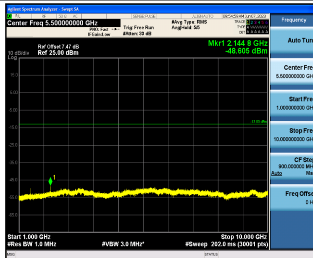
Band12-1.4MHz-16QAM-23173-1-0-Low-1000-10000--48.61-PASS
