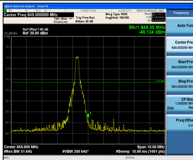
Band5-5MHz-16QAM-20625-1-5-High--46.12-PASS
