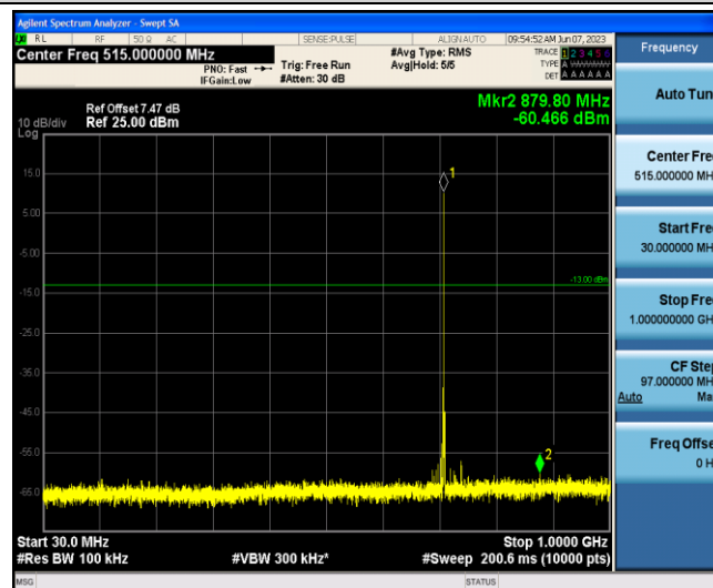
Band12-1.4MHz-16QAM-23173-1-0-Low-30-1000--60.47-PASS
