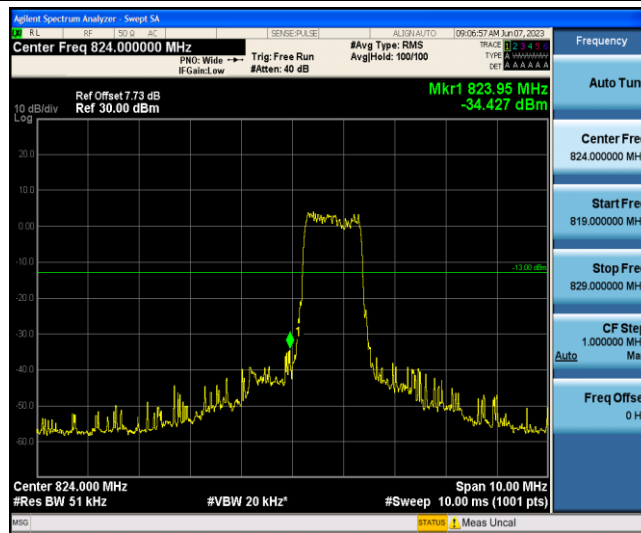
Band5-5MHz-16QAM-20425-6-0-Low--34.43-PASS
