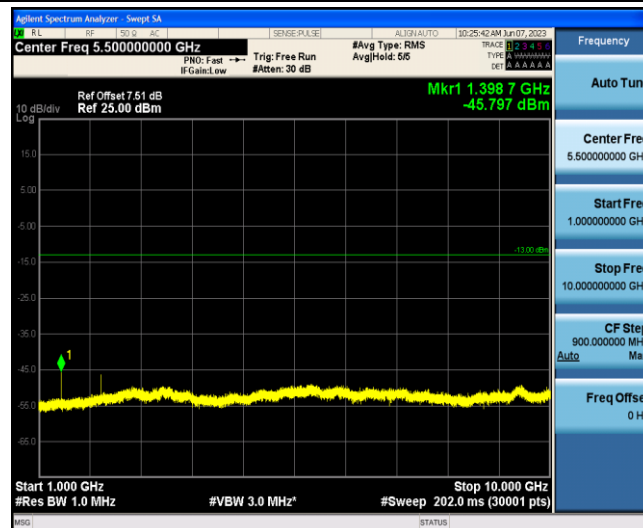
Band12-3MHz-QPSK-23025-1-0-Low-1000-10000--45.8-PASS
