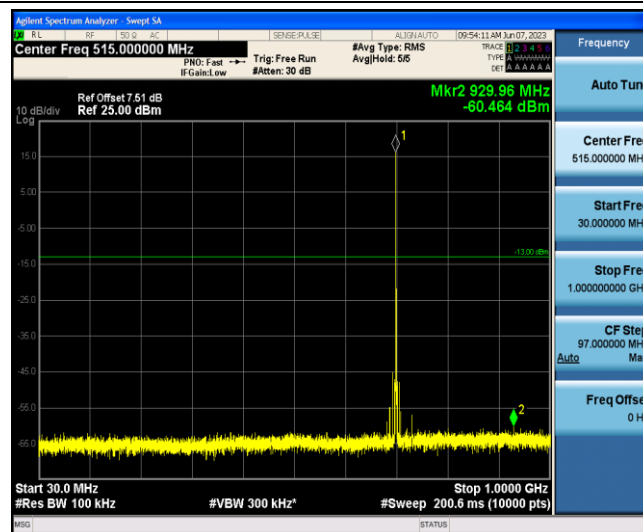
Band12-1.4MHz-16QAM-23095-1-0-Low-30-1000--60.46-PASS
