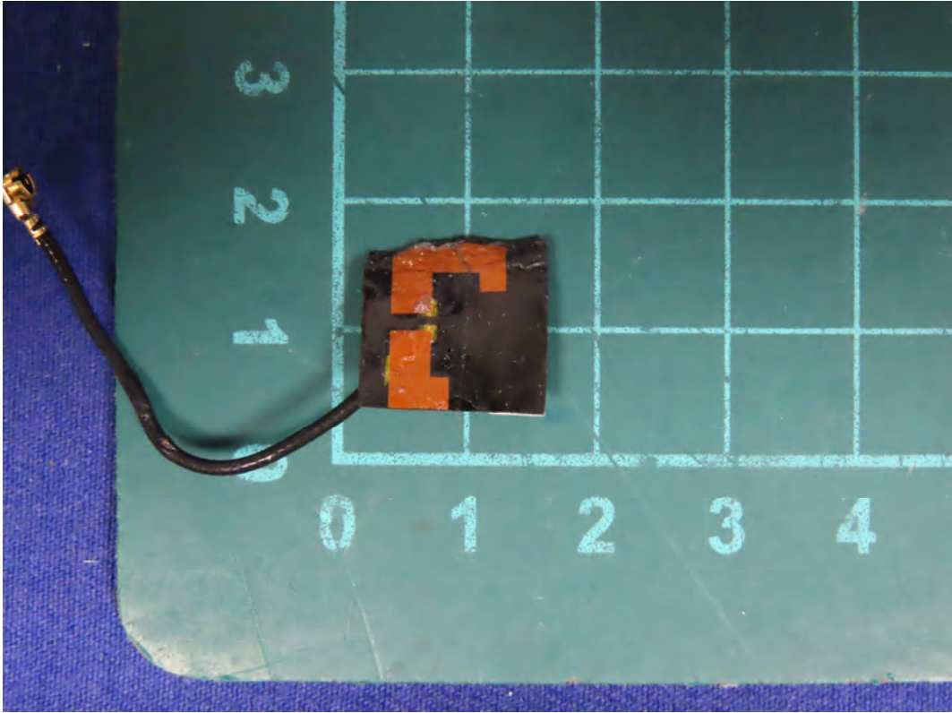
(26) EUT Photo_ RF Antenna
