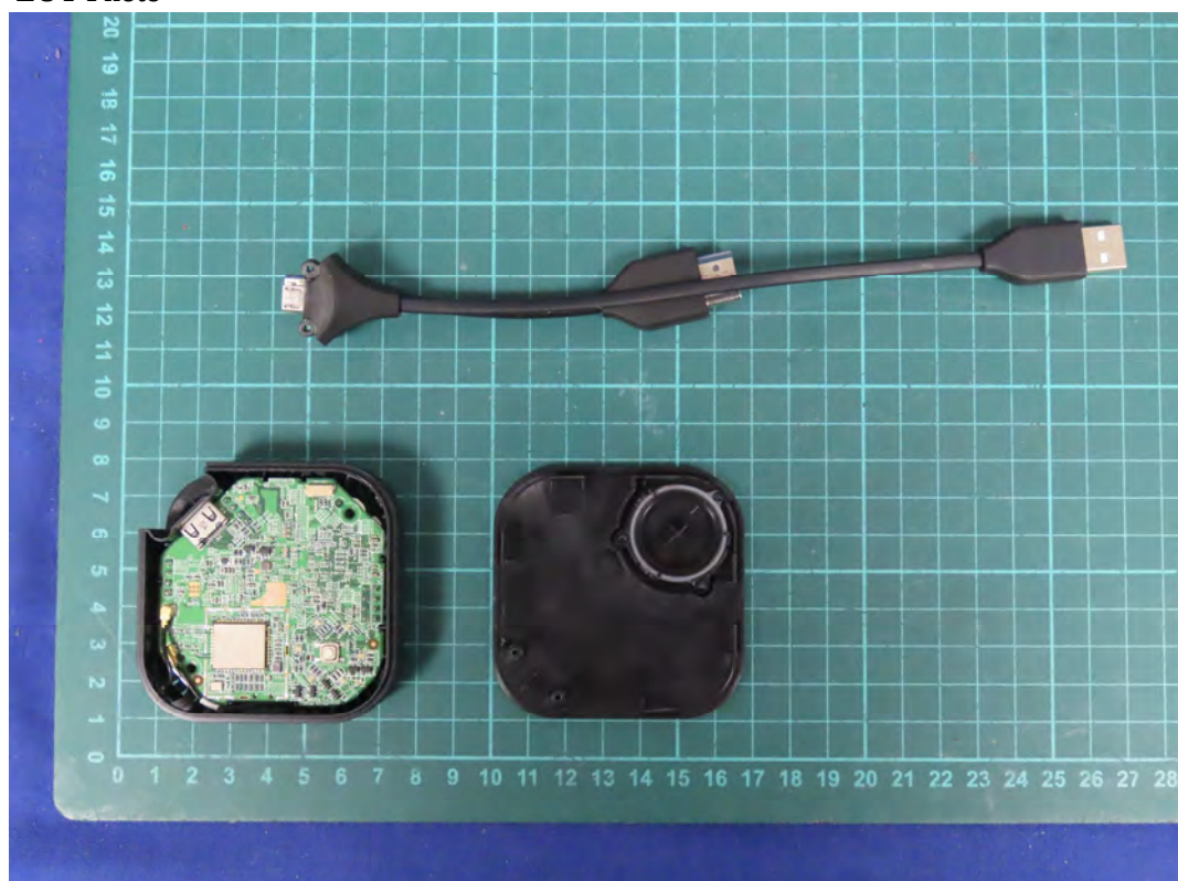
(7) EUT Photo
