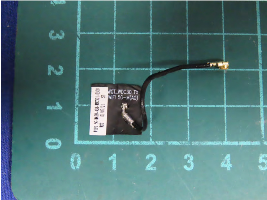
(25) EUT Photo_ RF Antenna
