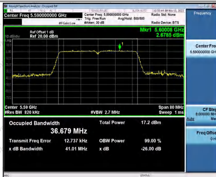
11AC40SISO_Ant2_5590
