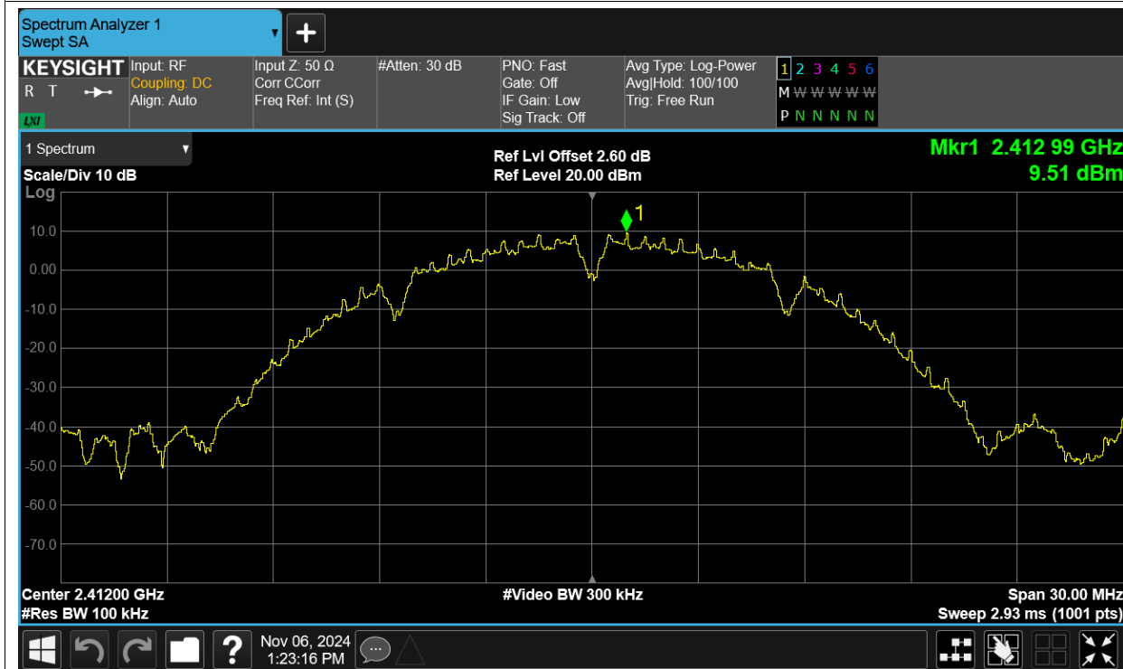
Band Edge NVNT b 2412MHz Ant14 Emission
