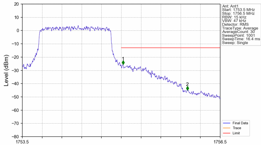
Band4_1.4MHz_16QAM_HCH_1754.3MHz_RB_6_0_NTNV
