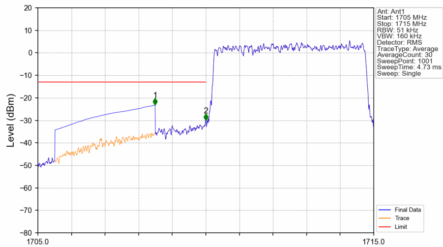
Band4_5MHz_QPSK_LCH_1712.5MHz_RB_25_0_NTNV
