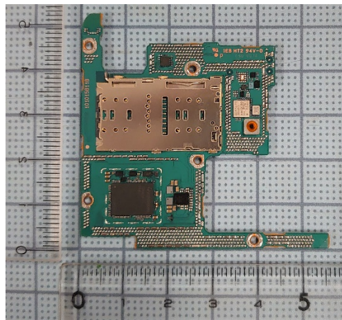
Internal Main-PWB Rear without Shield case (Front-side)
