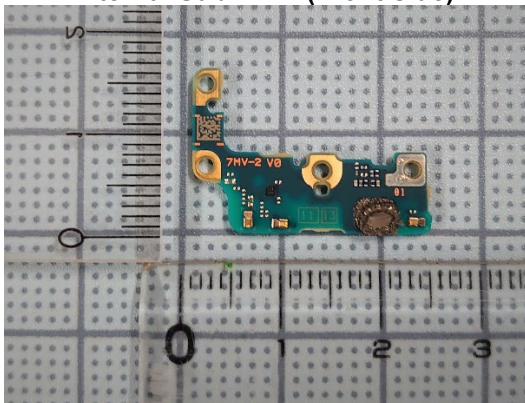
Internal Sub-PWB (Front-side)
