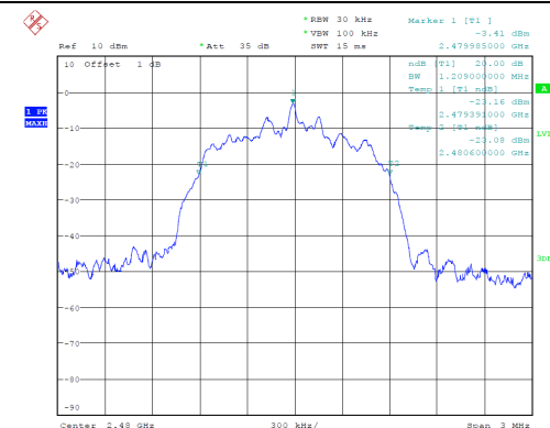
8-DPSK Mode 2480MHz
