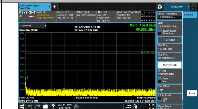
Band12-5MHz-QPSK-23035-1RB#0-0.15~30-PASS
