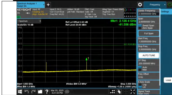
Band12-3MHz-QPSK-23095-1RB#14-1000~3000-PASS
