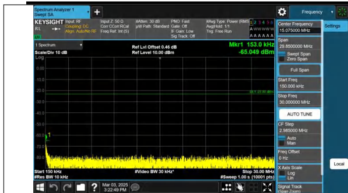
Band12-3MHz-QPSK-23165-1RB#14-0.15~30-PASS
