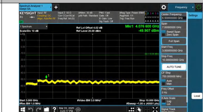
Band12-3MHz-QPSK-23165-1RB#14-3000~10000-PASS
