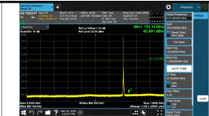
Band12-3MHz-QPSK-23165-1RB#14-30~1000-PASS
