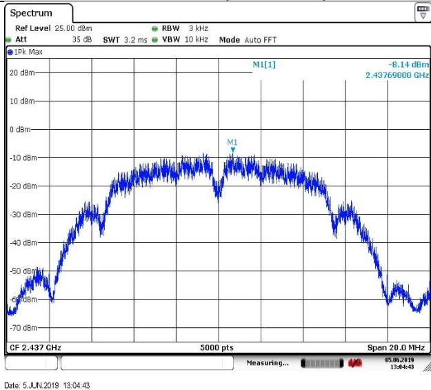
Channel 06 (2437MHz)
