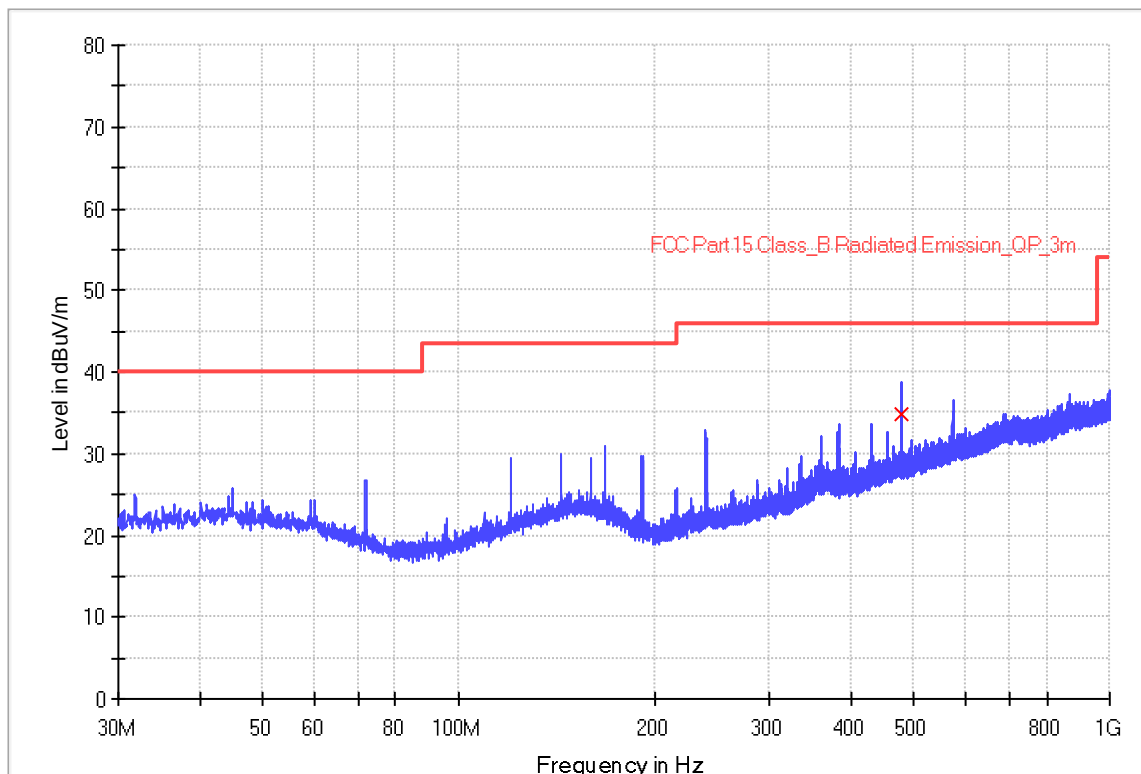
PE_VULB9168_pre_Cont_30-1000
