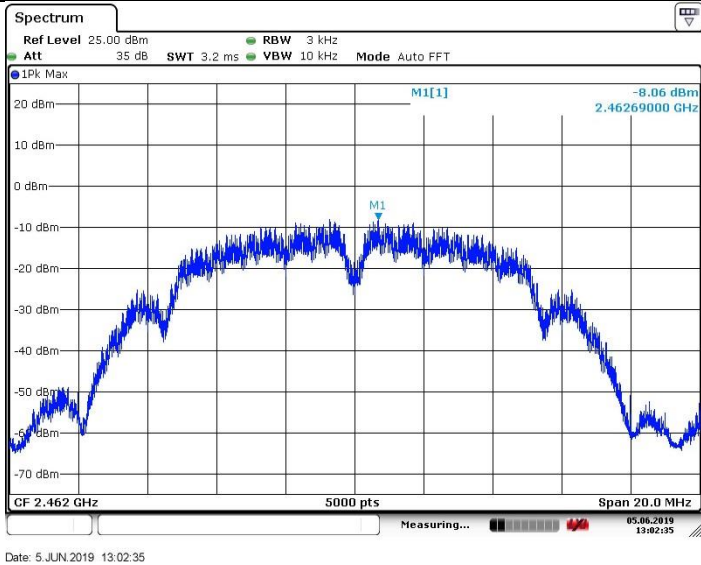
Channel 11 (2462MHz)
