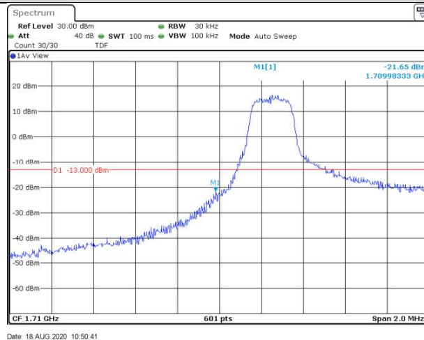
Band4-1.4MHz-16QAM-19957-1RB#5
