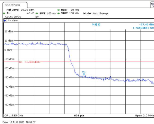
Band4-1.4MHz-16QAM-19957-1RB#0
