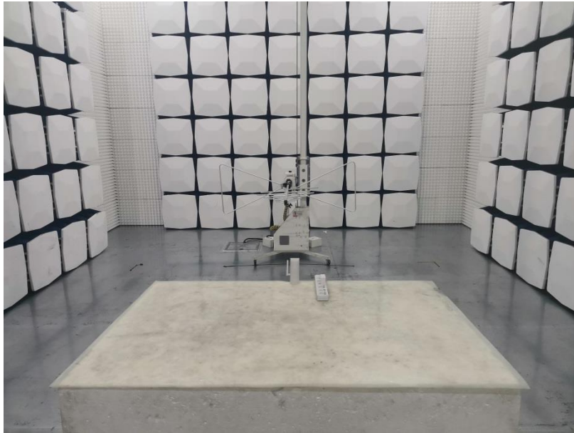
Spurious Emission (Below 1GHz)
