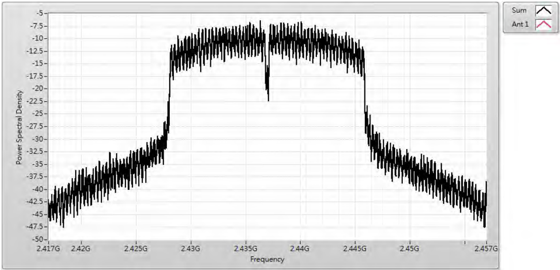
IEEE 802.11n (20MHz) - Channel 6 (2437MHz)
