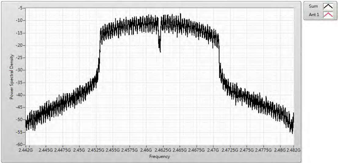
IEEE 802.11n (20MHz) - Channel 11 (2462MHz)
