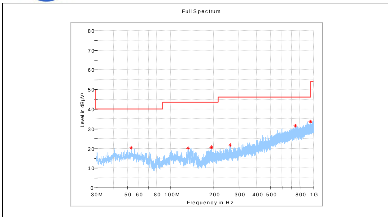
(802.11ac_5290MHz, Antenna Vertical, 30MHz to 1GHz)
