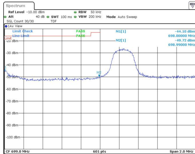
Band12-3MHz-QPSK-23025-15RB#0
