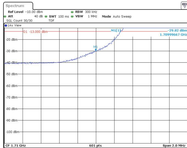
Band4-15MHz-QPSK-20025-1RB#74
