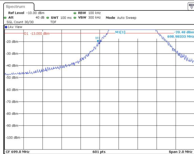
Band12-5MHz-QPSK-23035-1RB#24
