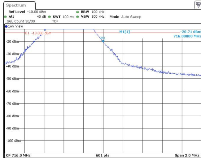
Band12-5MHz-QPSK-23155-25RB#0
