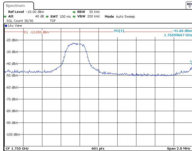
Band4-3MHz-QPSK-20385-1RB#14
