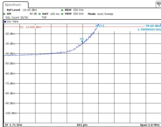
Band4-10MHz-QPSK-20000-1RB#49
