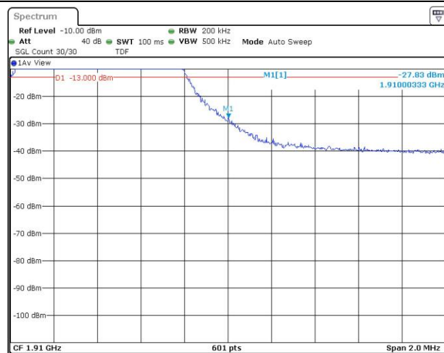
Band2-10MHz-16QAM-19150-25RB#0
