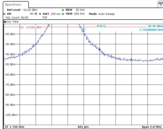
Band4-3MHz-16QAM-20385-15RB#0
