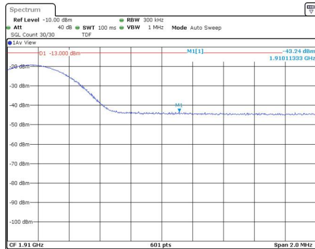
Band2-15MHz-QPSK-19125-1RB#74
