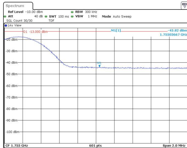
Band4-15MHz-QPSK-20325-1RB#74
