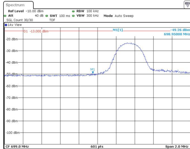
Band12-5MHz-QPSK-23035-25RB#0
