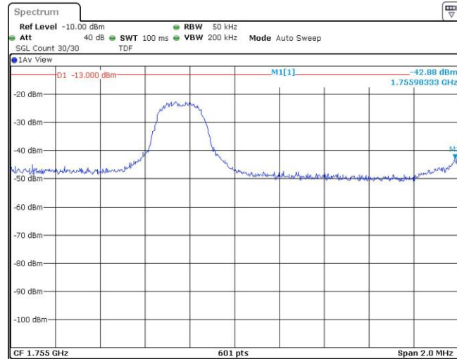
Band4-3MHz-16QAM-20385-1RB#14
