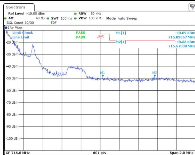
Band12-1.4MHz-16QAM-23173-1RB#5
