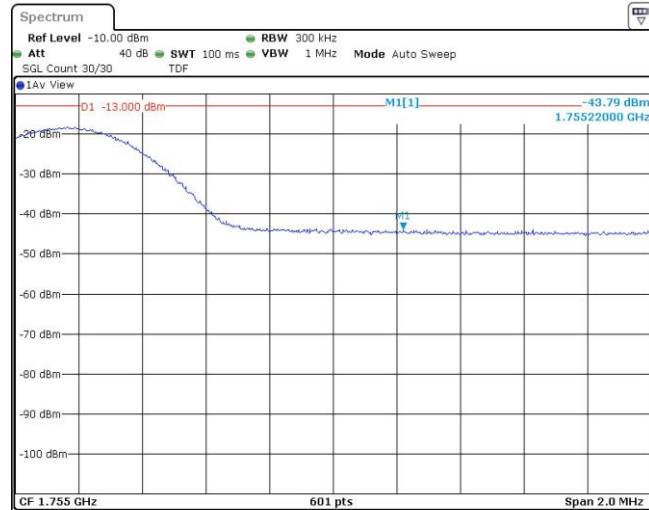
Band4-15MHz-16QAM-20325-1RB#74
