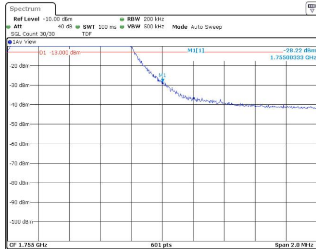
Band4-10MHz-QPSK-20350-50RB#0
