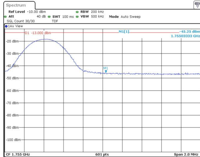
Band4-10MHz-QPSK-20350-1RB#49
