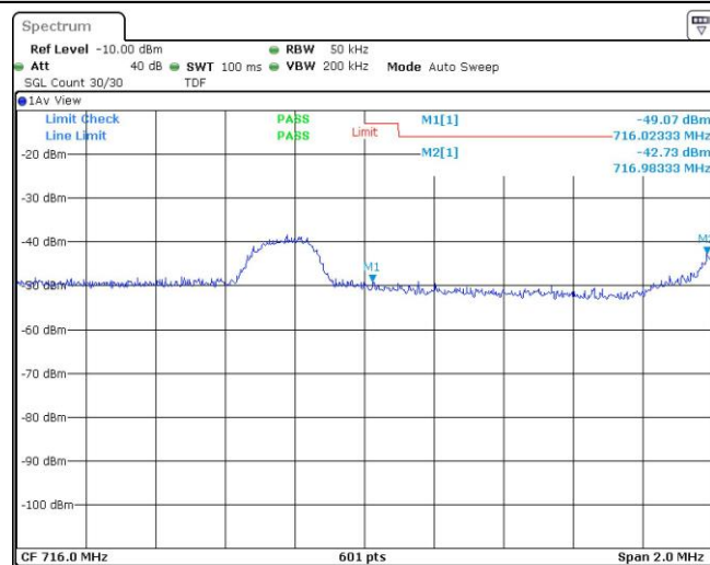
Band12-3MHz-16QAM-23165-1RB#14
