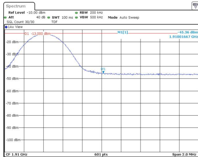
Band2-10MHz-16QAM-19150-1RB#49
