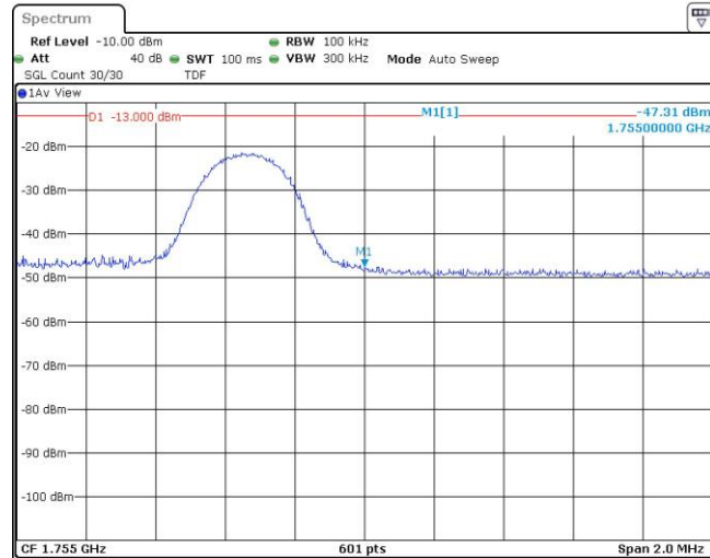
Band4-5MHz-16QAM-20375-1RB#24
