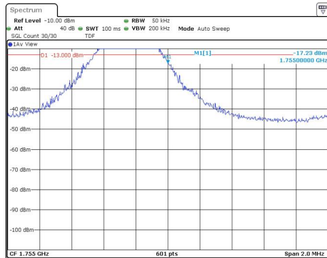
Band4-3MHz-QPSK-20385-15RB#0
