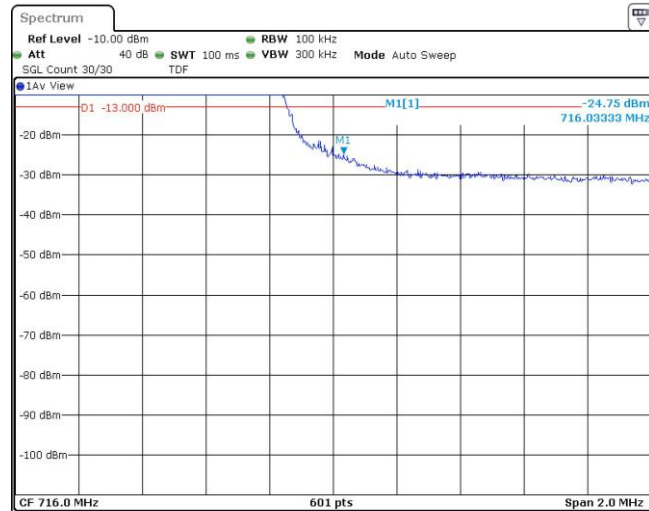
Band12-5MHz-16QAM-23035-1RB#0
