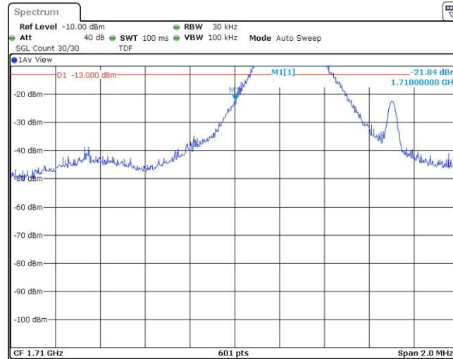
Band4-1.4MHz-16QAM-19957-1RB#5
