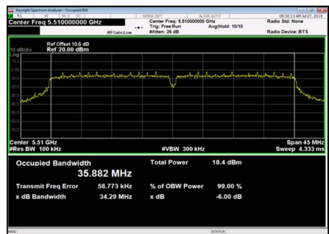
U-NII-2c 6dB Bandwidth-802.11n(40MHz) ,5510MHz
