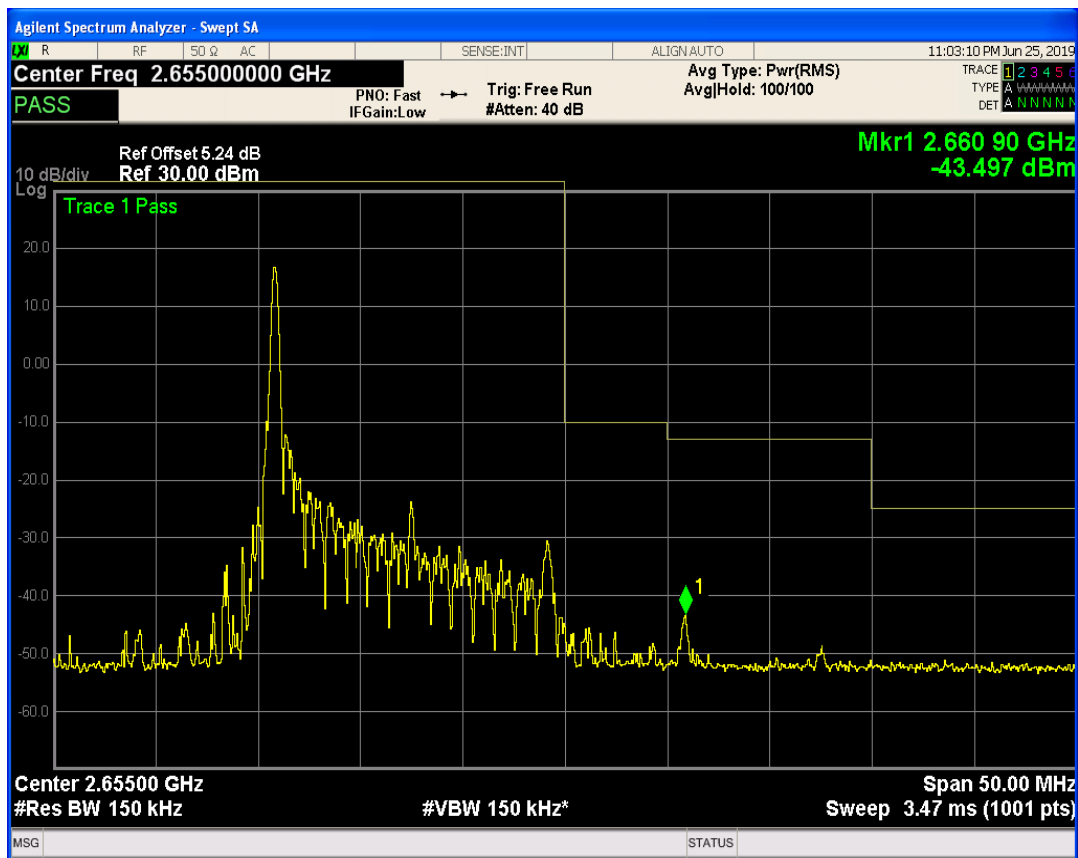
LTE Band41 QAM16 BW=15MHz Channel=41165 RB Size=1 Position=#Max
