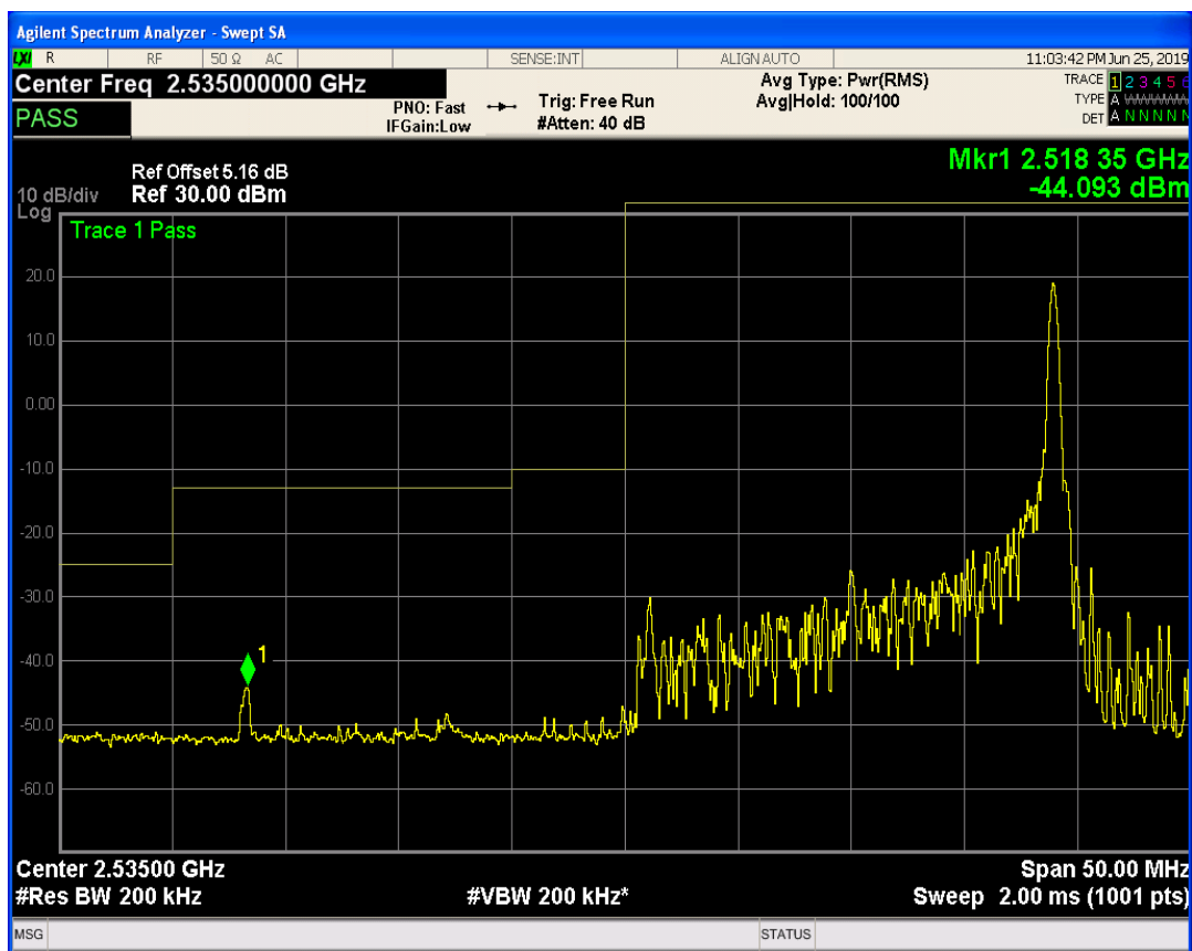
LTE Band41 QAM16 BW=20MHz Channel=40140 RB Size=50 Position=#Max
