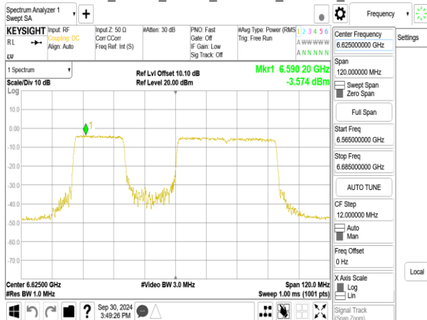
802.11be_80MHz_Chain0_6625MHz_484+242_MRU2
