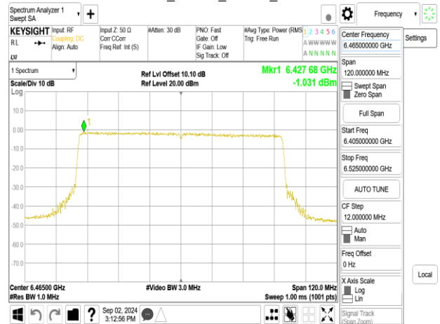
802.11be_80MHz_Chain0_6465MHz_RU484+242_Punc20
