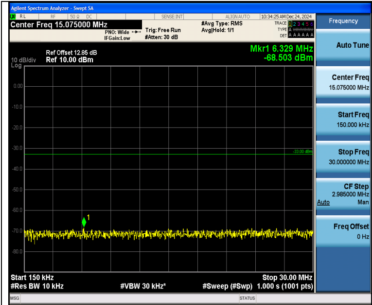
Band2_10MHz_QPSK_18900_50RB#0_0.15~30_0.15~30
