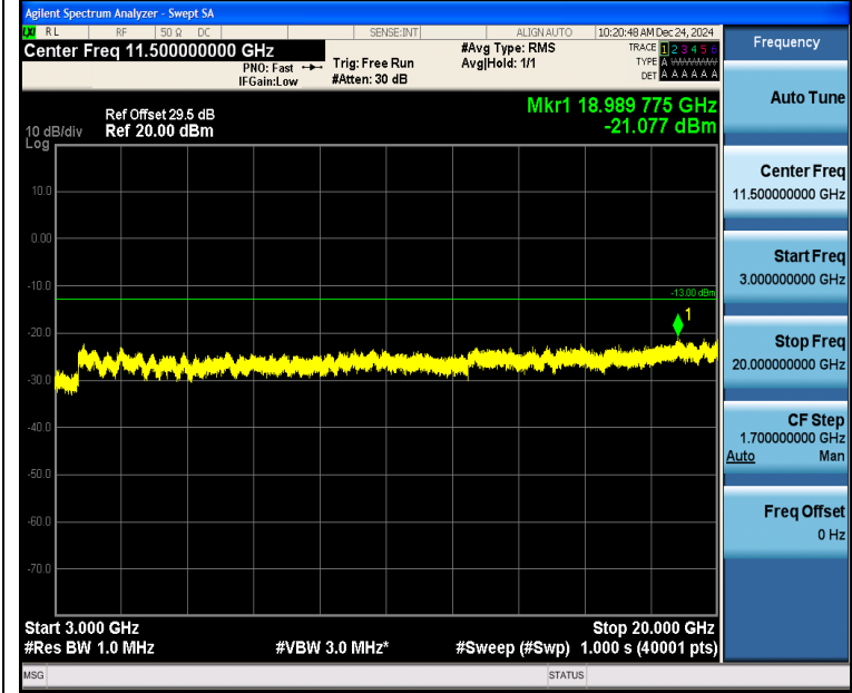
Band2_10MHz_QPSK_18650_1RB#0_3000~20000_3000~20000
