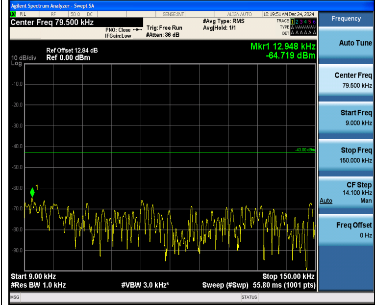
Band2_10MHz_QPSK_18650_1RB#0_0.009~0.15_0.009~0.15
