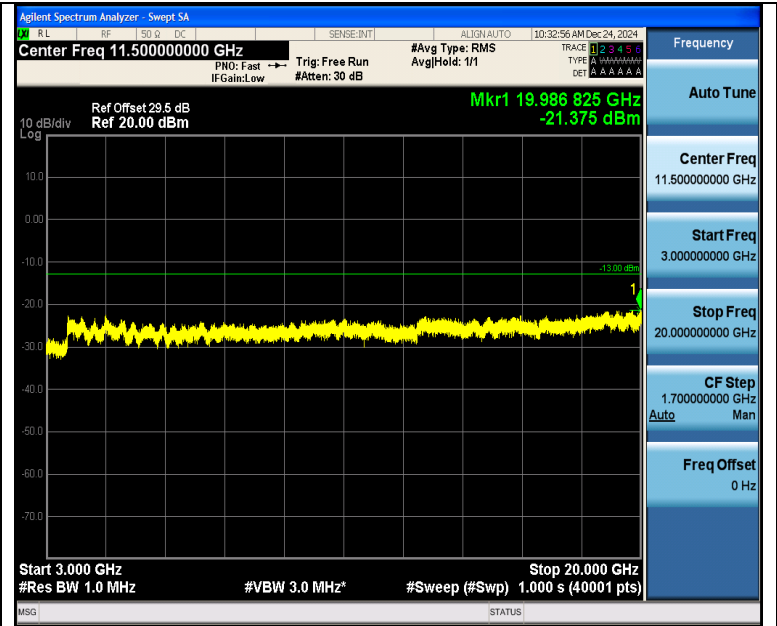
Band2_10MHz_16QAM_19150_1RB#49_3000~20000_3000~20000
