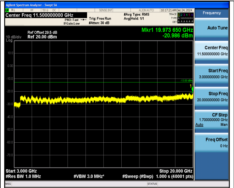
Band2_5MHz_16QAM_19175_25RB#0_3000~20000_3000~20000
