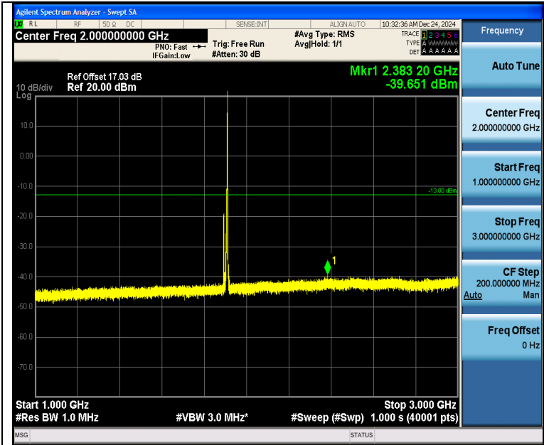
Band2_10MHz_16QAM_19150_1RB#49_1000~3000_1000~3000
