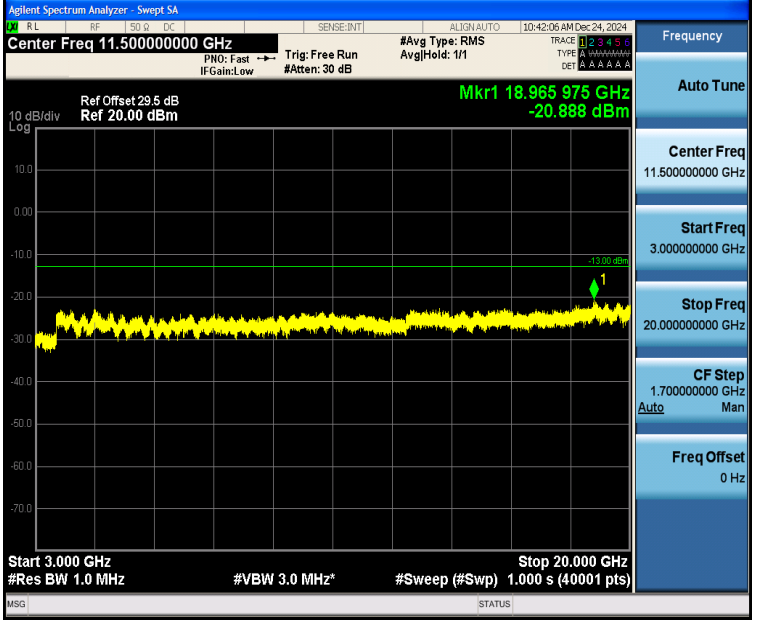
Band2_15MHz_QPSK_18675_1RB#74_3000~20000_3000~20000
