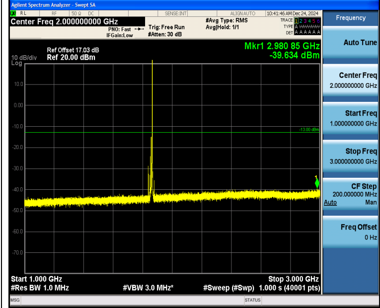
Band2_15MHz_QPSK_18675_1RB#74_1000~3000_1000~3000
