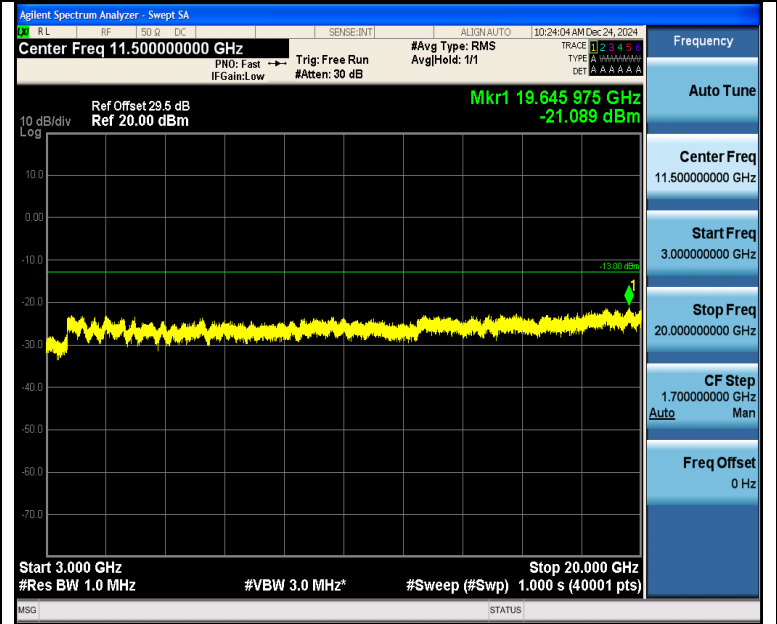
Band2_10MHz_16QAM_18650_1RB#49_3000~20000_3000~20000
