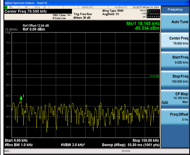
Band2_10MHz_16QAM_18650_1RB#0_0.009~0.15_0.009~0.15
