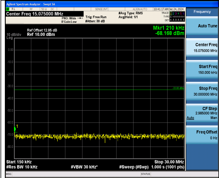
Band2_15MHz_QPSK_18675_1RB#74_0.15~30_0.15~30
