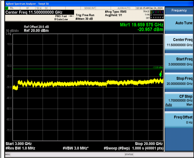
Band2_5MHz_QPSK_19175_25RB#0_3000~20000_3000~20000
