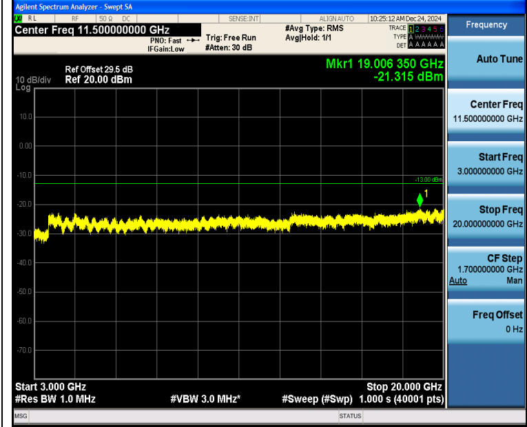
Band2_10MHz_QPSK_18900_1RB#0_3000~20000_3000~20000
