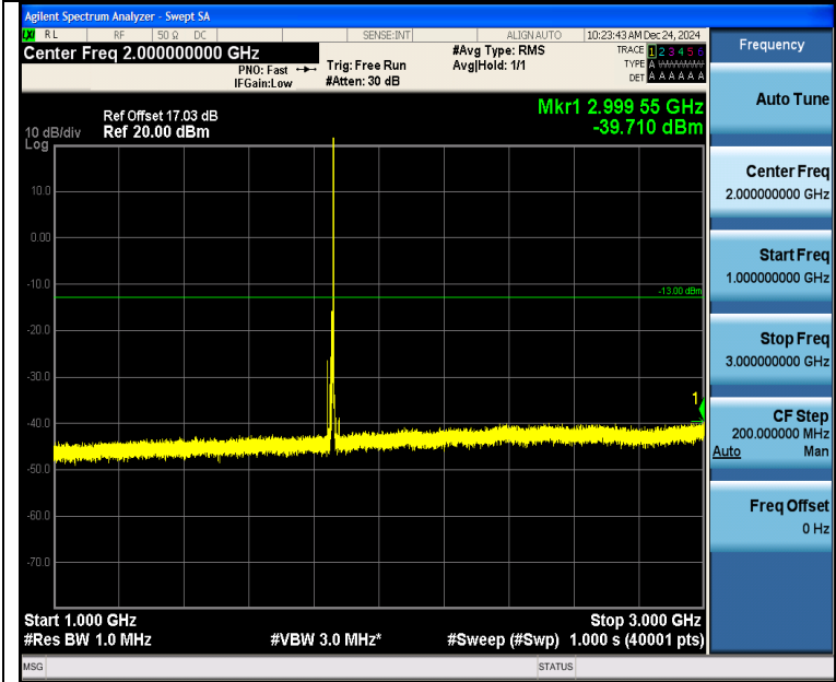
Band2_10MHz_16QAM_18650_1RB#49_1000~3000_1000~3000
