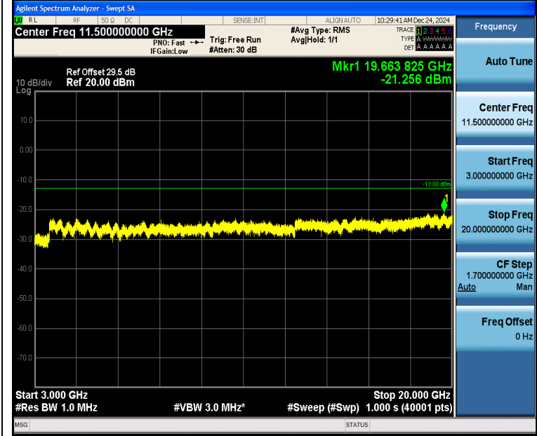
Band2_10MHz_QPSK_19150_1RB#0_3000~20000_3000~20000
