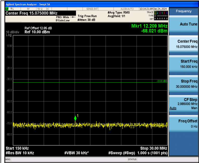
Band2_5MHz_16QAM_19175_1RB#24_0.15~30_0.15~30
