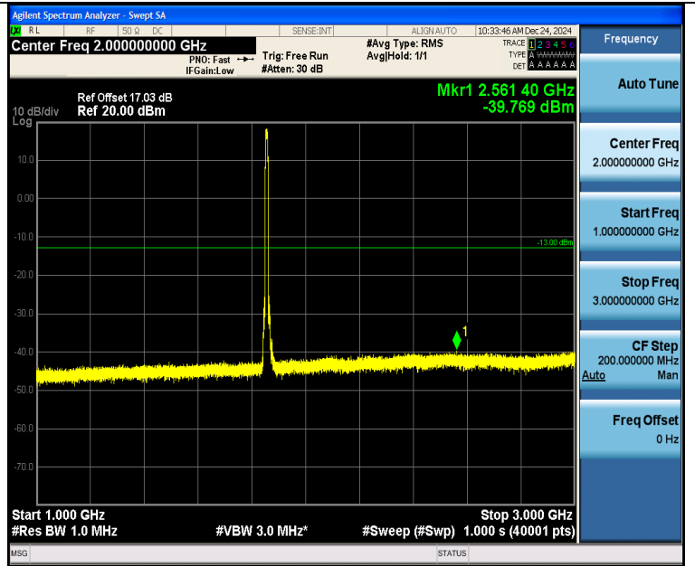
Band2_10MHz_QPSK_18650_50RB#0_1000~3000_1000~3000
