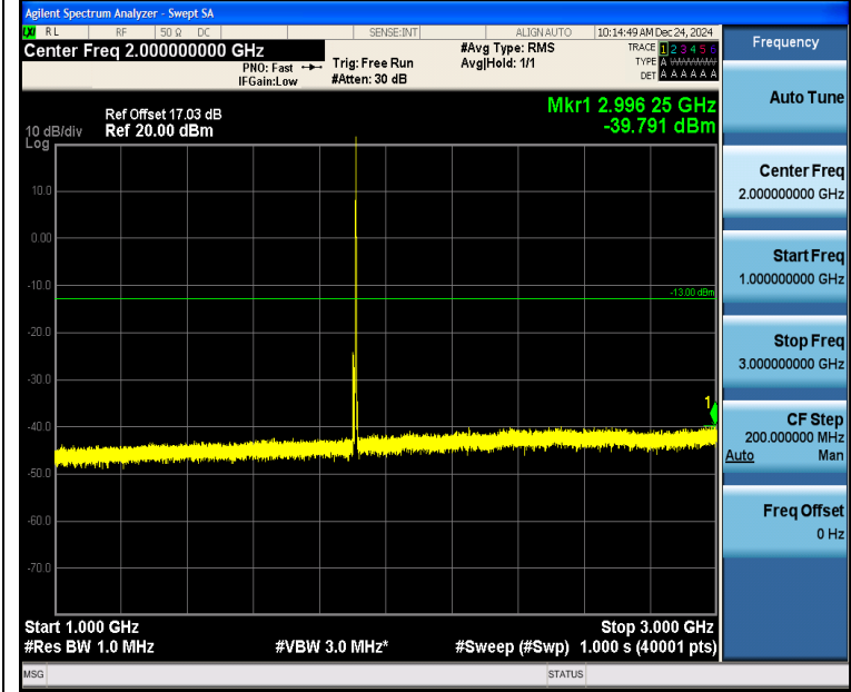
Band2_5MHz_16QAM_19175_1RB#24_1000~3000_1000~3000
