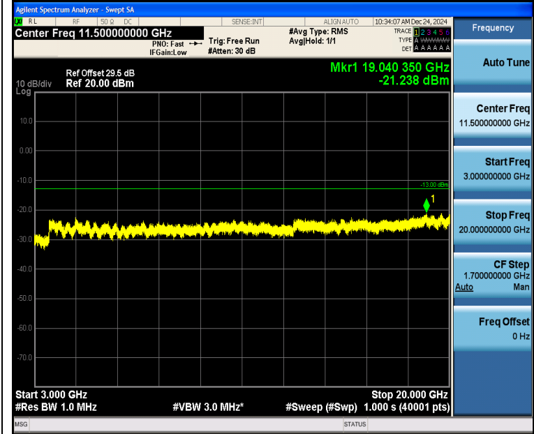
Band2_10MHz_QPSK_18650_50RB#0_3000~20000_3000~20000
