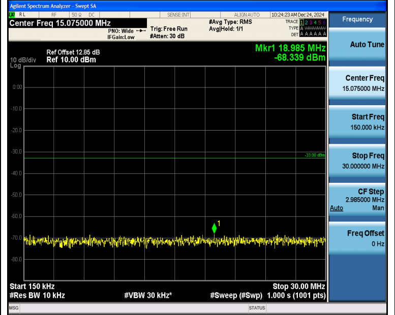
Band2_10MHz_QPSK_18900_1RB#0_0.15~30_0.15~30
