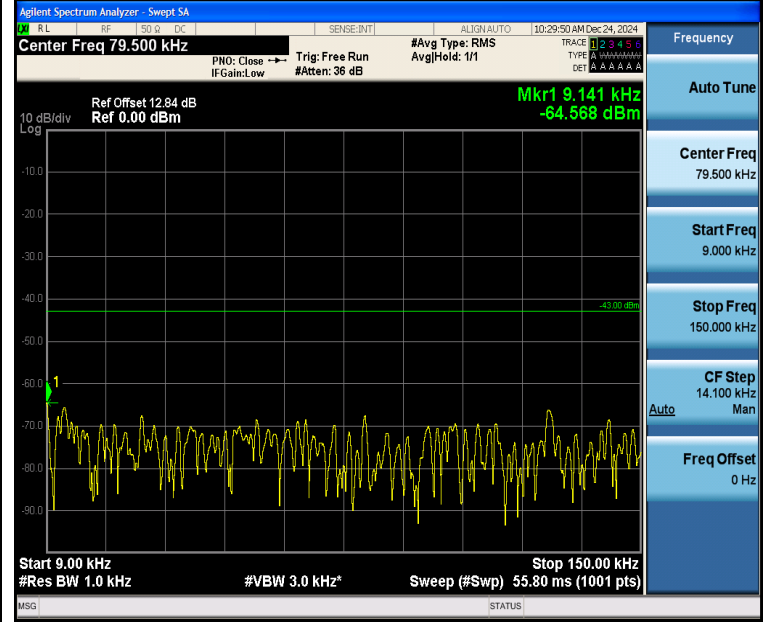
Band2_10MHz_16QAM_19150_1RB#0_0.009~0.15_0.009~0.15
