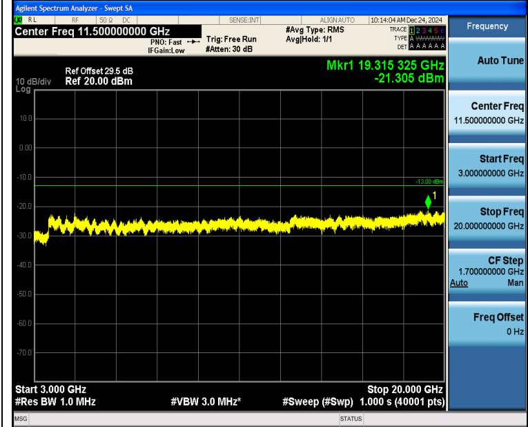
Band2_5MHz_QPSK_19175_1RB#24_3000~20000_3000~20000
