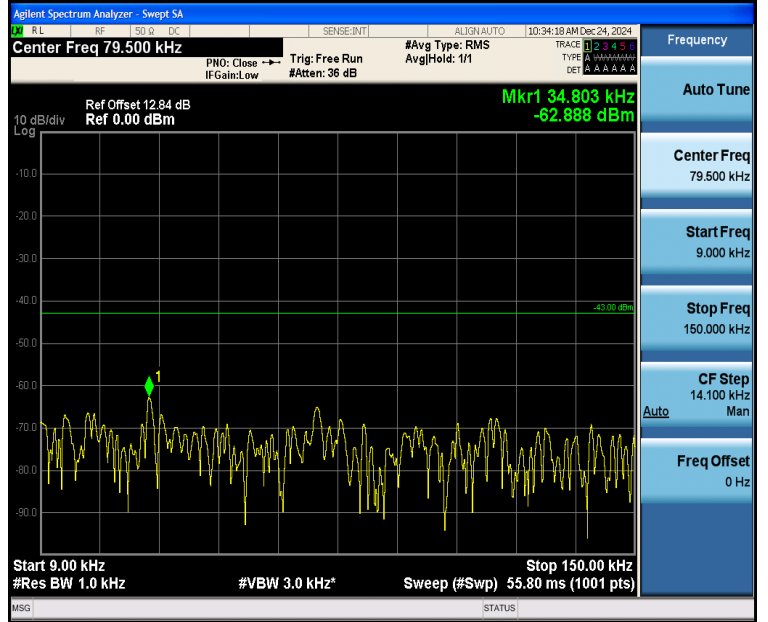
Band2_10MHz_QPSK_18900_50RB#0_0.009~0.15_0.009~0.15
