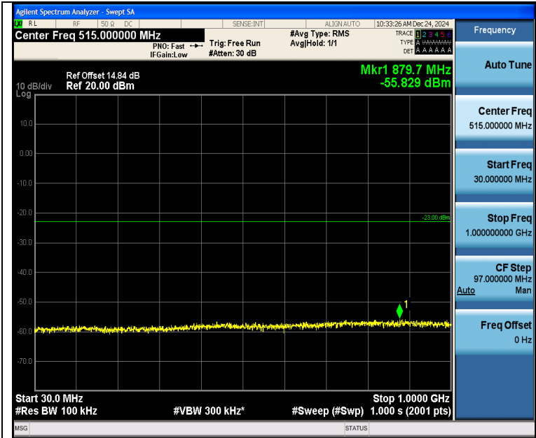
Band2_10MHz_QPSK_18650_50RB#0_30~1000_30~1000
