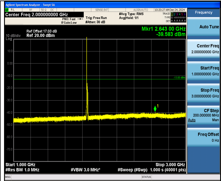
Band2_10MHz_QPSK_18650_1RB#0_1000~3000_1000~3000
