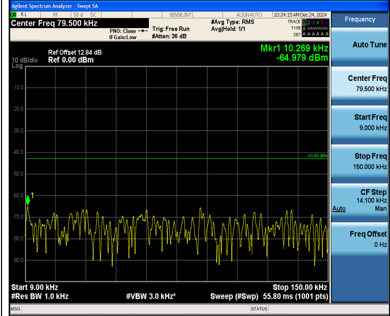
Band2_10MHz_QPSK_18900_1RB#0_0.009~0.15_0.009~0.15
