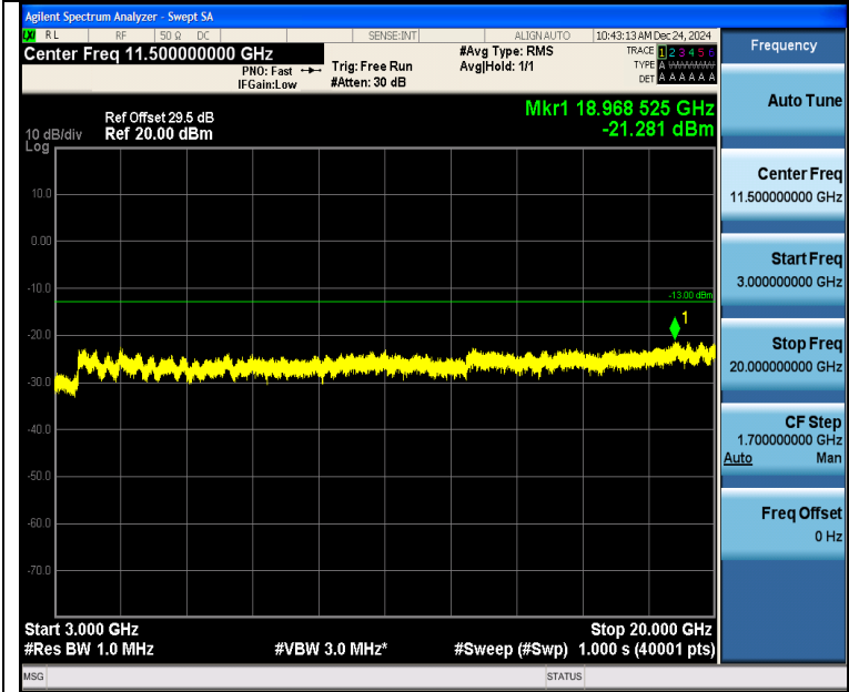
Band2_15MHz_16QAM_18675_1RB#74_3000~20000_3000~20000
