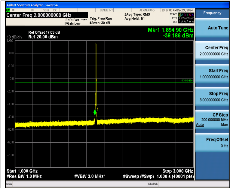
Band2_5MHz_16QAM_19175_25RB#0_1000~3000_1000~3000
