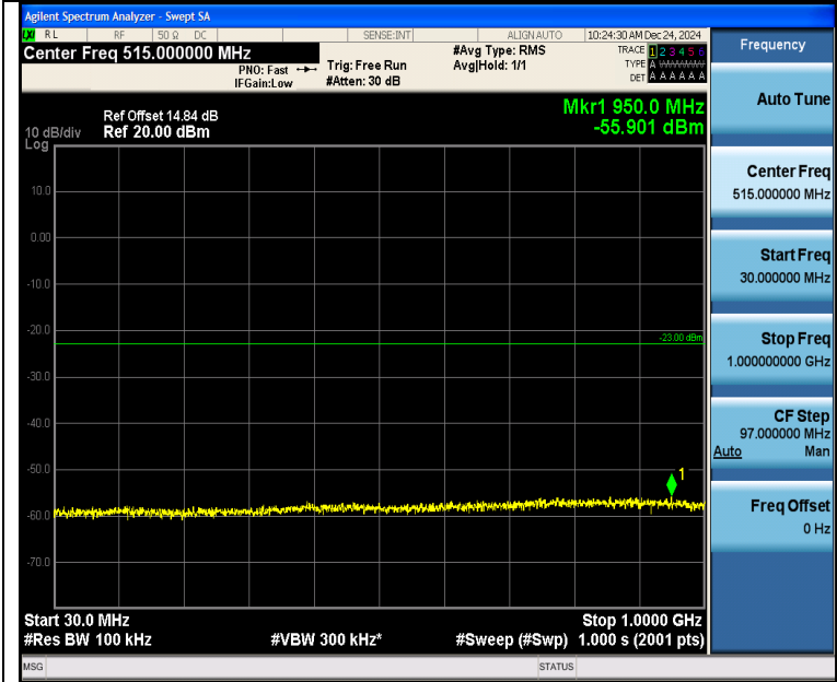
Band2_10MHz_QPSK_18900_1RB#0_30~1000_30~1000
