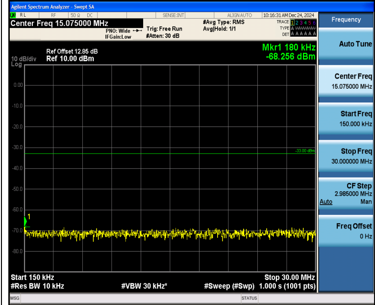
Band2_5MHz_16QAM_19175_25RB#0_0.15~30_0.15~30
