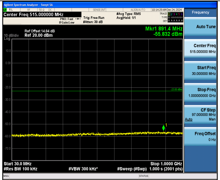
Band2_5MHz_16QAM_19175_1RB#24_30~1000_30~1000
