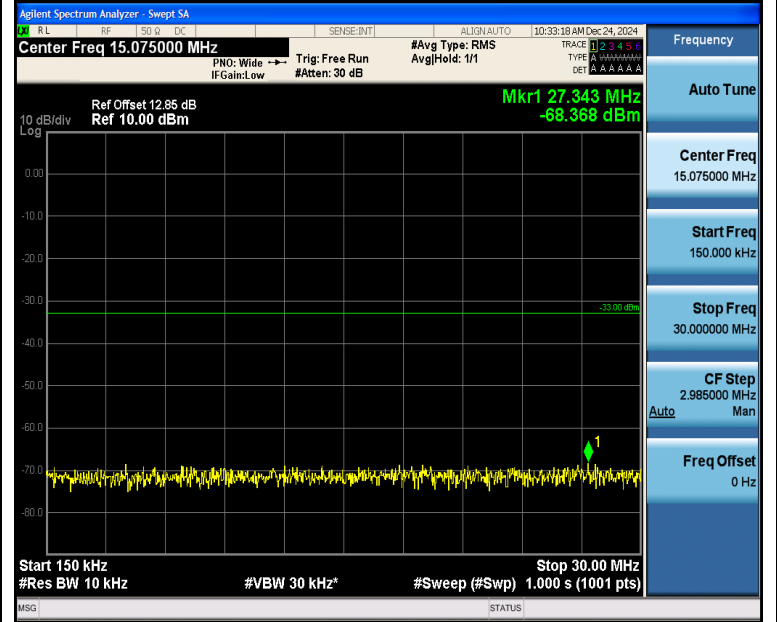
Band2_10MHz_QPSK_18650_50RB#0_0.15~30_0.15~30
