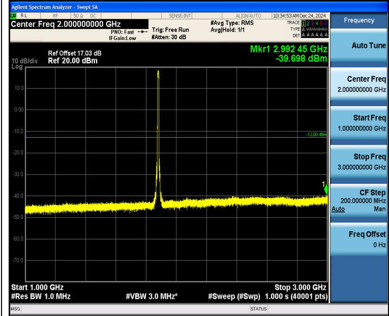
Band2_10MHz_QPSK_18900_50RB#0_1000~3000_1000~3000
