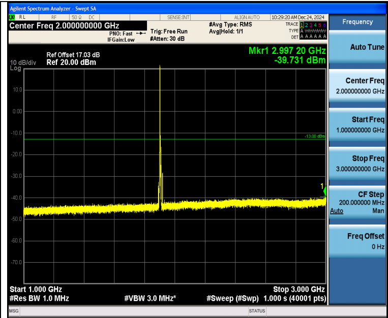
Band2_10MHz_QPSK_19150_1RB#0_1000~3000_1000~3000
