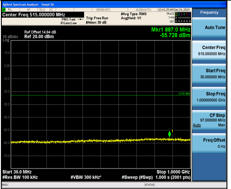
Band2_15MHz_QPSK_18675_1RB#74_30~1000_30~1000
