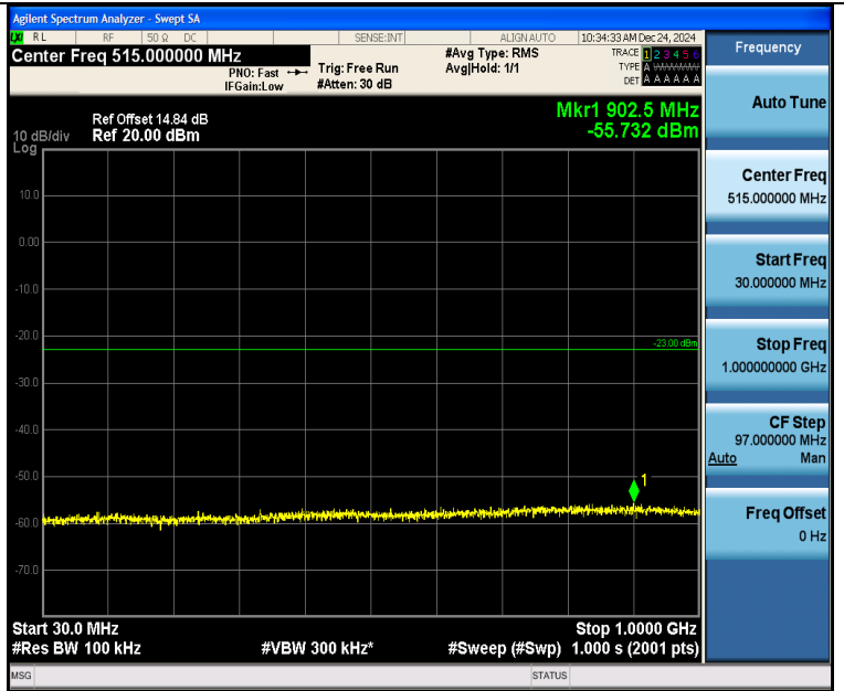
Band2_10MHz_QPSK_18900_50RB#0_30~1000_30~1000
