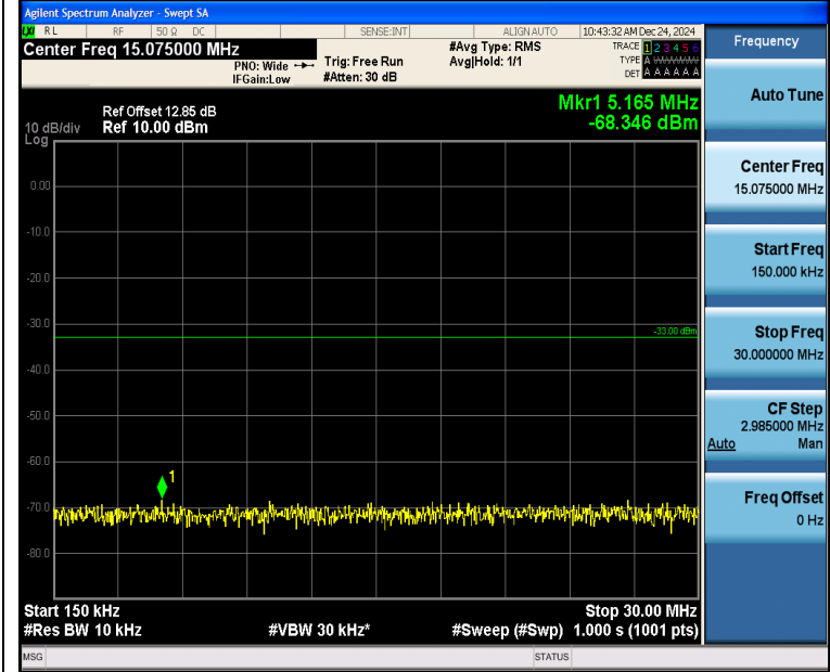
Band2_15MHz_QPSK_18900_1RB#0_0.15~30_0.15~30
