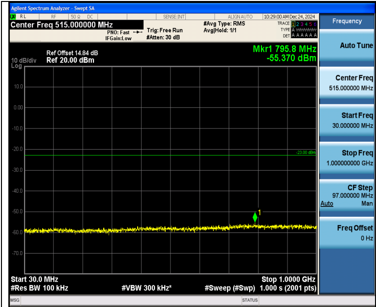
Band2_10MHz_QPSK_19150_1RB#0_30~1000_30~1000
