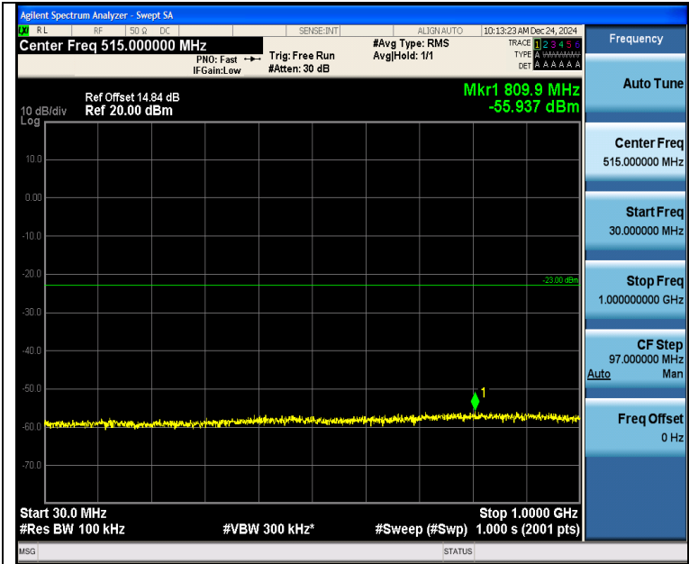
Band2_5MHz_QPSK_19175_1RB#24_30~1000_30~1000
