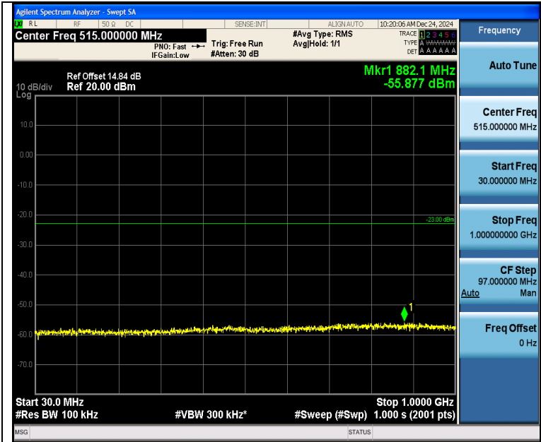
Band2_10MHz_QPSK_18650_1RB#0_30~1000_30~1000
