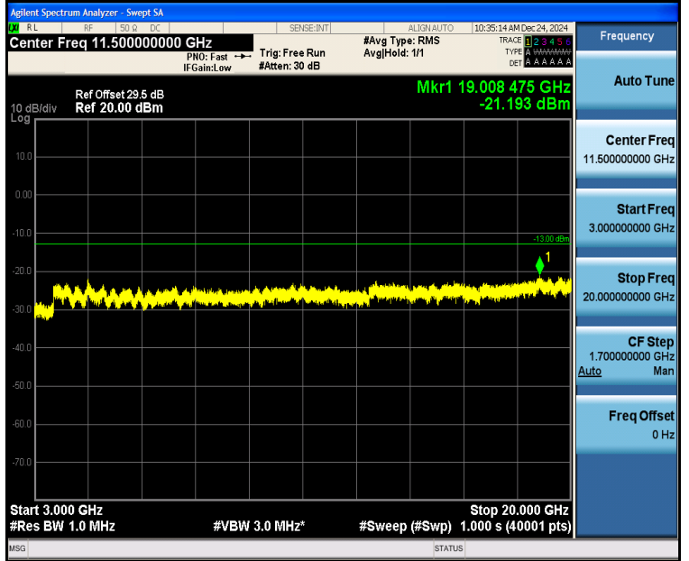
Band2_10MHz_QPSK_18900_50RB#0_3000~20000_3000~20000
