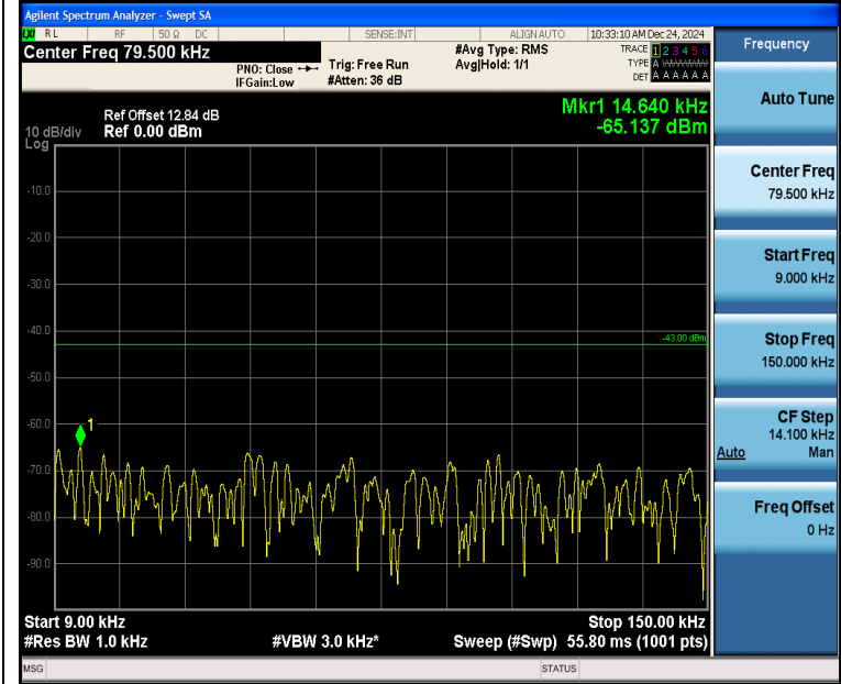
Band2_10MHz_QPSK_18650_50RB#0_0.009~0.15_0.009~0.15
