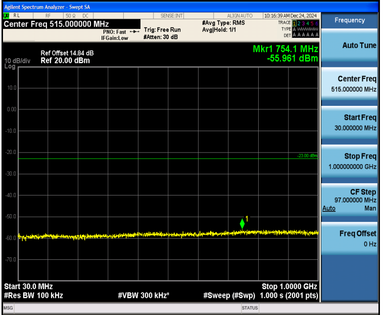
Band2_5MHz_16QAM_19175_25RB#0_30~1000_30~1000
