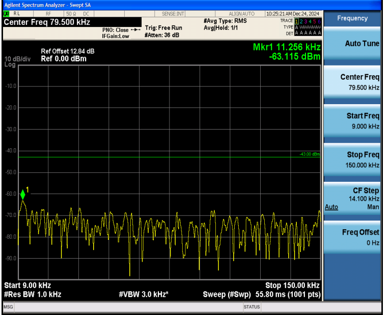
Band2_10MHz_16QAM_18900_1RB#0_0.009~0.15_0.009~0.15
