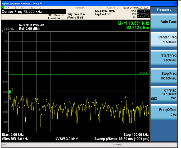
Band2_5MHz_16QAM_19175_25RB#0_0.009~0.15_0.009~0.15
