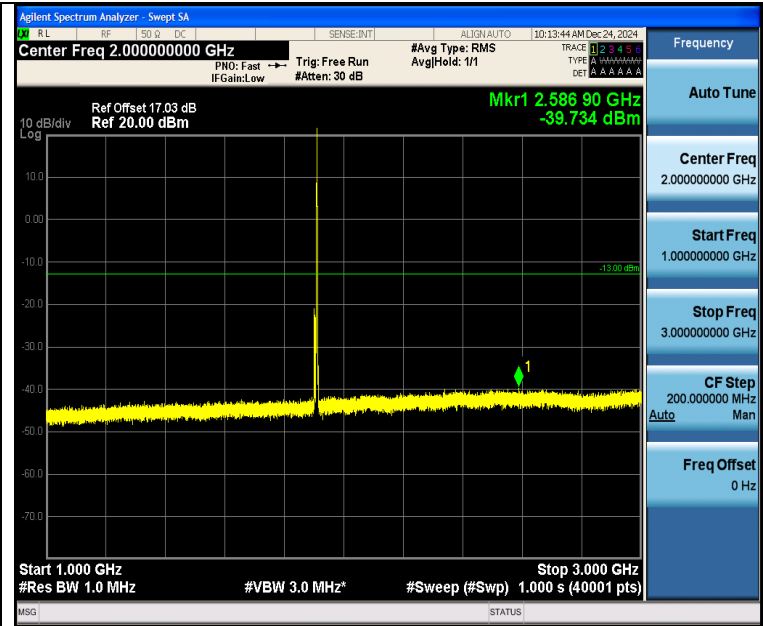
Band2_5MHz_QPSK_19175_1RB#24_1000~3000_1000~3000
