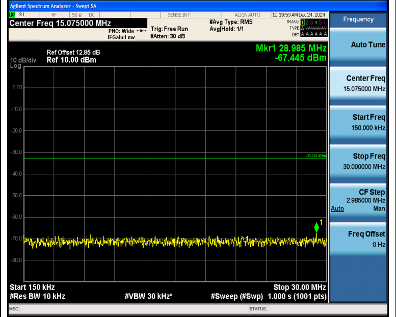
Band2_10MHz_QPSK_18650_1RB#0_0.15~30_0.15~30
