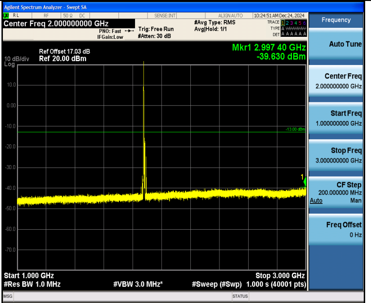
Band2_10MHz_QPSK_18900_1RB#0_1000~3000_1000~3000
