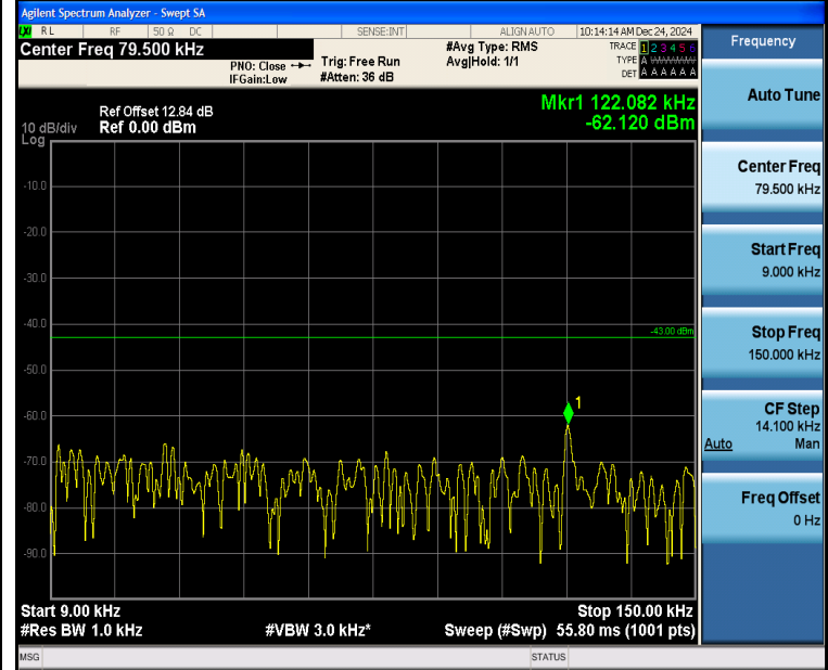
Band2_5MHz_16QAM_19175_1RB#24_0.009~0.15_0.009~0.15
