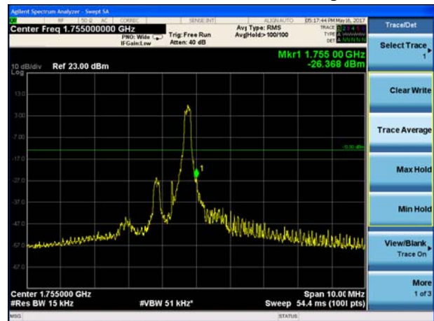
LTE Band 4 QPSK 1.4MHz CH-High, 5 RB
