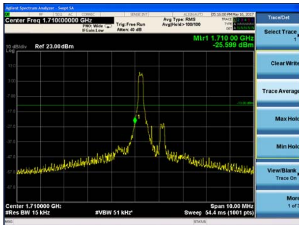
LTE Band 4 QPSK 1.4MHz CH-Low, 5 RB
