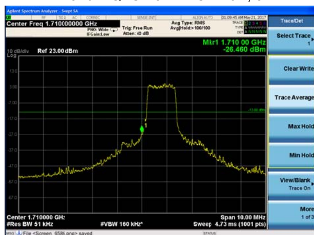
LTE Band 4 QPSK 5MHz CH-Low, 5 RB
