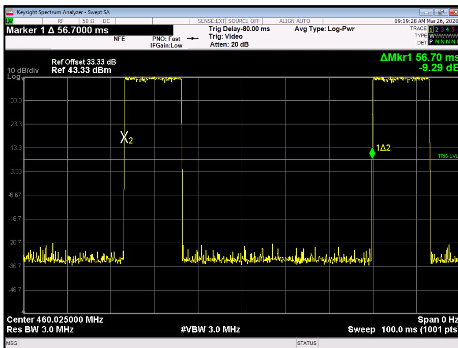
Figure 6 - Burst Period
