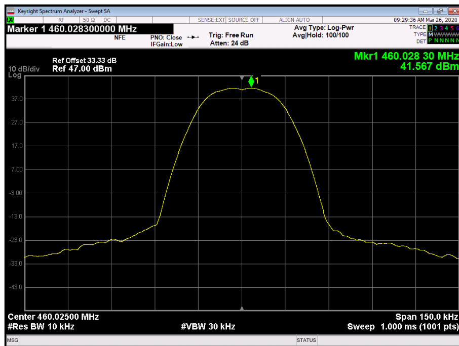
Figure 7 - Frequency Spectrum
