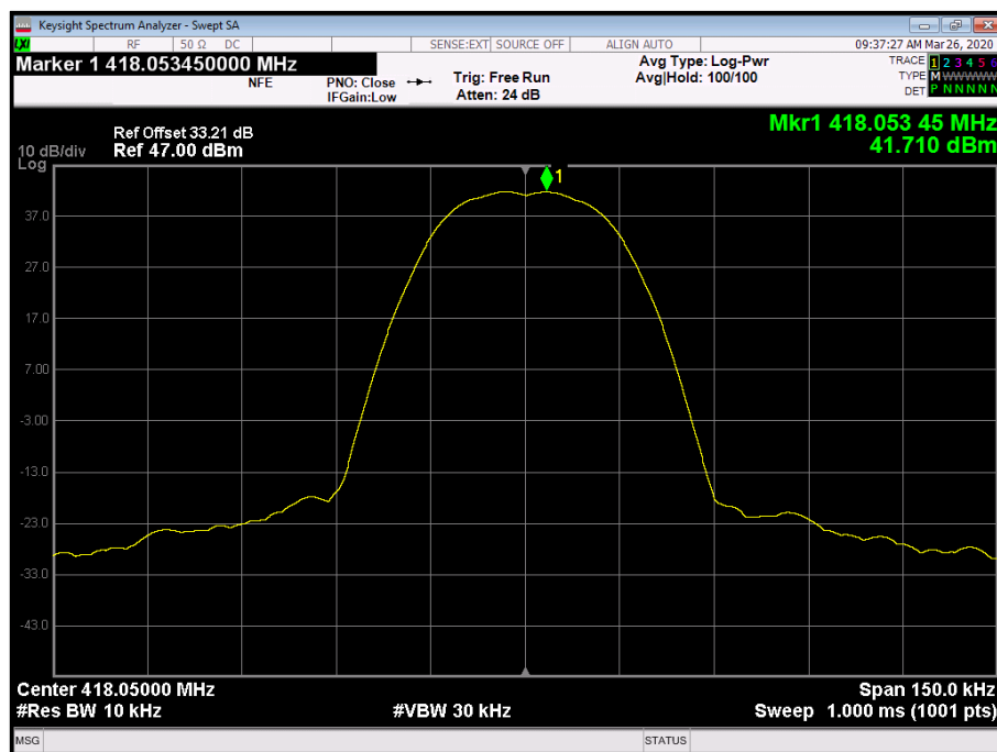
Figure 4 - Frequency Spectrum
