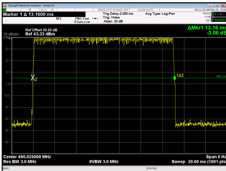
Figure 5 - Burst Length
