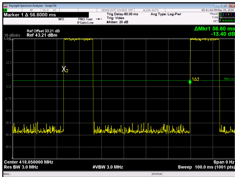
Figure 3 - Burst Period
