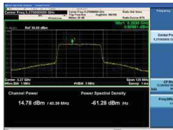
Antenna D
