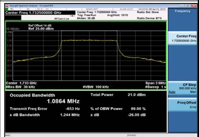
FDD04_MidRange_3_1732.5_Q16
