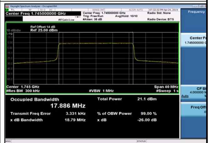
FDD66_MidRange_20_1745_Q16
