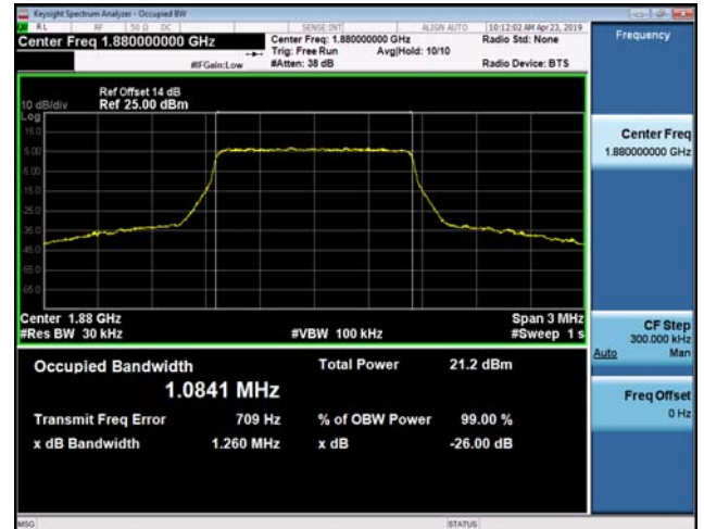
FDD02_MidRange_3_1880_Q16
