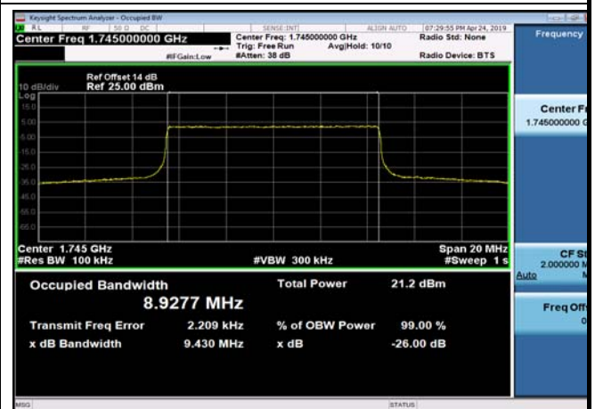
FDD66_MidRange_10_1745_Q16
