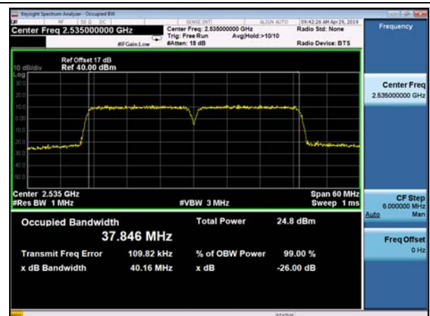
FDD7_MidRange_20+20_Q16
