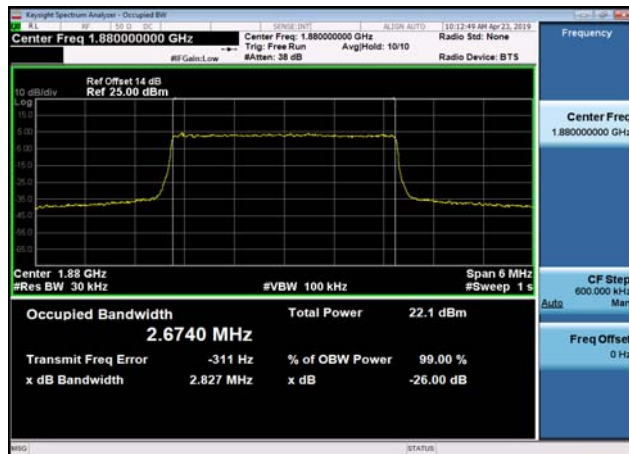
FDD02_MidRange_5_1880_QPSK
