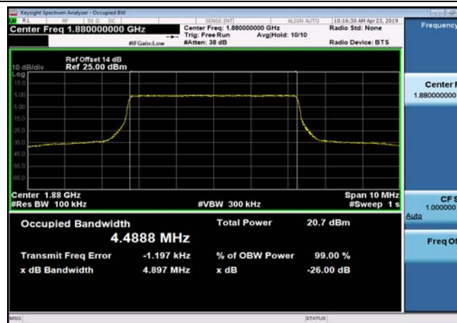
FDD02_MidRange_5_1880_Q16
