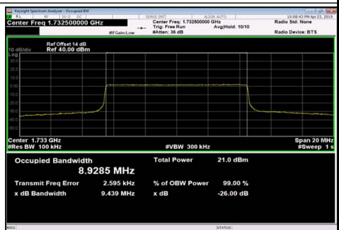
FDD04_MidRange_10MHz_1732.5MHz_Q16
