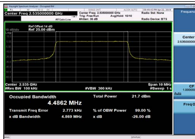
FDD07_MidRange_10MHz_2535MHz_QPSK
