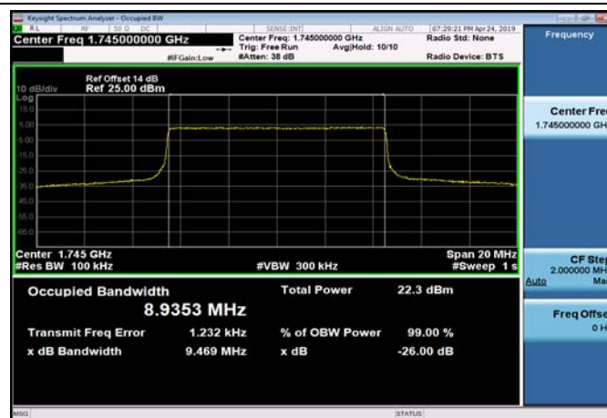
FDD66_MidRange_10_1745_QPSK
