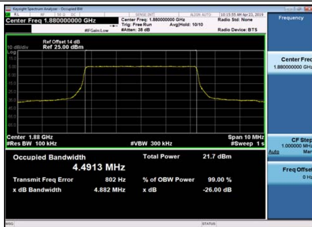
FDD02_MidRange_5_1880_QPSK
