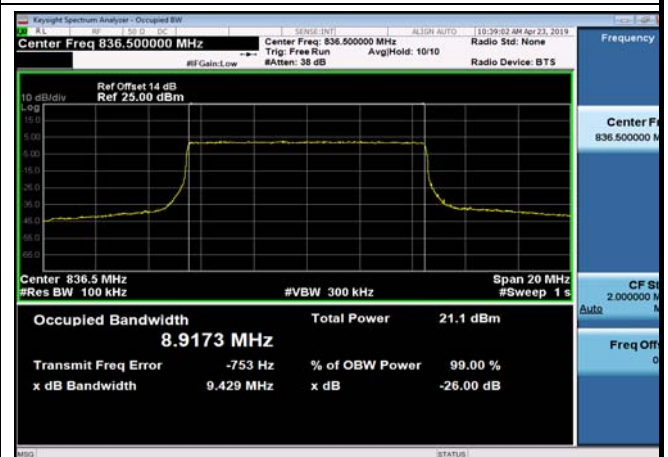
FDD05_MidRange_10_836.5_Q16
