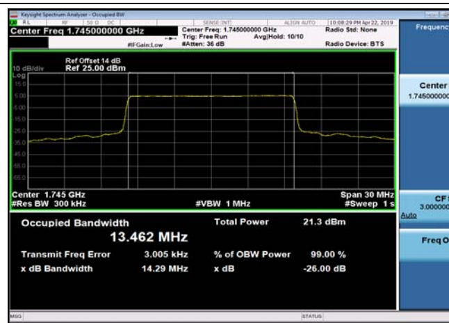
FDD66_MidRange_15MHz_1745MHz_QPSK
