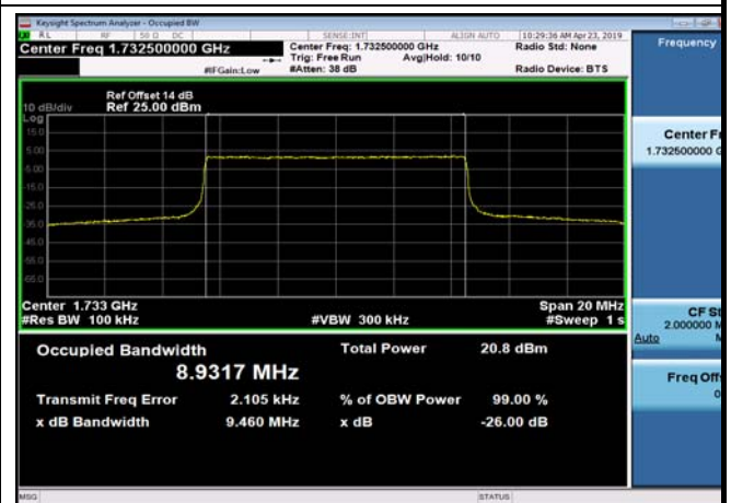
FDD04_MidRange_15_1732.5_Q16
