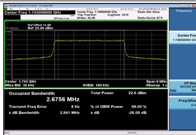
FDD66_MidRange_5_1745_QPSK
