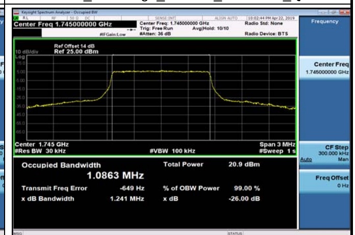
FDD66_MidRange_1.4MHz_1745MHz_Q16
