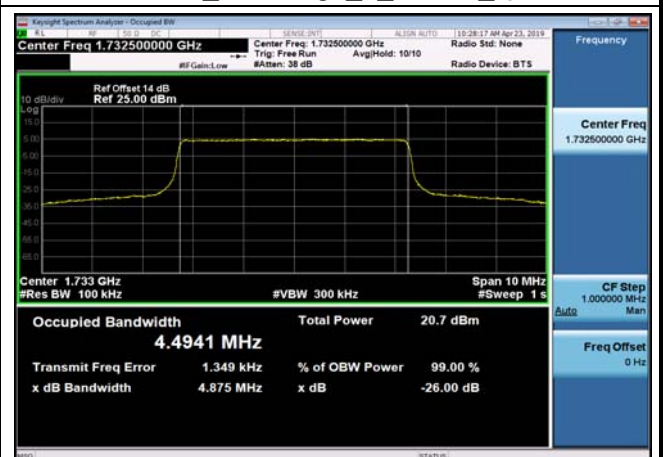
FDD04_MidRange_5_1732.5_Q16
