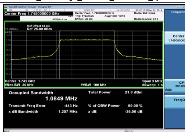
FDD66_MidRange_1.4MHz_1745MHz_QPSK
