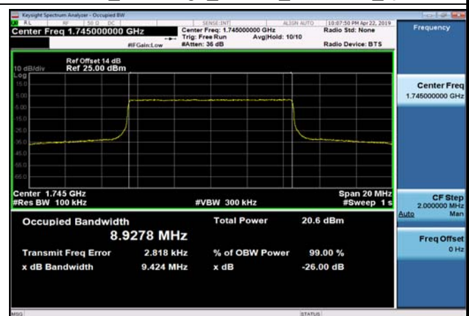
FDD66_MidRange_10MHz_1745MHz_Q16
