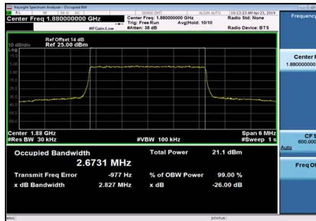
FDD02_MidRange_5_1880_Q16
