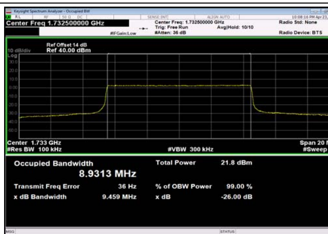
FDD04_MidRange_10MHz_1732.5MHz_QPSK
