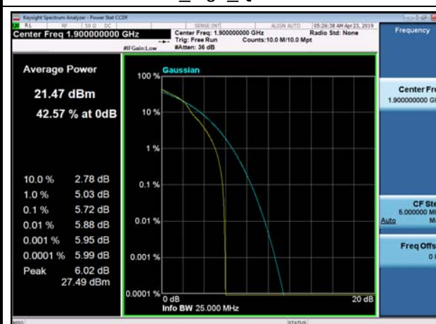
FDD02_HighRange_20MHz_1900_OneRB _high_Q16
