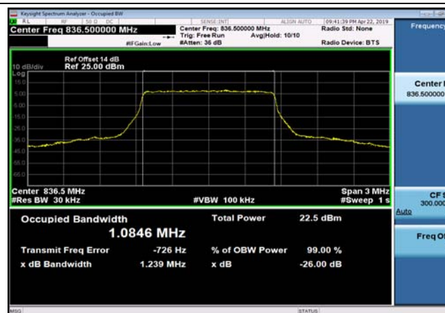
FDD05_MidRange_1.4MHz_836.5MHz _QPSK
