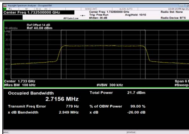
FDD04_MidRange_5MHz_1732.5MHz_QPSK
