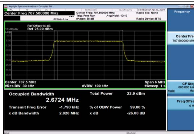
FDD12_MidRange_3_707.5_QPSK
