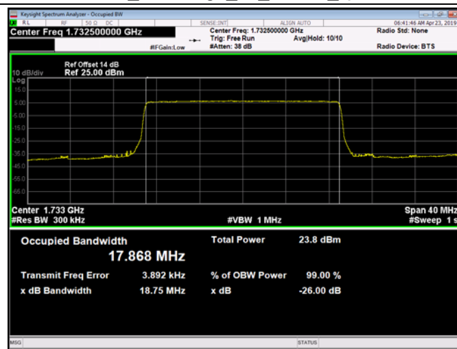
FDD04_MidRange_20_1732.5_QPSK
