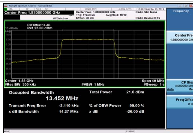
FDD02_MidRange_20_1880_QPSK
