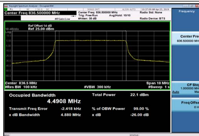
FDD05_MidRange_10_836.5_QPSK
