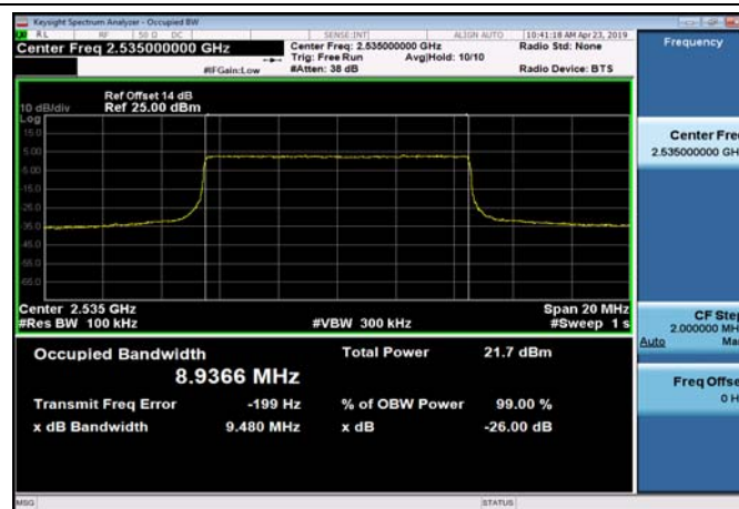
FDD07_MidRange_15_2535_QPSK
