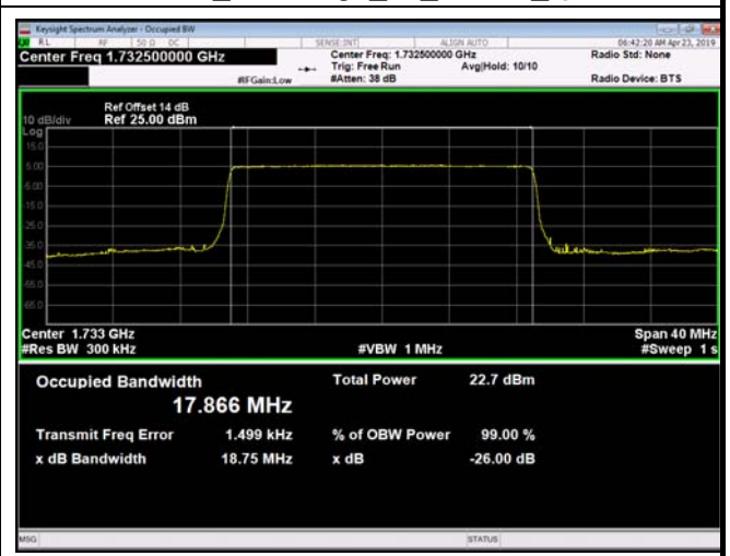
FDD04_MidRange_20_1732.5_Q16
