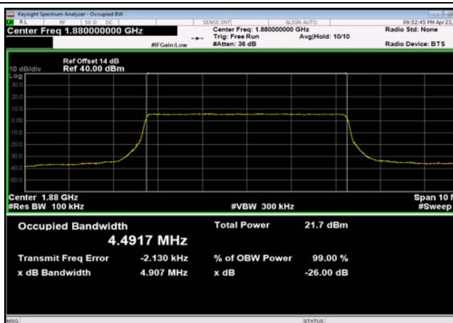
FDD02_MidRange_5MHz_1880MHz_QPSK
