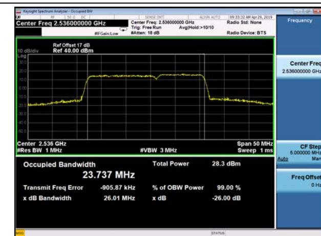
FDD7_MidRange_15+10_QPSK
