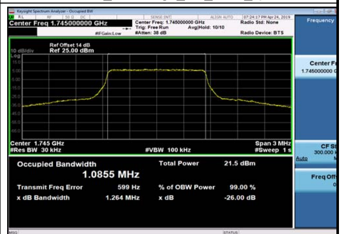
FDD66_MidRange_1.4_1745_Q16
