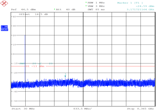
5MHz_Middle_QPSK_1@0 -24.59 dBm
