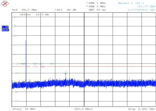
5MHz_High_QPSK_25@0 -21.77 dBm
