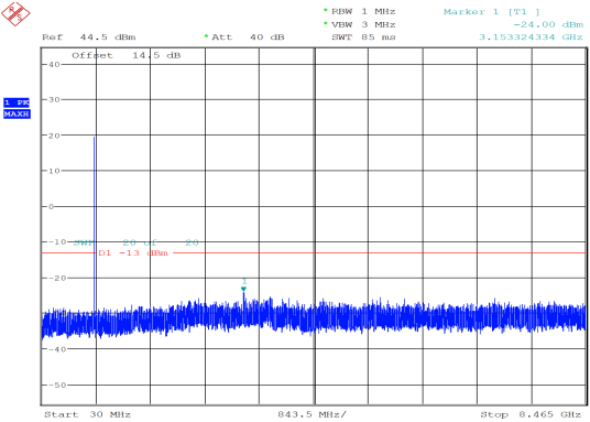
5MHz_High_QPSK_1@0 -24.00 dBm
