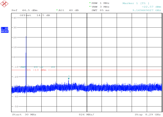
10MHz_Low_QPSK_1@0 -22.57 dBm
