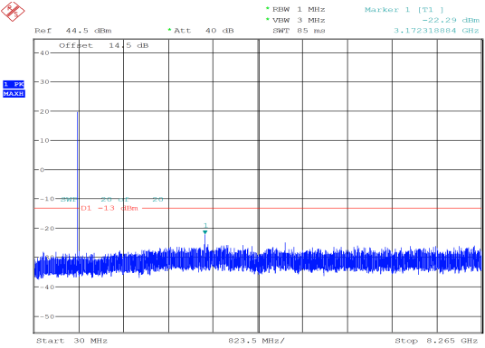
5MHz_Low_QPSK_1@0 -22.29 dBm
