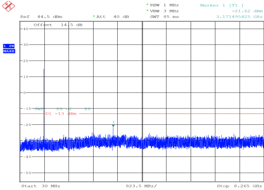
5MHz_Low_QPSK_25@0 -21.62 dBm
