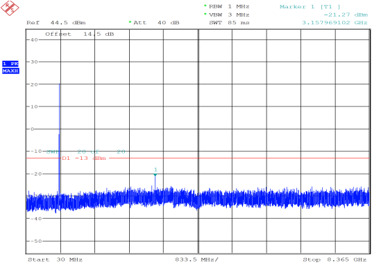
10MHz_Middle_QPSK_1@0 -21.27 dBm
