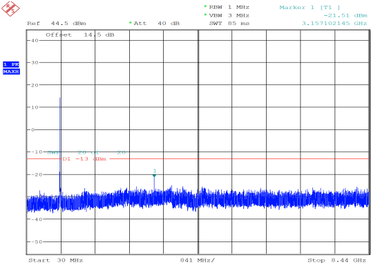
10MHz_High_QPSK_50@0 -21.51 dBm
