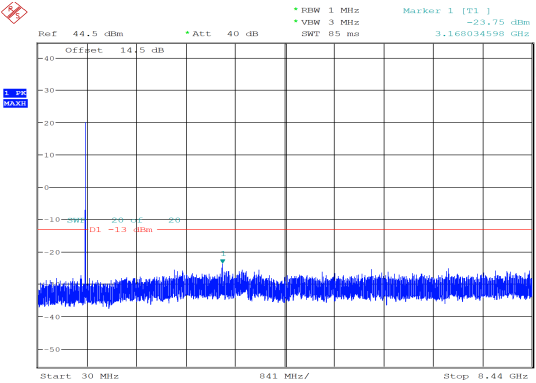
10MHz_High_QPSK_1@0 -23.75 dBm
