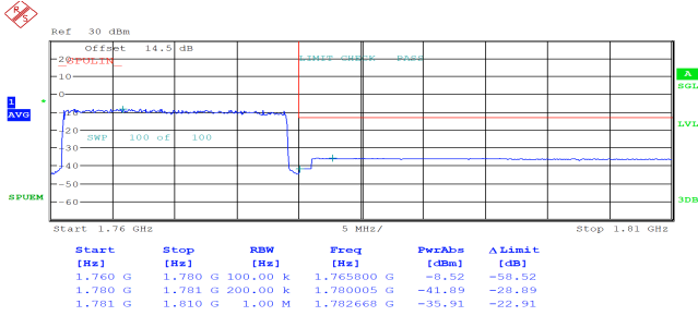
20MHz_High_QPSK_100@0
