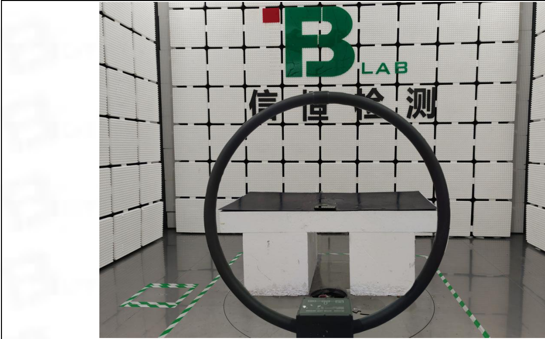
Emissions in restricted frequency bands (0.15-30 MHz)
