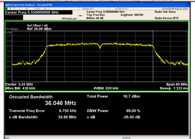
IEEE 802.11n Channel 110 40MHz Antenna 3
